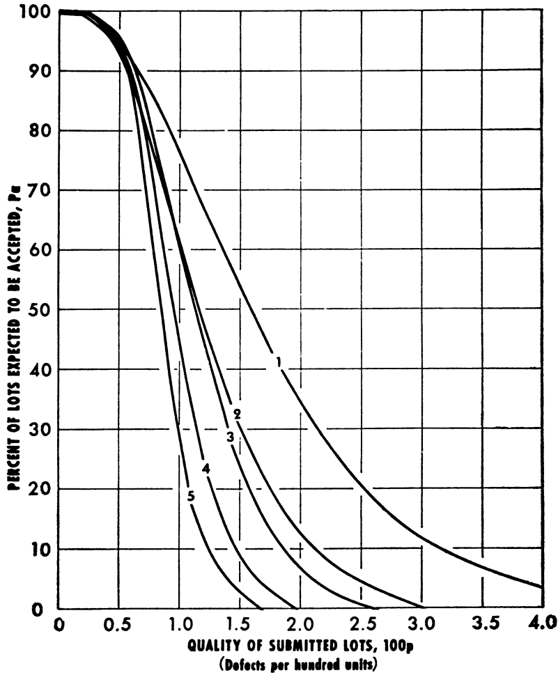
OC CURVES - AQL = 1.00
