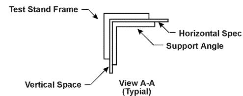
Horizontal and Vertical Specimens are Clamped in Place on all Edges between Angles as Shown in View A-A
