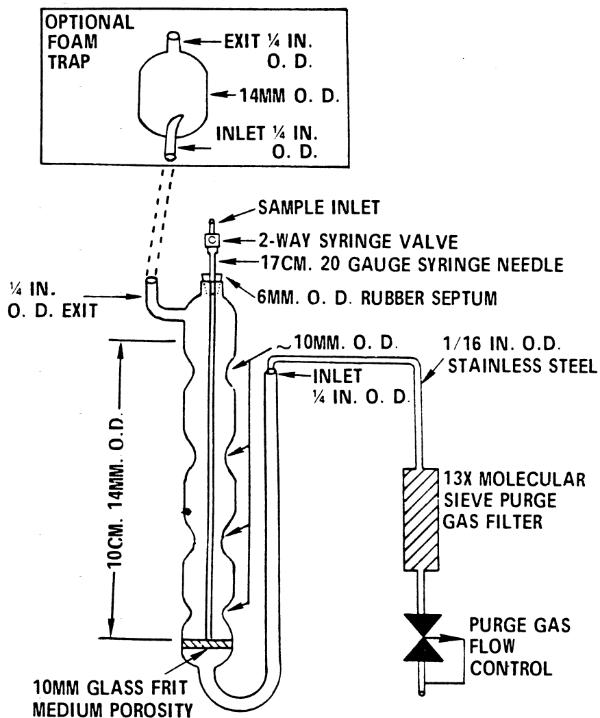
Figure 1. Purging device.
