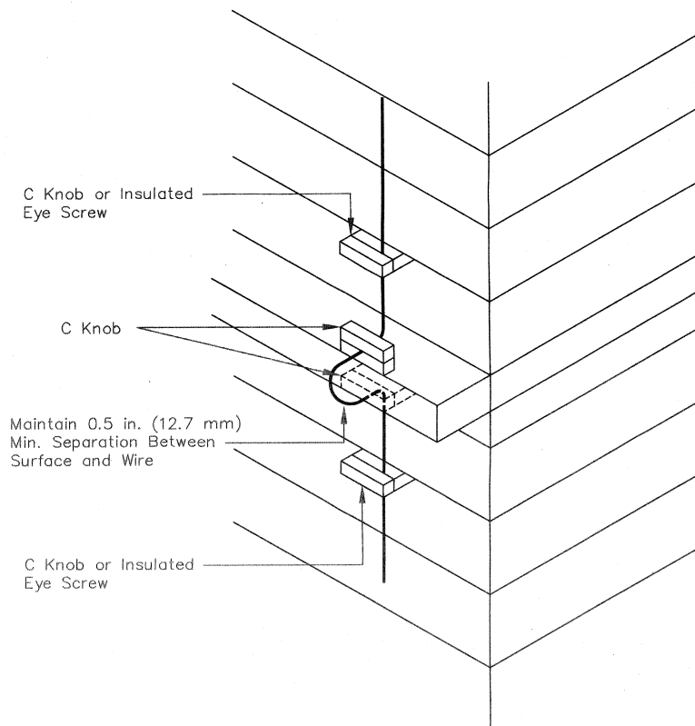
FIGURE 6 AERIAL SERVICE WIRE CROSSING COMBUSTIBLE BUILDING PROJECTIONS
