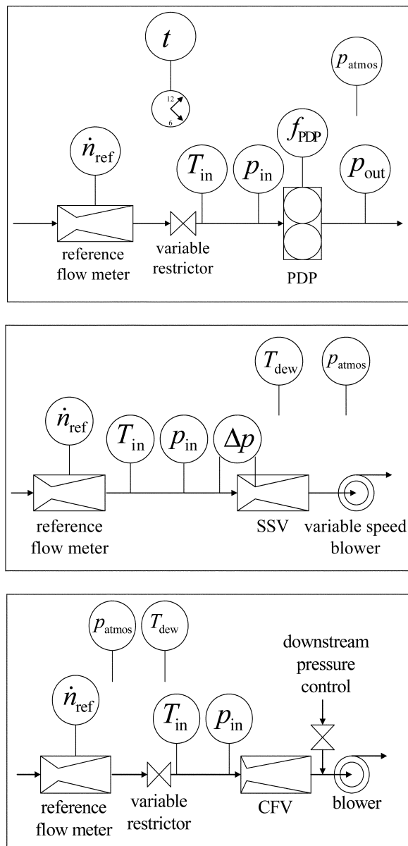
Figure 1 of § 1066.140—CVS calibration configurations
