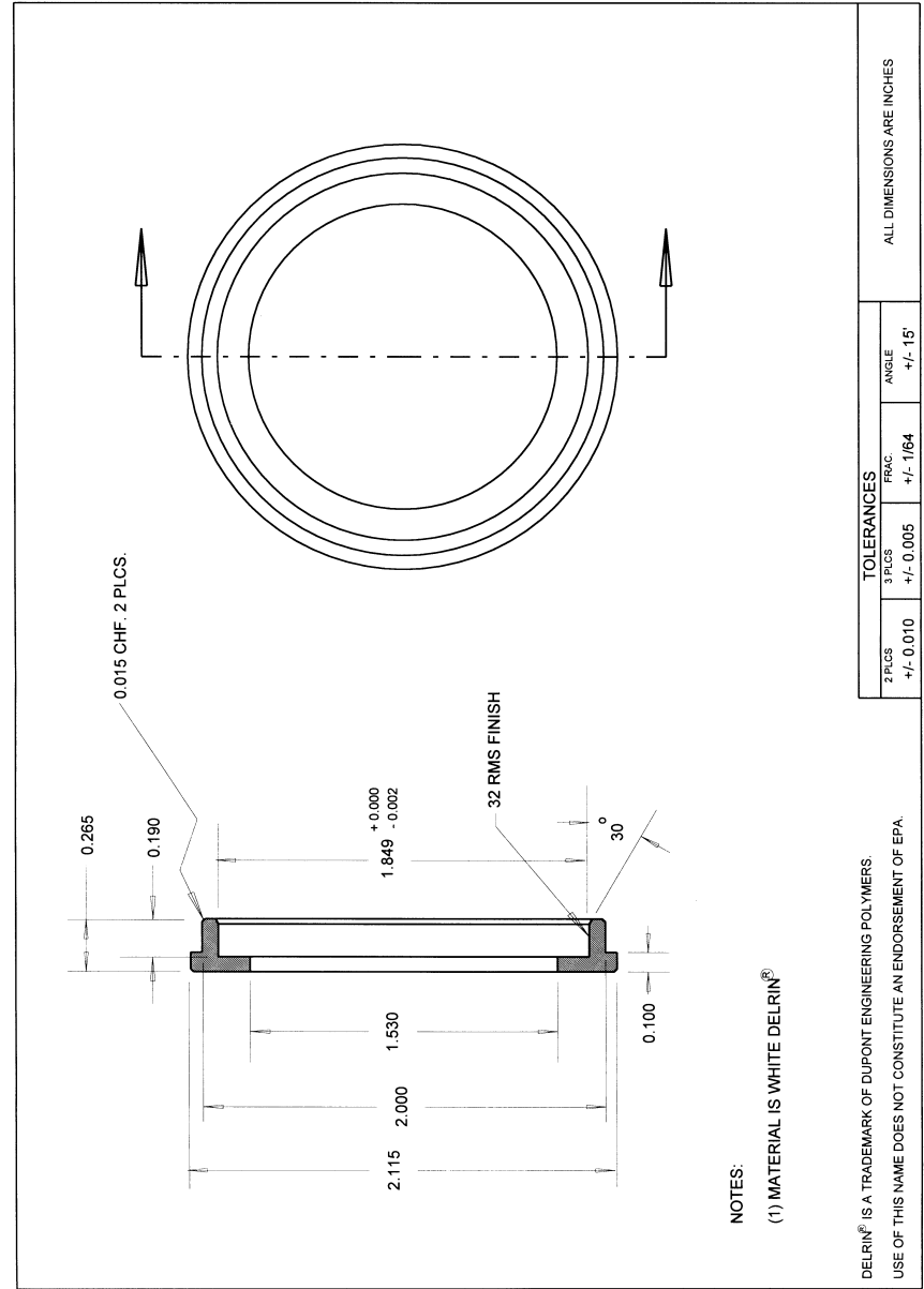
FIGURE L-29. FILTER CASSETTE, LOWER SECTION
