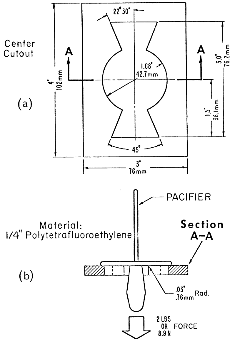
FIG I—PACIFIER TEST FIXTURE
