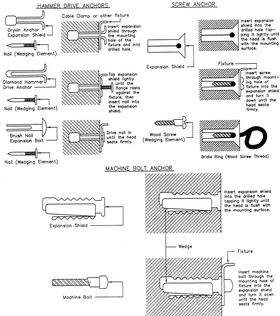
FIGURE 1 ANCHORING DEVICES
