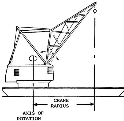
Figure 173.010 Crane Radius
