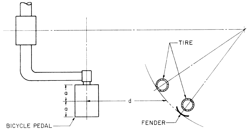
FIG 6 -TOE CLEARANCE
