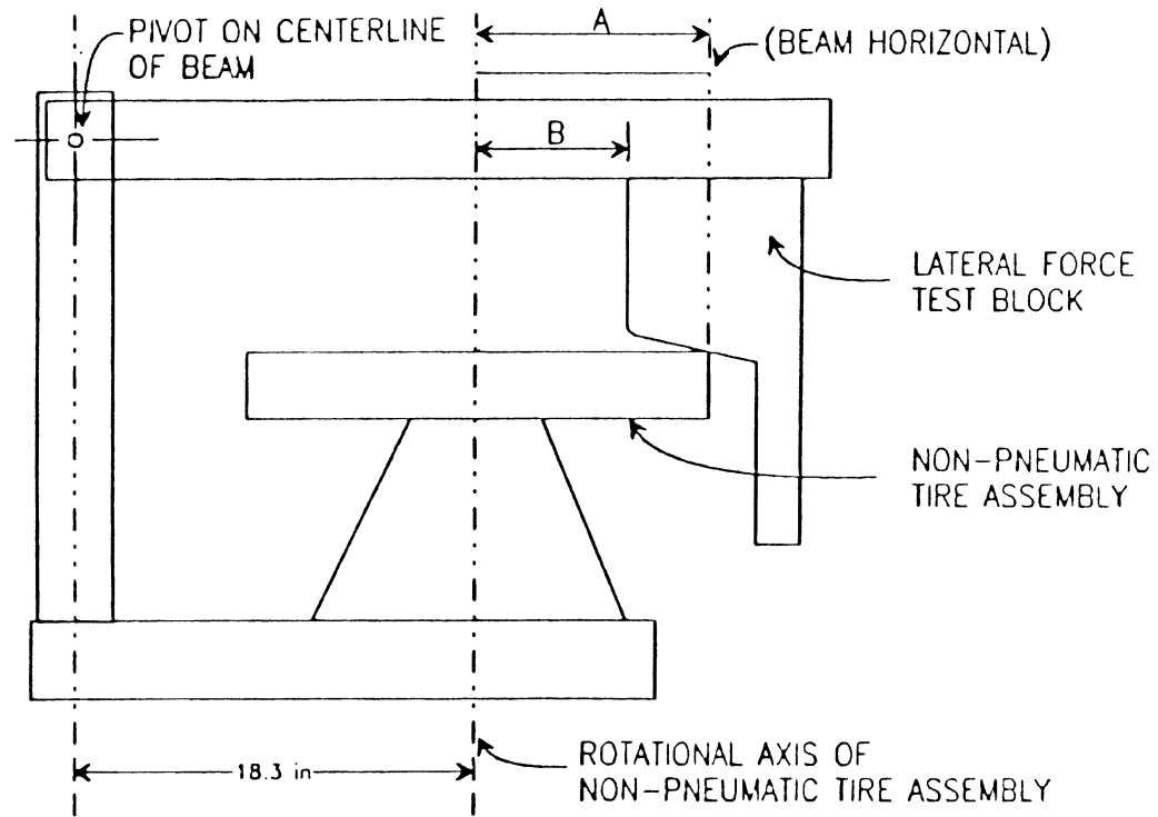
FIGURE 1 - LATERAL FORCE TEST FIXTURE (DIMENSIONS IN INCHES)
