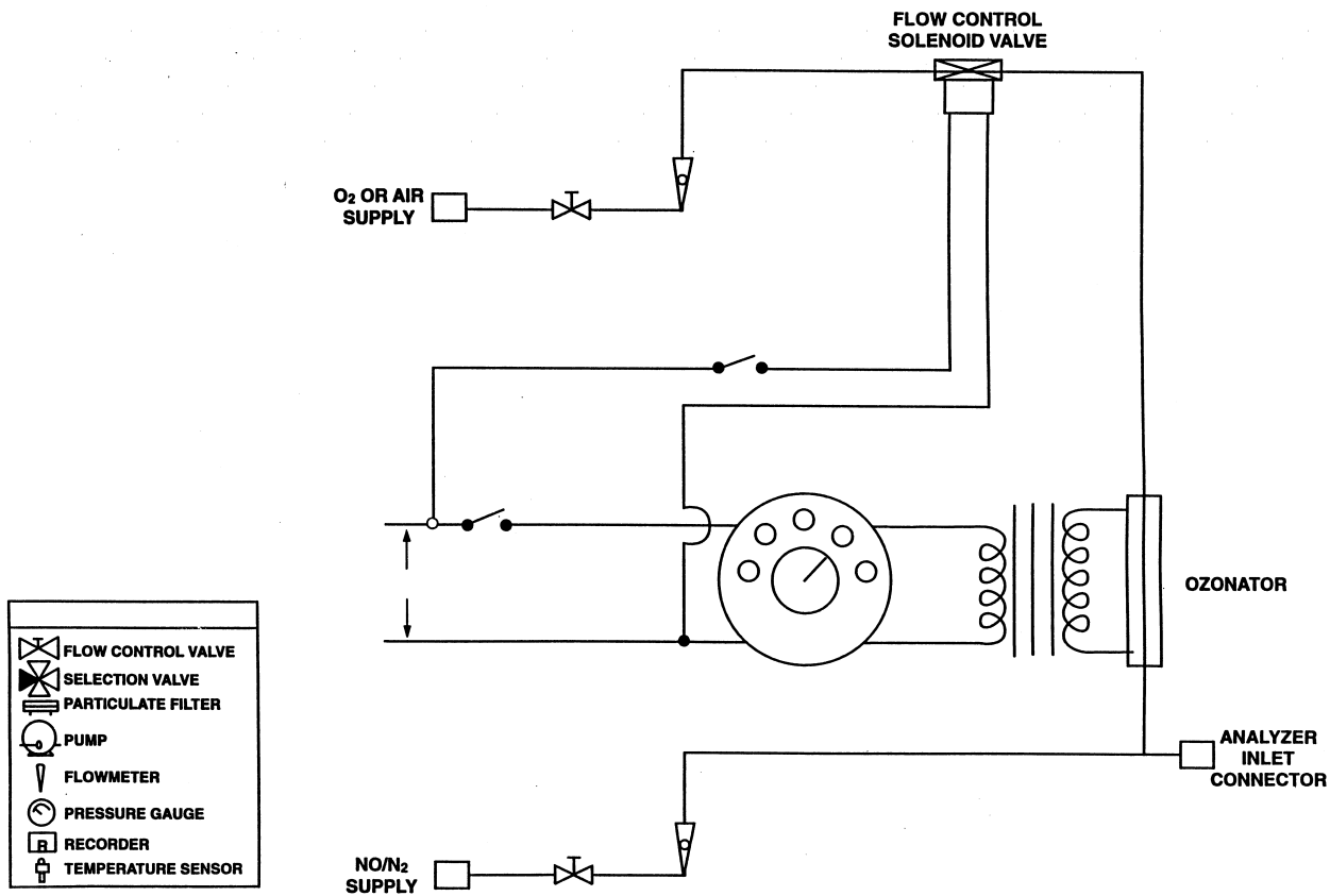
Figure 2. — NO x Converter Efficiency Detector
