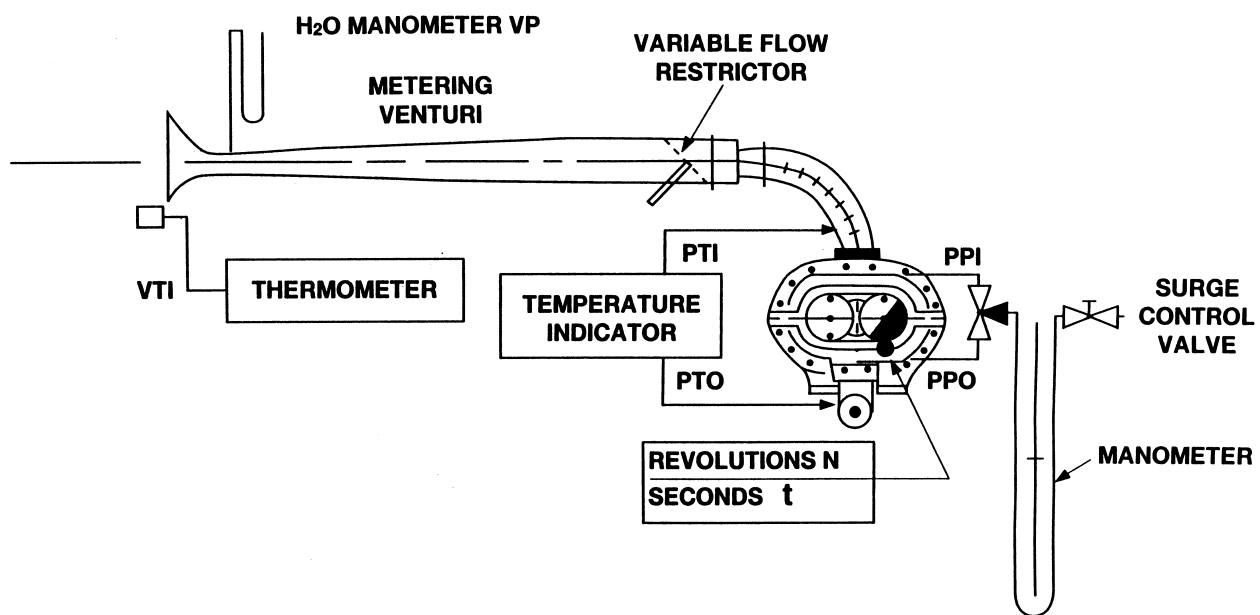
Figure 5. — PDP-CVS Calibration Configuration
