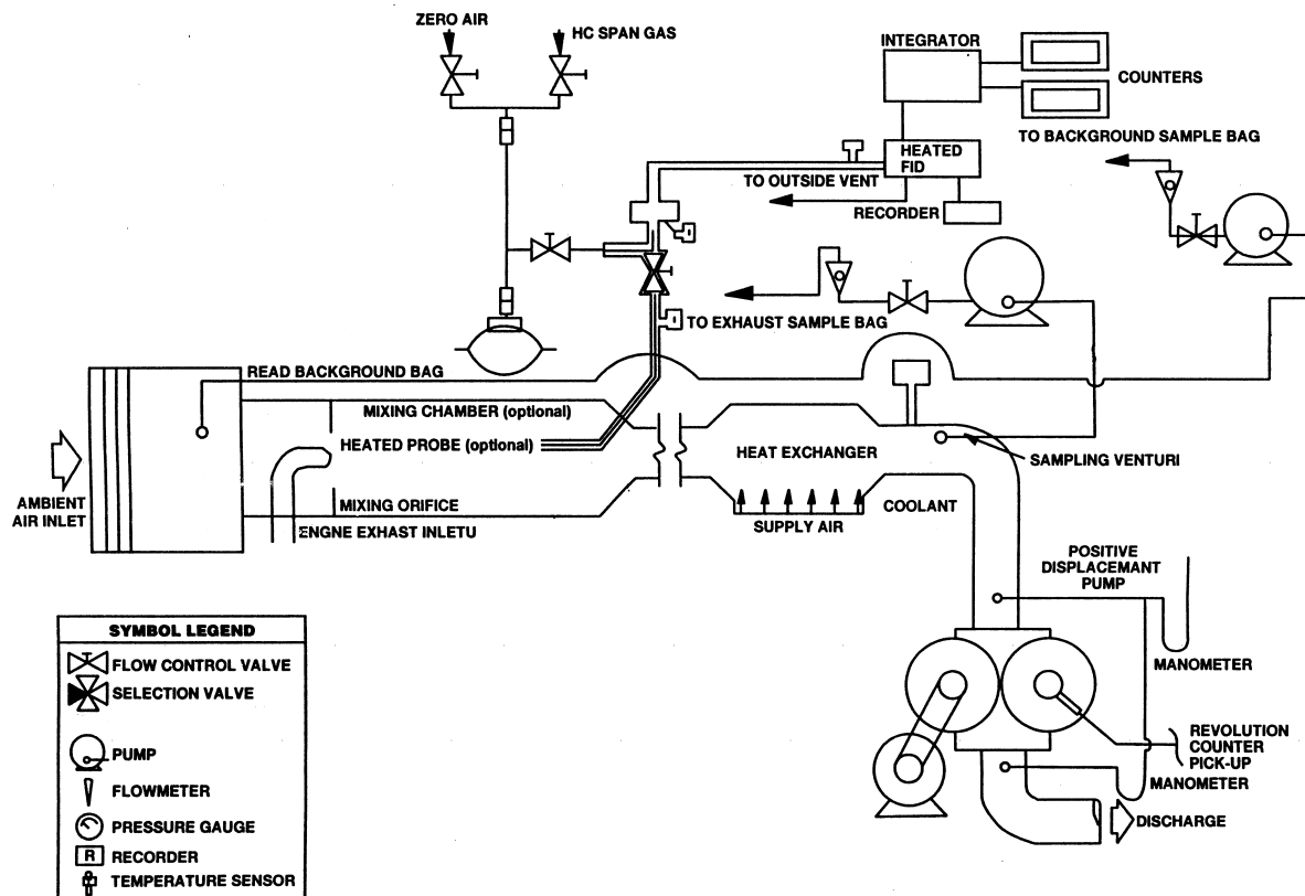
Figure 2 — Gaseous Emissions Sampling System (PDP-CVS) Showing both grab bag sampling and continous sampling
