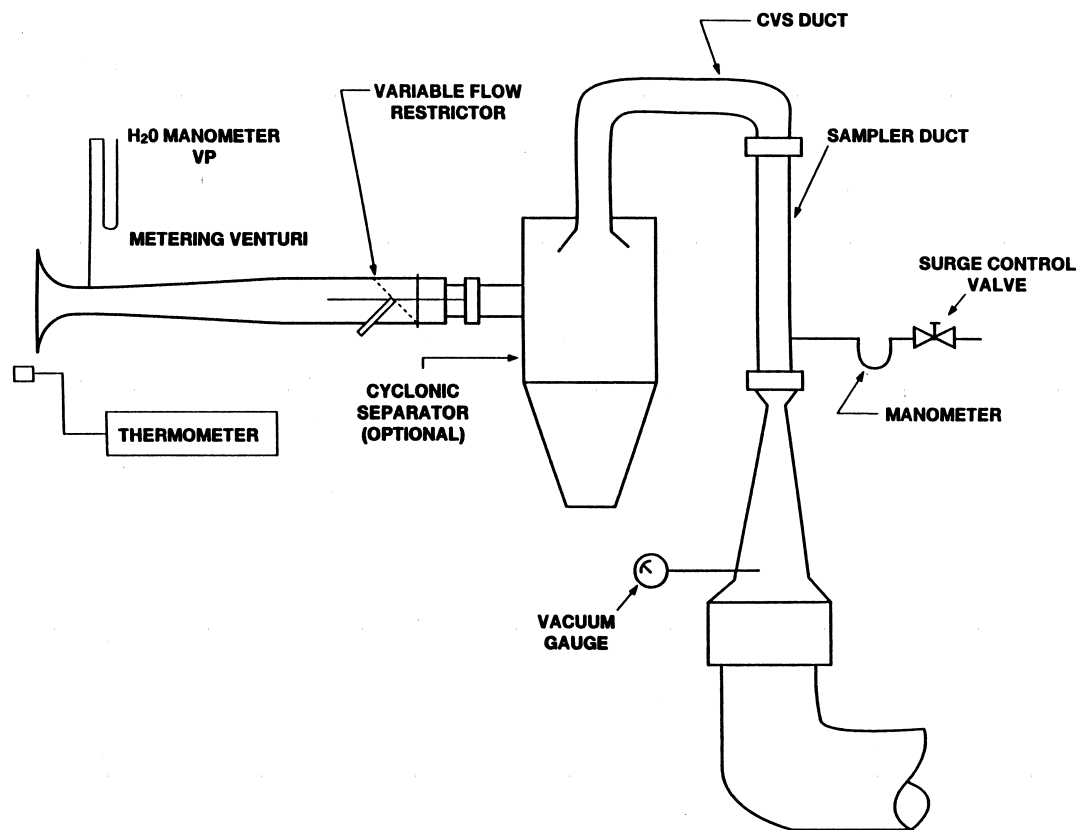
Figure 6. — CFV-CVS Calibration Configuration
