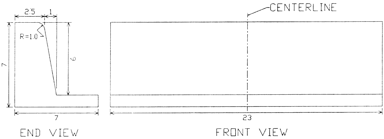
FIGURE 2 - LATERAL FORCE TEST BLOCK
