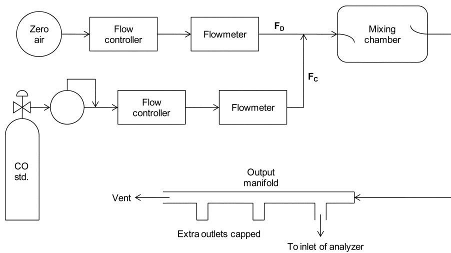
Figure 1. Dilution method for calibration of CO analyzers.
