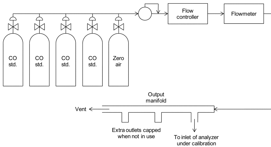
Figure 1. Dilution method for calibration of CO analyzers.
