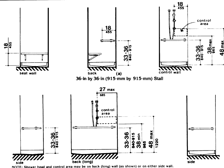
(b) 30-in by 60-in (760-mm by 1525-mm) Stall Fig. 37 Grab Bars at Shower Stalls
