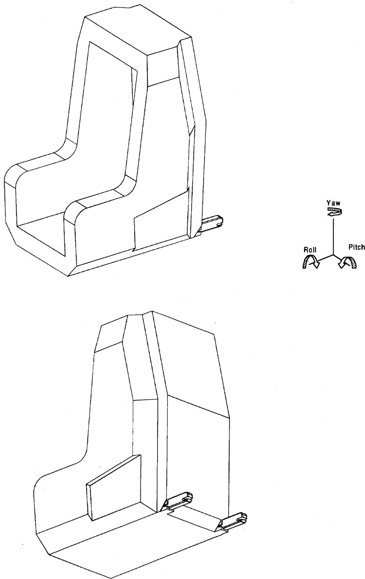
Figure 1 – Child restraint fixture (CRF)
