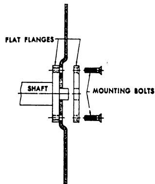
FIGURE NO. O-24 The Type 27 A Wheel is mounted between flat non-relieved flanges of equal bearing surfaces.
