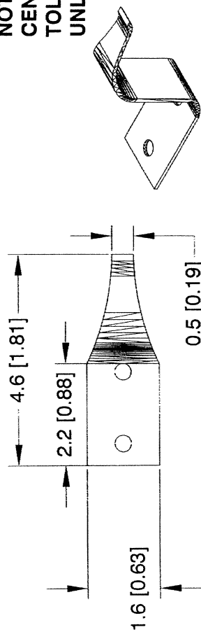
FIGURE 5 TO PART 1610—AN EXAMPLE OF A TYPICAL GAS SHIELD
