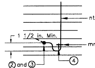
SKETCH B: Aerial Service Wire - Aerial Service Entrance
