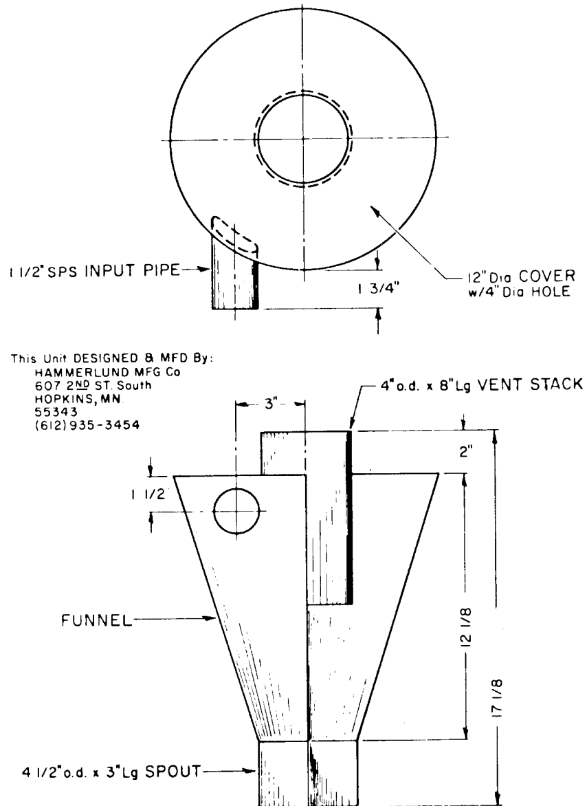
FIG 2—CYCLONE RECEIVER WELDMENT
