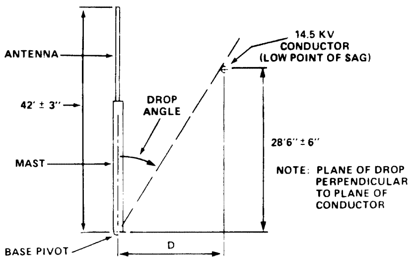
ANTENNA SYSTEM TEST SETUP
