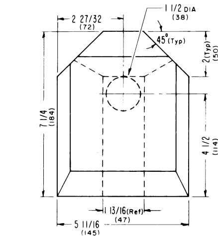
FIGURE 2 TO PART 1509—HEADFORM PROBE
