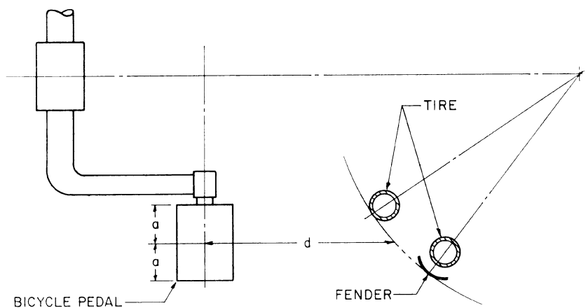
FIG 6 -TOE CLEARANCE
