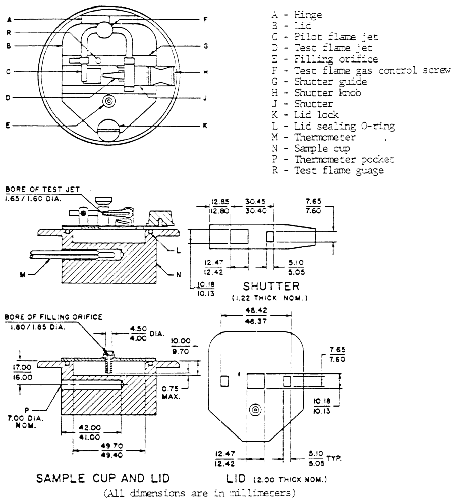
FIGURE 1 - Closed-cup tester
