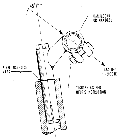
FIG 2—HANDLEBAR STEM LOADING
