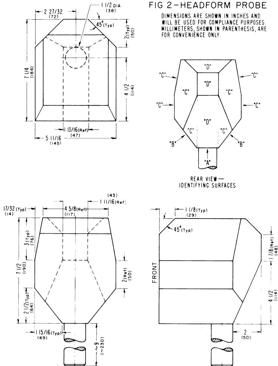
FIGURE 2 TO PART 1509—HEADFORM PROBE
