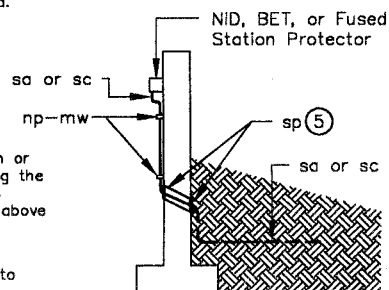
SKETCH C: Buried Service - Below Grade Entrance
