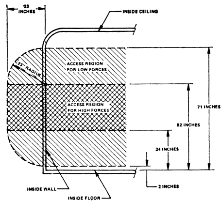
3A. SIDE EMERGENCY EXIT
