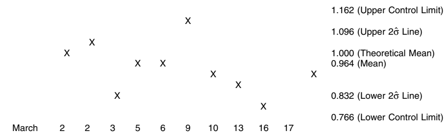
FIGURE 1—THEORETICAL EXAMPLE OF A CONTROL CHART FOR A POOL OF AN ANALYTE
