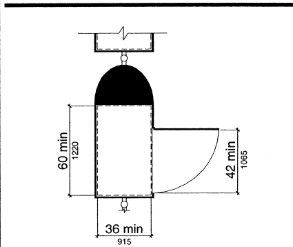
Fig. A9 Wheelchair Spaces - Side Entry
