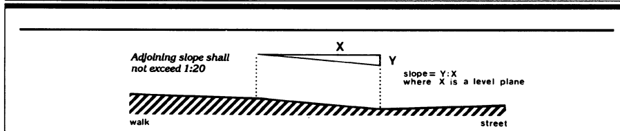
Fig. 11 Measurement of Curb Ramp Slopes
