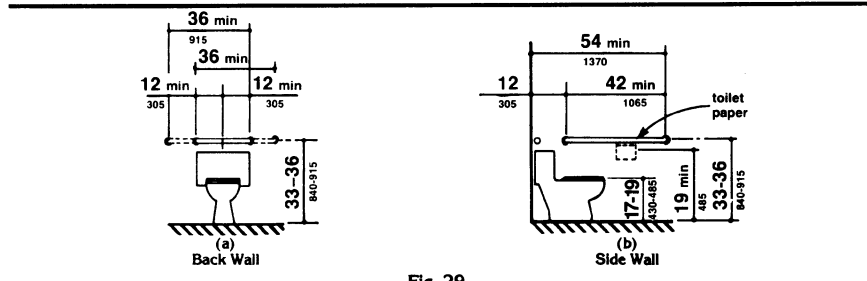
Fig. 29 Grab Bars at Water Closets
