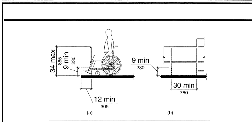
Fig. 62 Edge Protection at Fishing Piers
