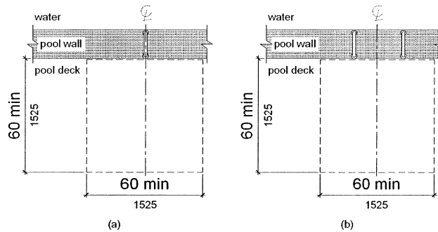
Fig. 74 Clear Deck Space at Transfer Walls
