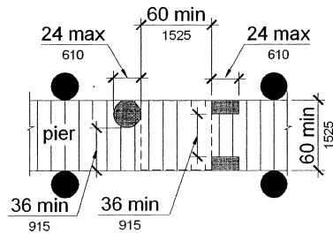
Fig. 60 Pier Clear Space Reduction
