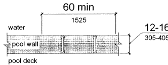
Fig. 76 Transfer Wall Depth and Length
