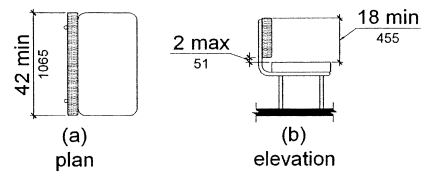
Fig. 48 Bench Back Support
