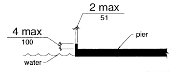
Fig. 61 Edge Protection at Pier
