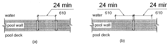
Fig. 76 Transfer Wall Depth and Length
