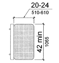
Fig. 47 Size of Bench
