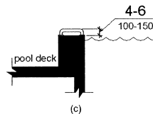
Fig. 77 Grab Bars at Transfer Walls
