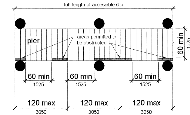
Fig. 59 Pier Clearances
