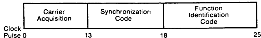
Figure 6 - Preamble organization.
