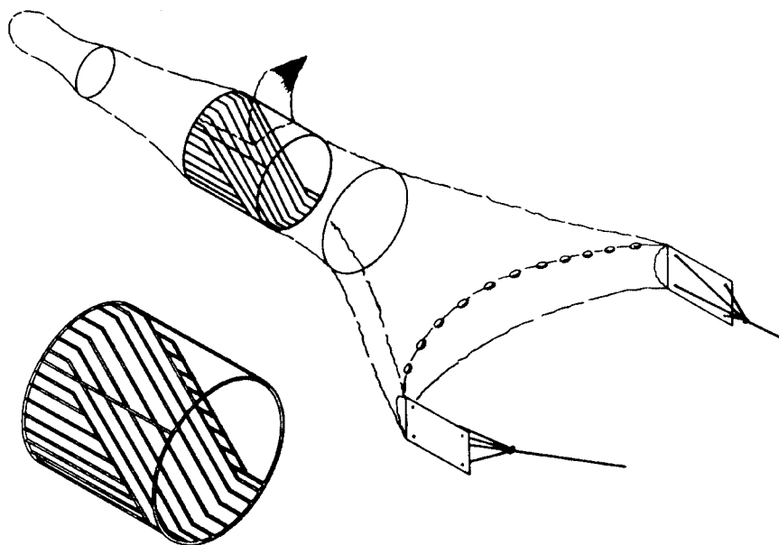
FIGURE 2 TO PART 223—CAMERON TED
