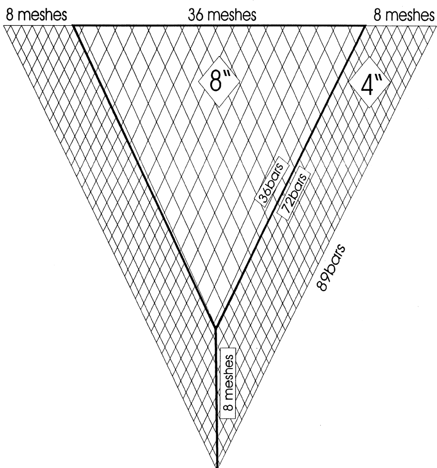
Parker Soft TED
