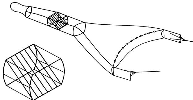
FIGURE 1 TO PART 223—NMFS TED
