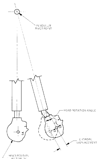
FIGURE 40-3 NECK COMPONENT TEST
