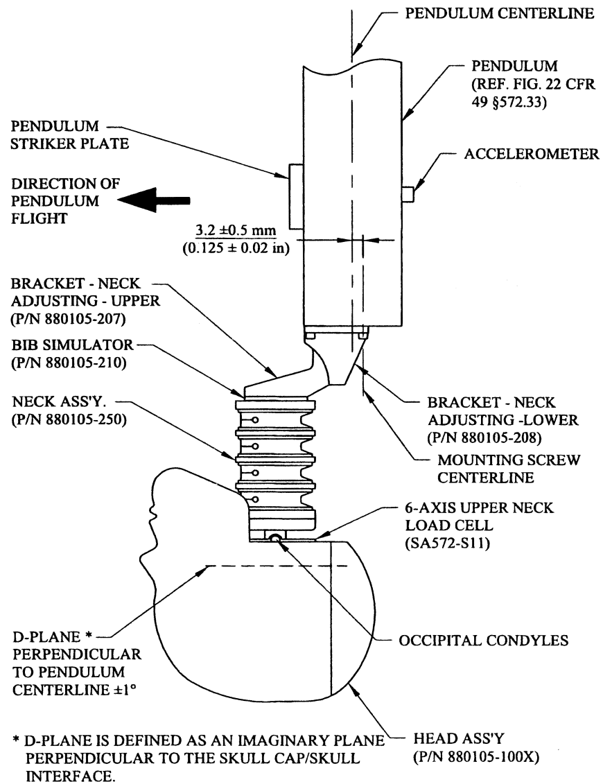
FIGURE O1 NECK FLEXION TEST SETUP SPECIFICATIONS
