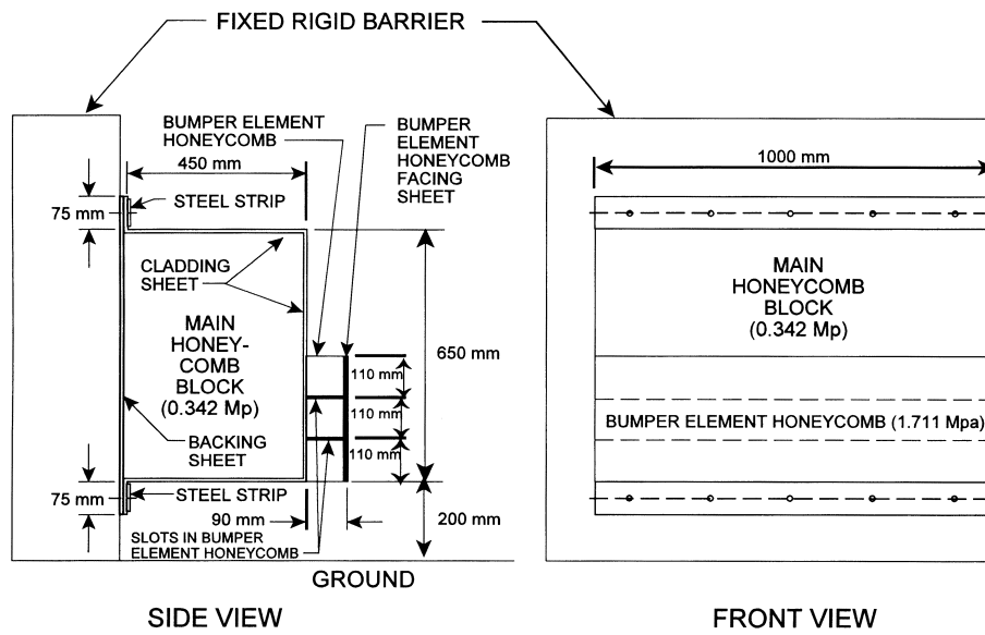
FIGURE 1 OFFSET BARRIER
