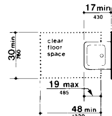
Fig. 32 Clear Floor Space at Lavatories
