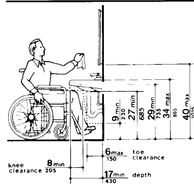
Fig. 31 Lavatory Clearances
