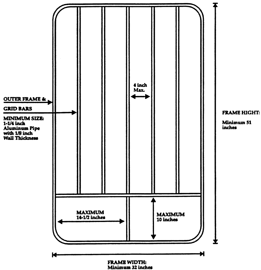
FIGURE 10 TO PART 223—FLOUNDER TED
