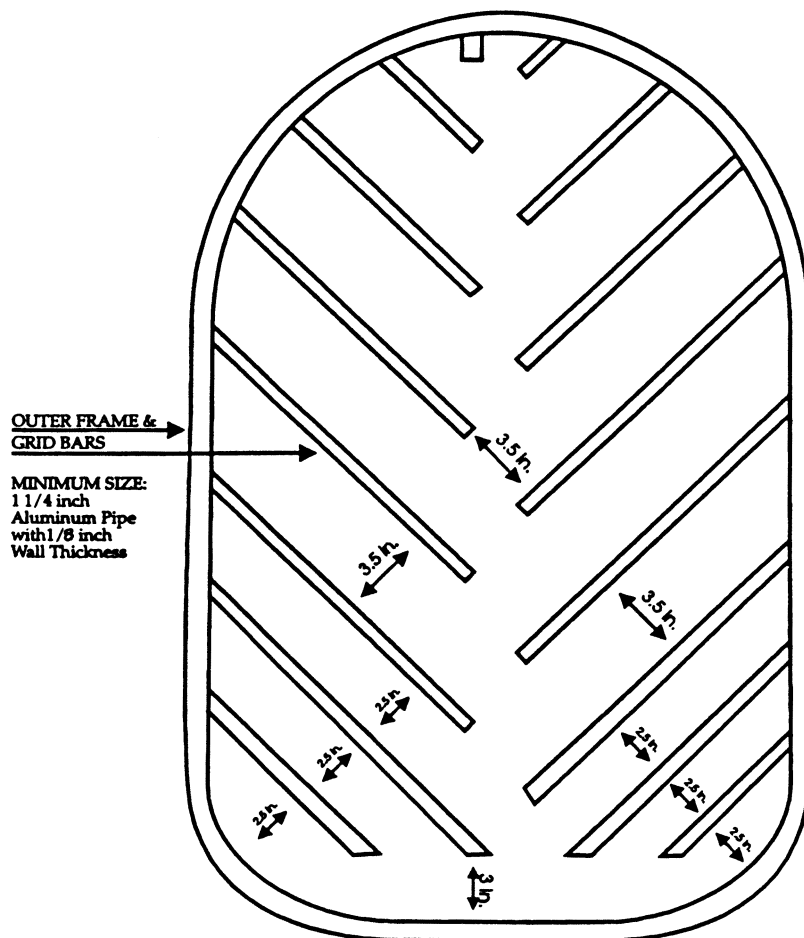
FIGURE 11 TO PART 223—JONES TED
