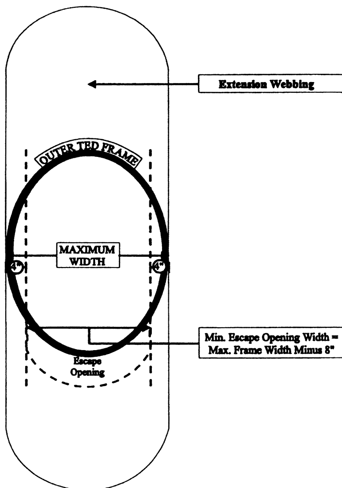
FIGURE 13 TO PART 223—SINGLE GRID HARD TED ESCAPE OPENING [60 FR 15520, Mar. 24, 1995]
