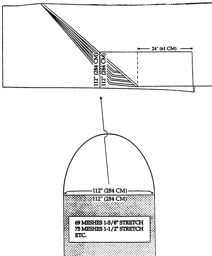
FIGURE 12B TO PART 223—GRID TED LEATHERBACK MODIFICATION
