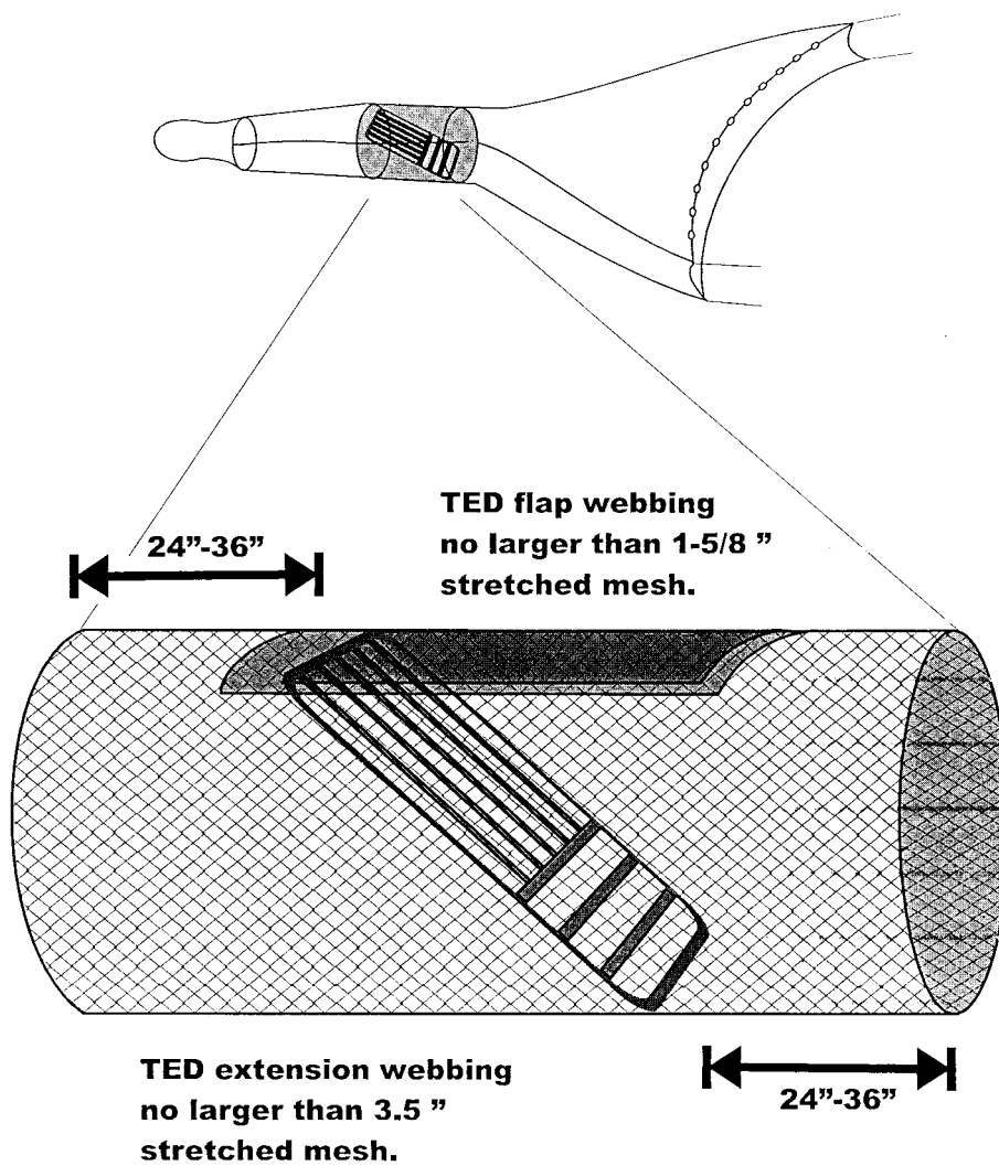
FIGURE 6 TO PART 223—TED EXTENSION IN SUMMER FLOUNDER TRAWL [64 FR 55864, Oct. 15, 1999]
