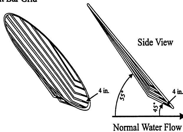
FIGURE 14B TO PART 223—MAXIMUM ANGLE OF DEFLECTOR BARS WITH BENT BARS ATTACHED TO THE BOTTOM OF THE FRAME
