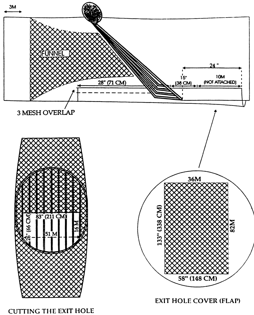
FIGURE 12A TO PART 223—ATTACHMENT OF THE EXIT HOLE COVER [59 FR 25830, May 18, 1994]
