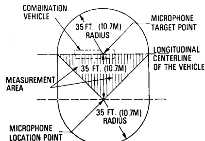
Figure 4 NON-STANDARD TEST SITE: (35 FT (10.7M) DISTANCE BETWEEN MICROPHONE LOCATION AND TARGET POINTS)
