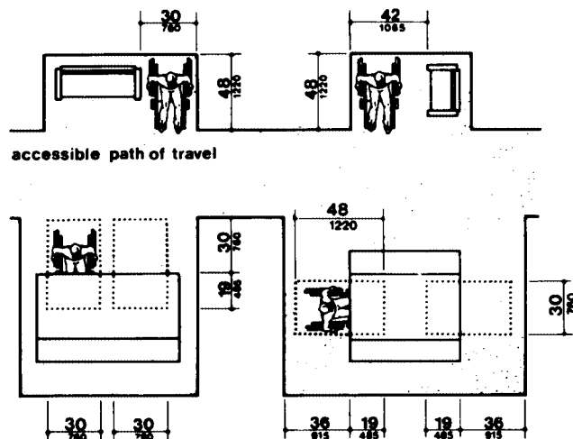
Fig. 45 Minimum Clearances for Seating and Tables
