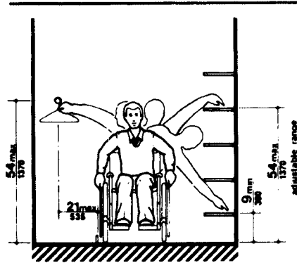
Fig. 38 Storage Shelves and Closets
