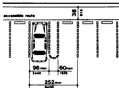
Fig. 9 Dimensions of Parking Spaces
