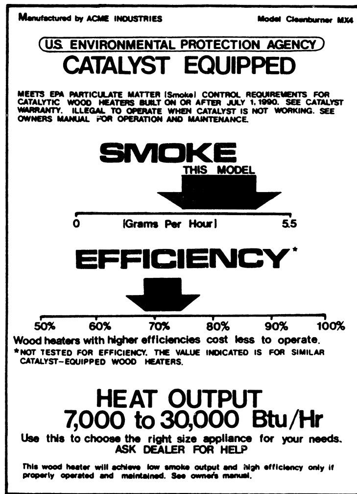
Figure 1. Temporary label for hypothetical wood heater: (1) catalytic, (2) estimated efficiency, and (3) meets 1990 standard. Emissions: 3.5 g/hr Efficiency: 72 percent
