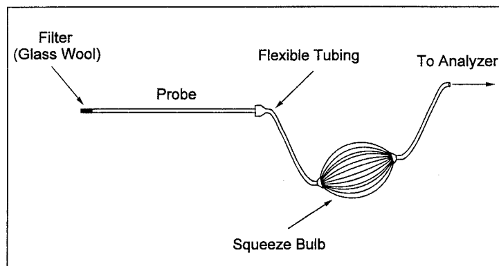
Figure 3-1. Grab-Sampling Train.
