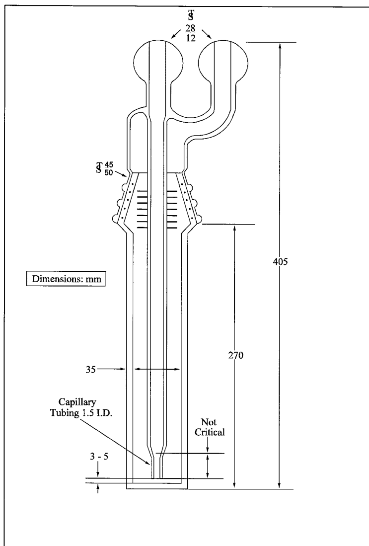
Figure 7C-2. Restricted-Orifice Impinger.
