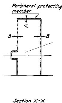
Section X-X
