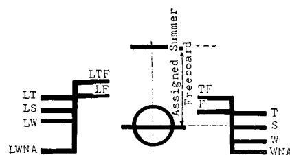
FIGURE 42.13-25(a)—Load line mark and lines to be used with this mark.
