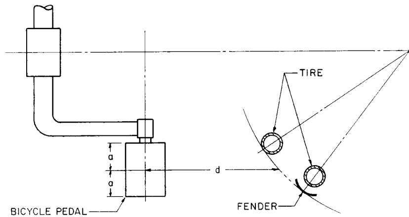
FIG 6-TOE CLEARANCE
