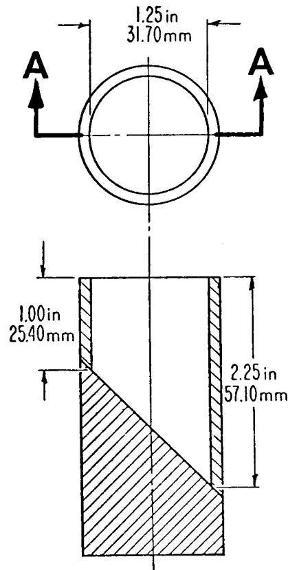
FIG 2-SMALL PARTS GAGE
