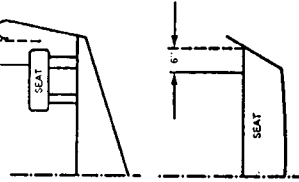
FIGURE 13. LOCATION OF CENTER OF GRAVITY OF WEIGHTS ON SEATS
