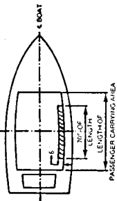
FIGURE 11. PASSENGER CARRYING AREA: LOCATION OF CENTER OF GRAVITY OF WEIGHTS
