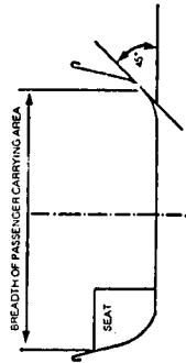
FIGURE 12. STABILITY TEST LOCATION OF CENTER OF GRAVITY OF WEIGHTS: STARBOARD SIDE
