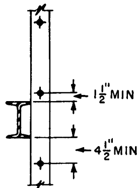
Minimum Ladder Clearances
