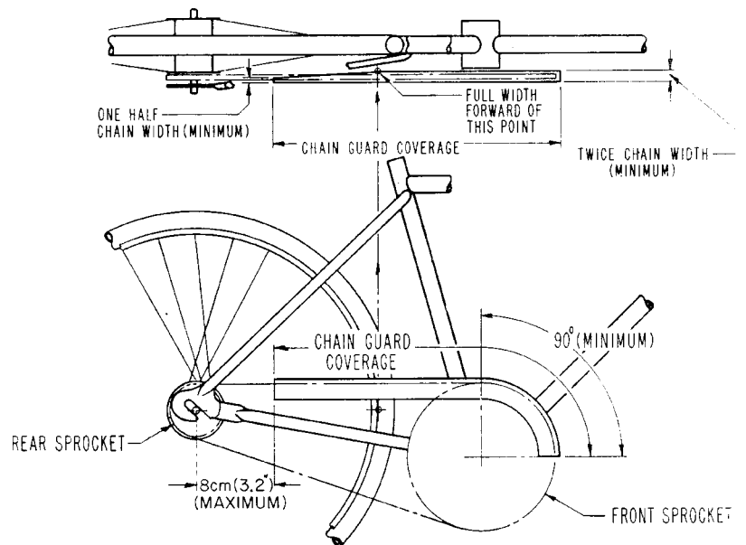
FIG 7-CHAIN GUARD REQUIREMENTS
