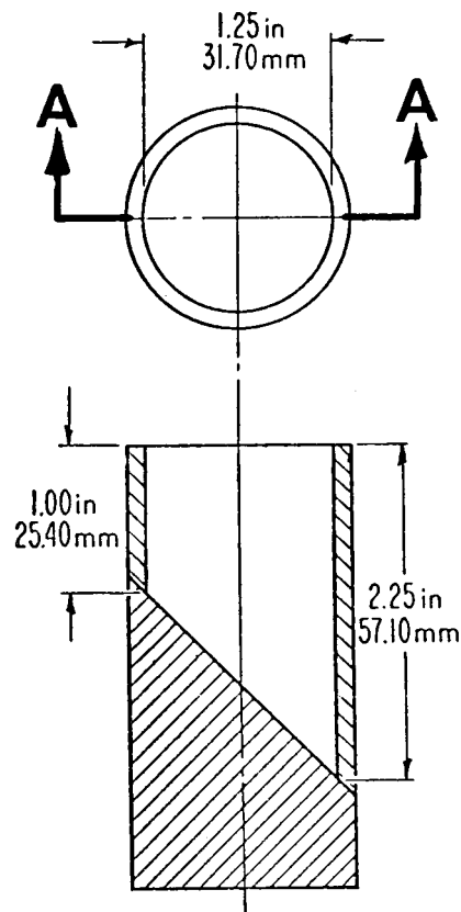
FIG 2-SMALL PARTS GAGE
