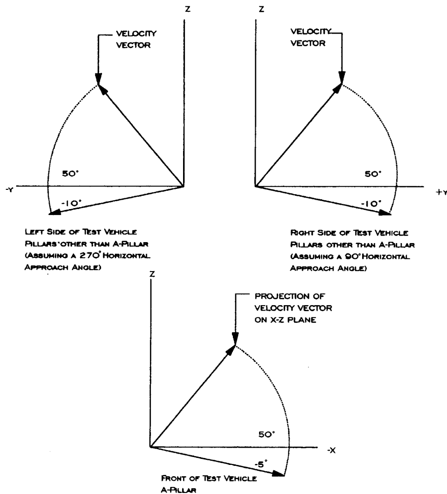
VERTICAL AND HORIZONTAL APPROACH ANGLE PLANE
