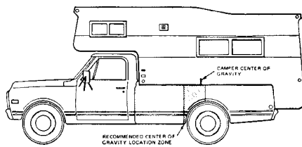
FIGURE 3. EXAMPLE OF PROPER TRUCK AND CAMPER MATCH
