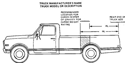
FIGURE 1 - TRUCK LOADING INFORMATION
