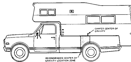
FIGURE 2 - EXAMPLE OF PROPER TRUCK AND CAMPER MATCH
