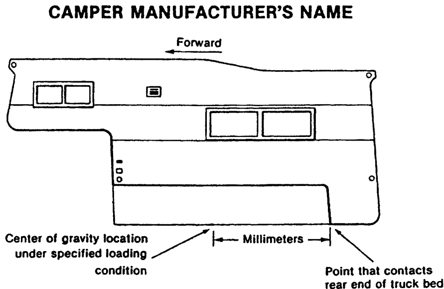
Figure 2.—Camper Center Of Gravity Information
