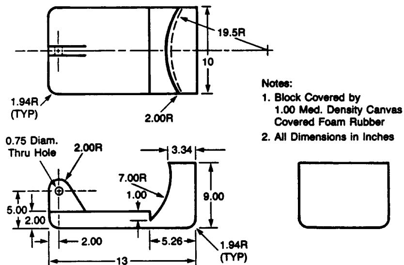
Figure 2B Optional Body Block for Center Seating Positions
