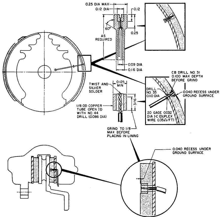
FIGURE 2 THERMOCOUPLE INSTALLATION
