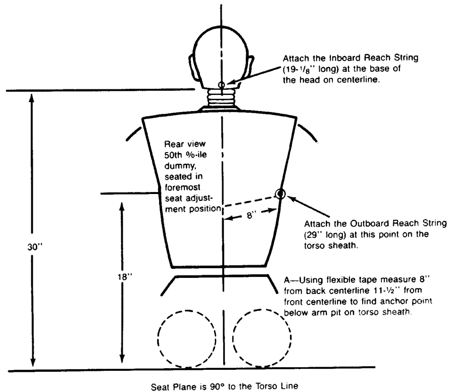
Figure 3b. — Location of Anchoring Points for Latchplate Reach Limiting Chains or Strings to Test for Latchplate Accessibility Using Subpart E Test Device
