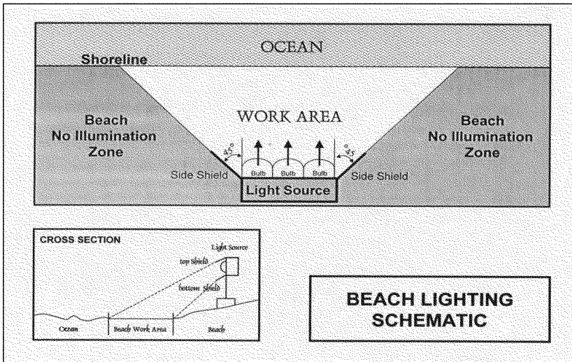
Figure 15. Beach lighting schematic.
