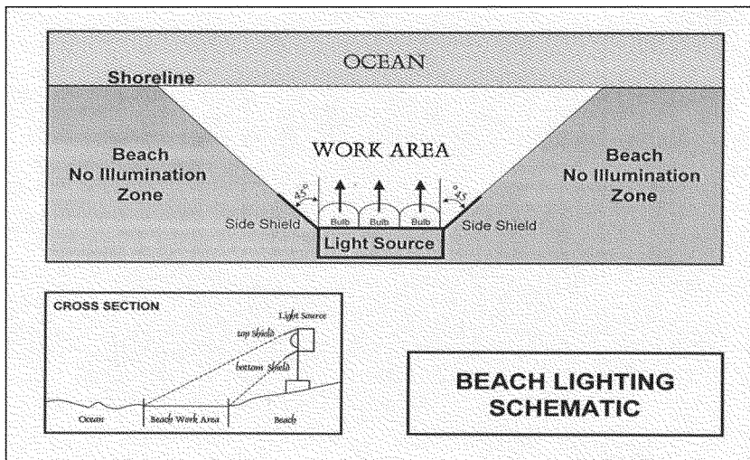
Figure 19. Beach lighting schematic.
