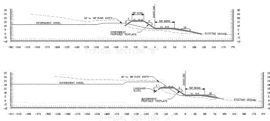
Selected plan typical cross sections to be constructed
