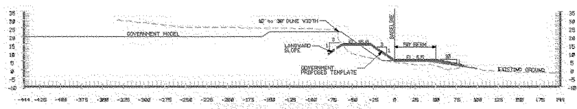
Selected plan typical cross sections to be constructed
