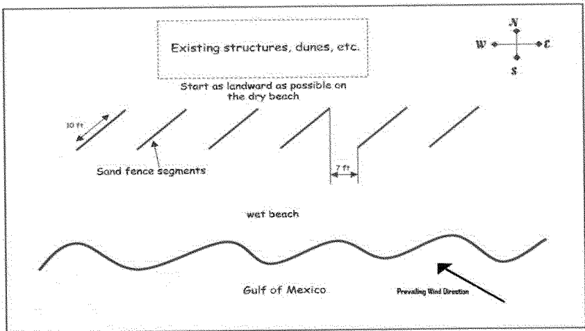
Figure 20. Dune restoration fence alignment.
