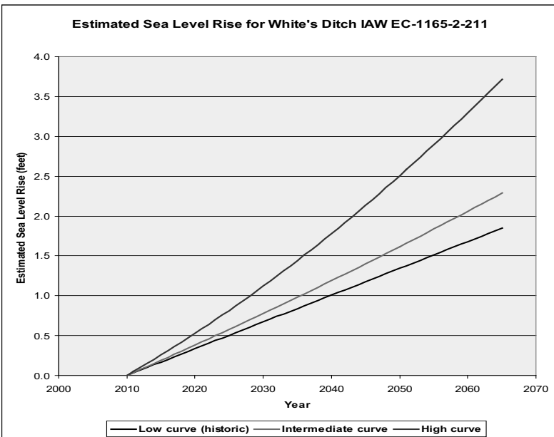
Figure 7-2: Sea level rise rates for the White Ditch Study Area
