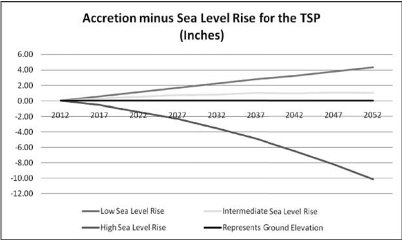
Figure 5-8: Accretion minus sea level rise for the recommended plan
