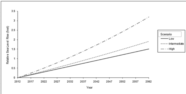
Figure 5-5: Projected RSLR over project life
