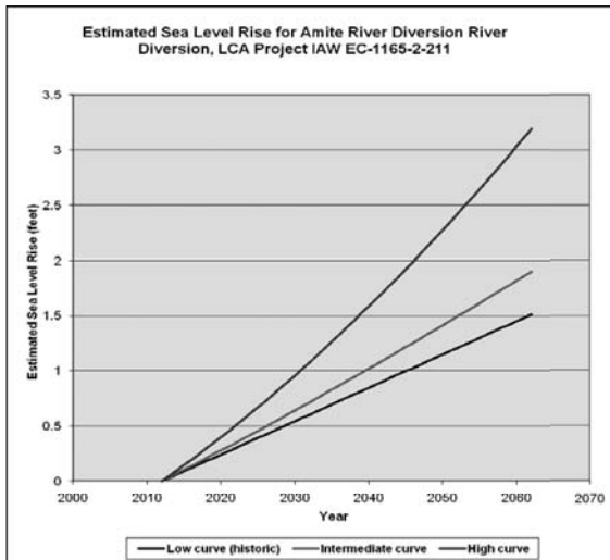
Figure 3-4: Sea level rise for Study Area
