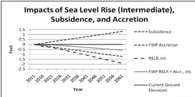
Figure 3-6: Impacts of Intermediate Sea Level Rise, Subsidence, and Accretion
