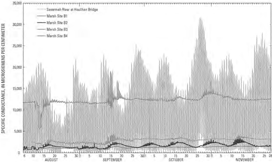
Figure 16. Hourly specific conductance at four marsh gaging stations along the Little Back and Back Rivers and specific-conductance values at the Houlihan Bridge on the Savannah River for the period August 6 to November 30, 2001.
