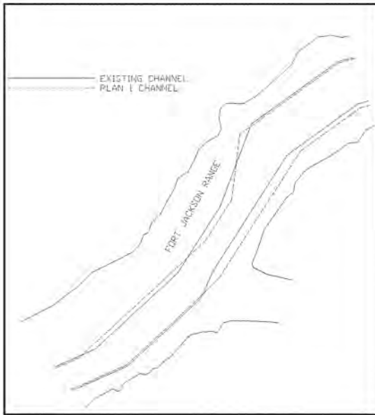
Figure 7. Fort Jackson Range, Plan 1
