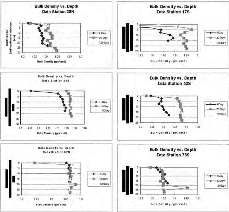
Figure A-6: Bulk density profiles for Sedflume cores consolidated 4, 20, and 120 days
