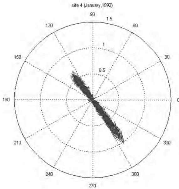
Figure 54. Current vectors at site 4 (current speed in m/s)
