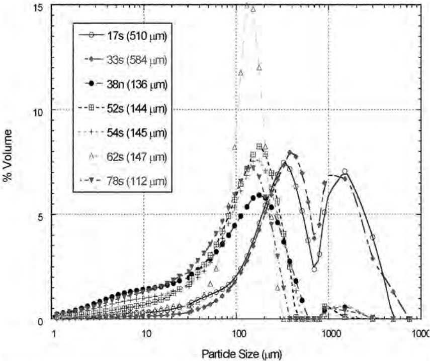
Figure 4-4. Particle size volume distribution for six Sedflume sample sites.
