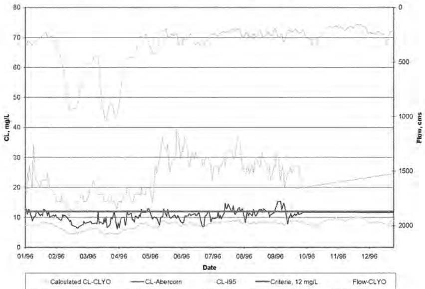
Figure 5-6 Calculated Chloride Time Series at Clio - 1996
