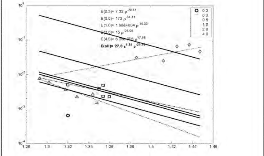
Figure A-5d: Erosion data for Site 78S
