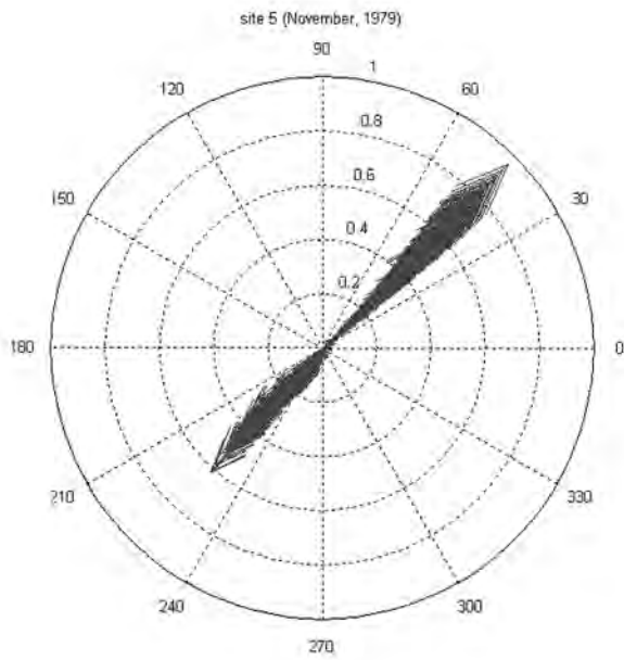
Figure 42. Current vectors at site 5 (current speed in m/s)
