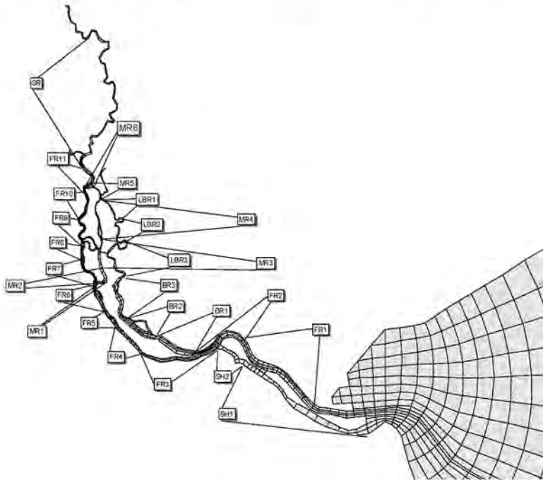
Figure 2-3 Zones' Delineation of Savannah Estuary Computational Grid
