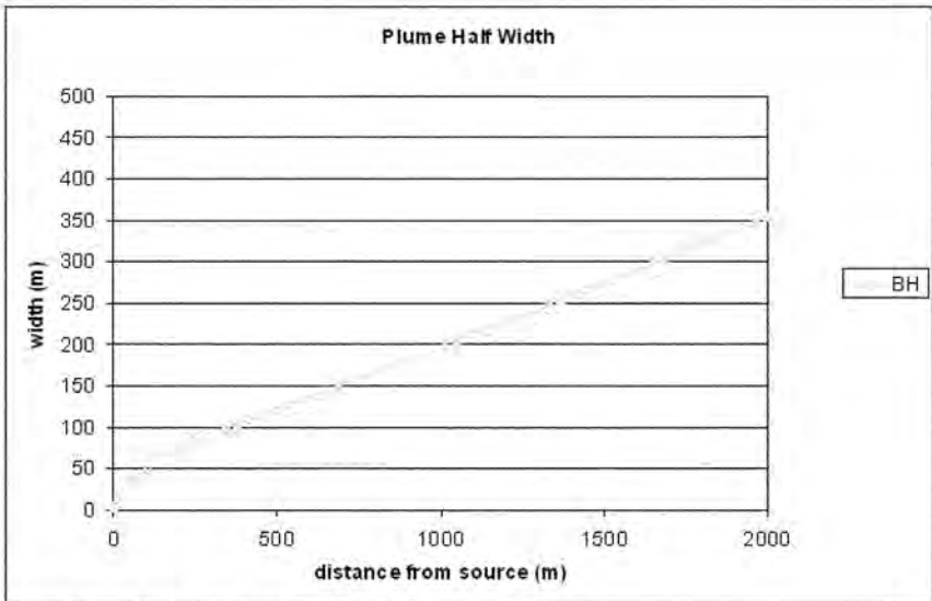
Figure 5-10b: Plume gaussian half width, simulation riv10h
