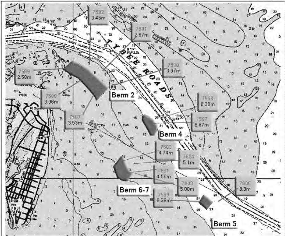
Figure 4-18. Locations for GTRAN erosion calculation; mounds 2,4-7.
