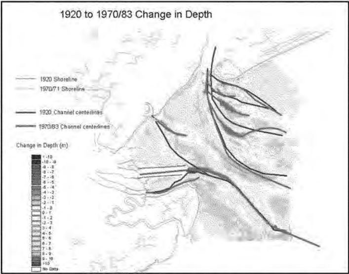
Figure 2-20. 1920 to 1970/83 change in bathymetry.
