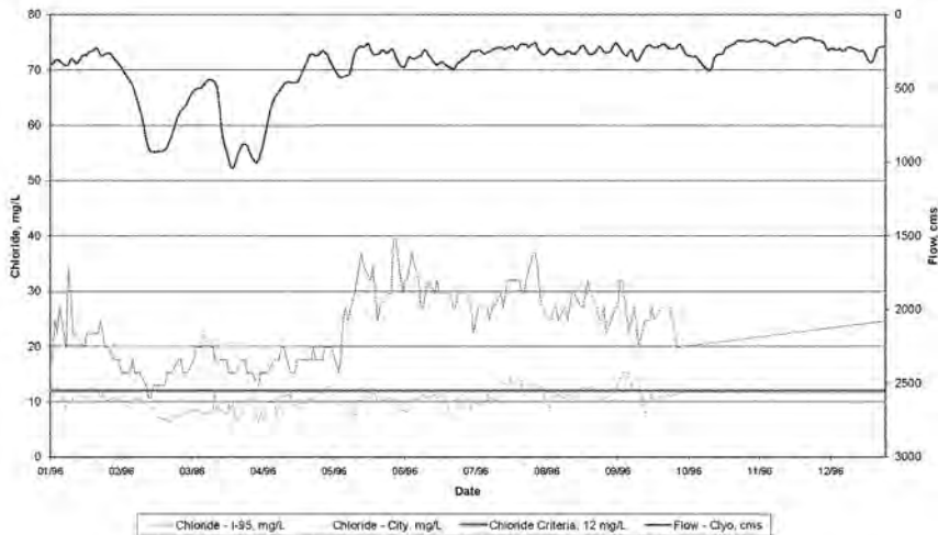
Figure 4-4 Chloride Values and Corresponding Flow Measurements for 1996
