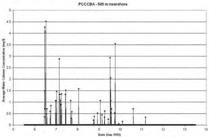
Figure 5-5d: SSFATE simulation PCCCAA, depth-averaged time-series concentration 500m toward shore from the source
