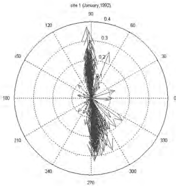
Figure 51. Current vectors at site 1 (current speed in m/s)
