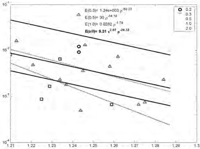
Figure A-5a: Erosion data for Site 38N
