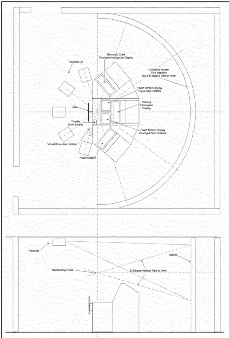
Figure 15. Arrangement of ERDC Ship/Tow bridge module
