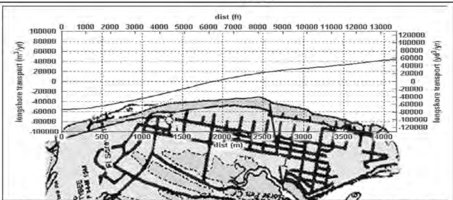
Figure 4-11. Average annual net longshore sediment transport rate estimated by GENESIS along Tybee Island shoreline for 1976-1995 simulation.
