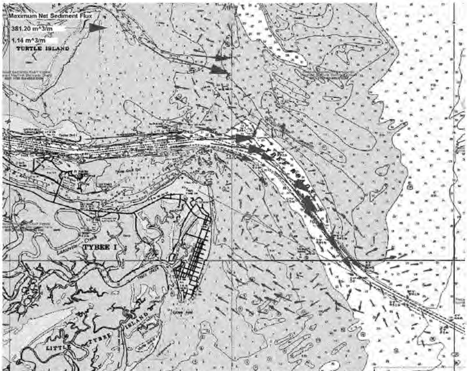
Figure 5B-1. Cumulative sediment transport vectors for November 1979 existing conditions GTRAN simulation.
