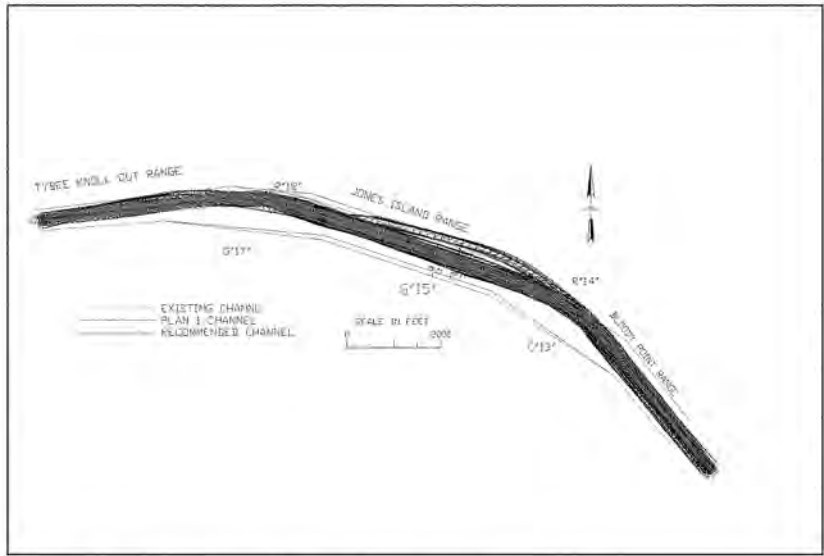
Figure 22. 43-ft draft Susan Maersk at Jones Island Range Turn
