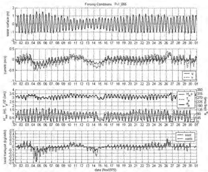
Figure 4-21a Time-series of water level, current, waves, and transport for November 1979 at Point 65 (Figure 4-20)
