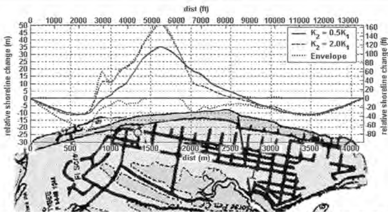
Figure 4-15. Relative change in shoreline between the Berm 14 and base case. Solid line represents range in solutions within the uncertainty in the value of K_2 . Dotted line indicates range of relative shoreline change over the 20-year simulation.
