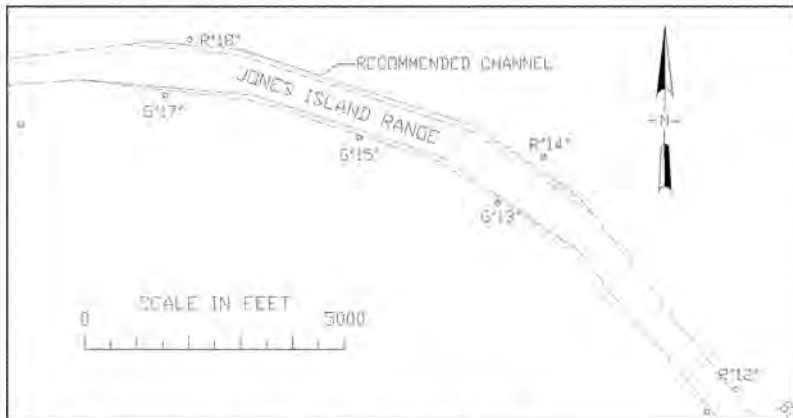
Figure 26. Recommended widener for Jones Island Range
