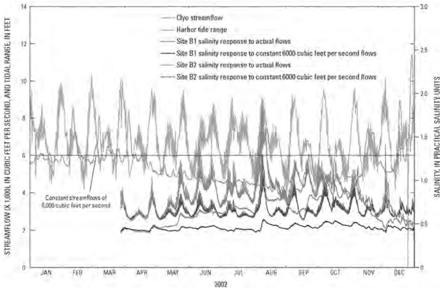
Figure 46. Hourly salinity response for two tidal marsh sites (B1 and B2) off the Little Back River for calendar year 2002 streamflows and constant 6,000 ft 3 /s streamflows. Tidal range for Savannah River at Fort Pulaski (station 02198980) also are shown.
