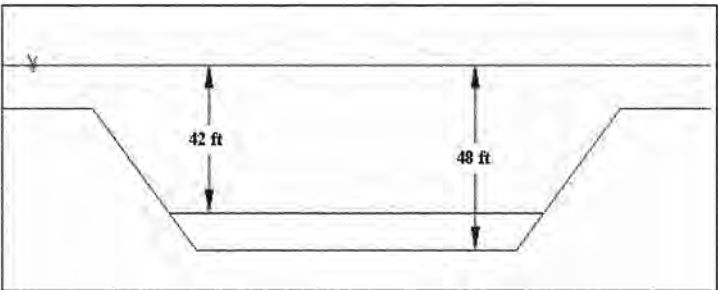
Figure 2. Channel deepened on existing side slopes
