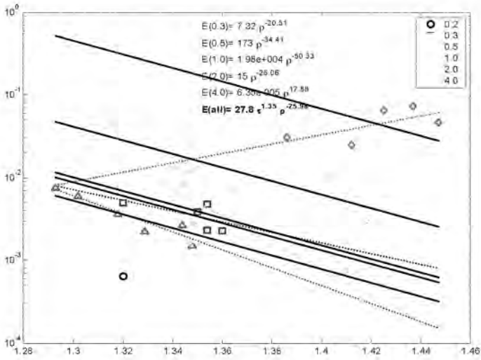
Figure 4-6. Erosion data and equation at Site 78S.
