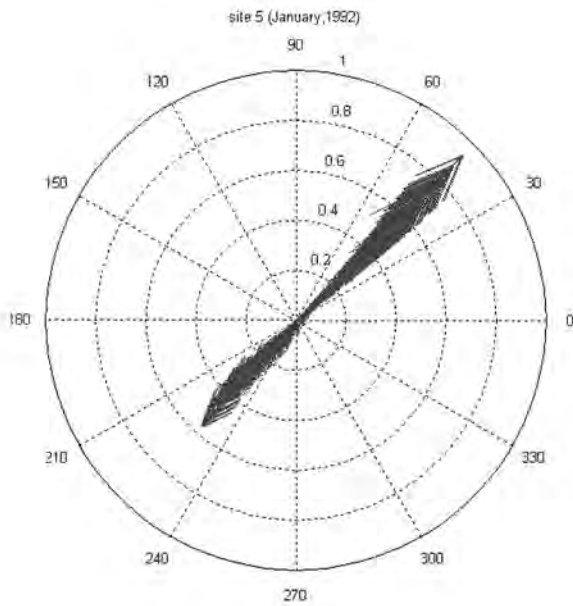
Figure 55. Current vectors at site 5 (current speed in m/s)
