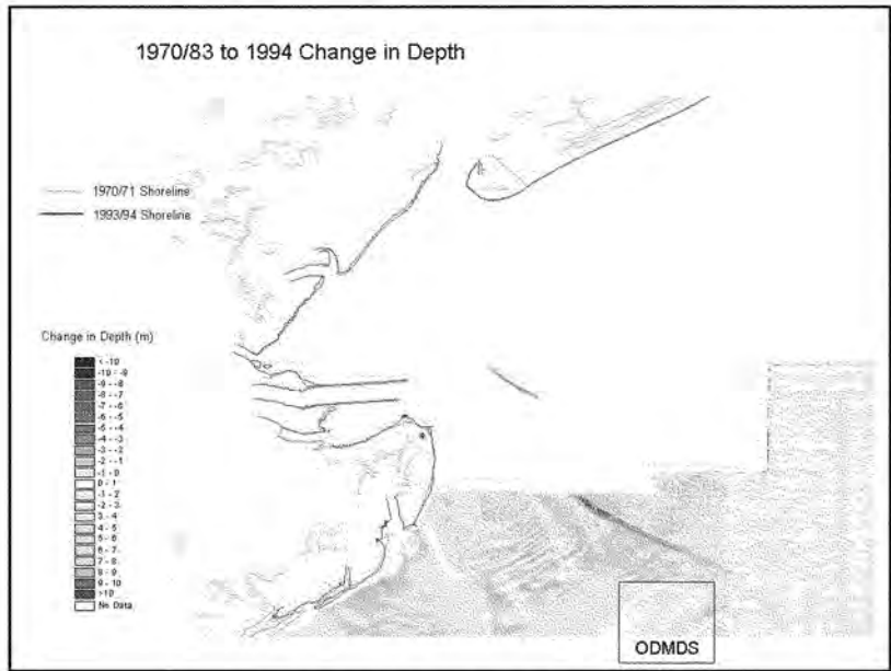
Figure 2-22. 1970/83 to 1993/94 change in bathymetry.
