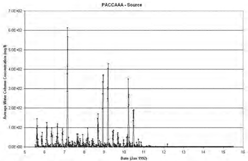
Figure 5-2a: SSFATE simulation PACCAAA, depth-averaged time-series concentration at the source
