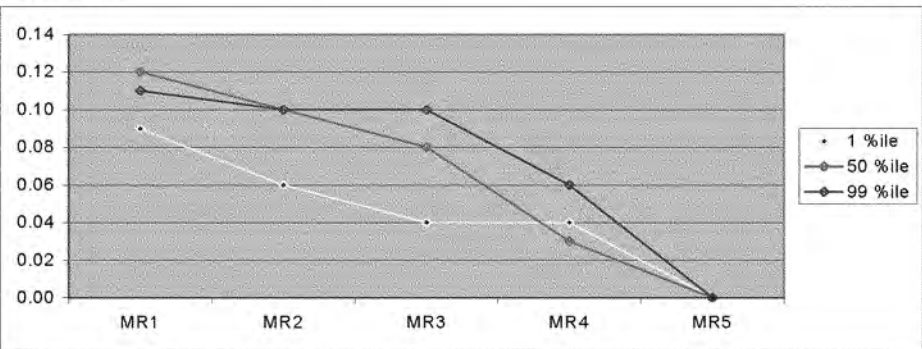
11. Figure C.1. Longitudinal profile of Dissolved Oxygen (mg/l) distribution along Critical cells of Savannah Estuary: Existing bathymetry
