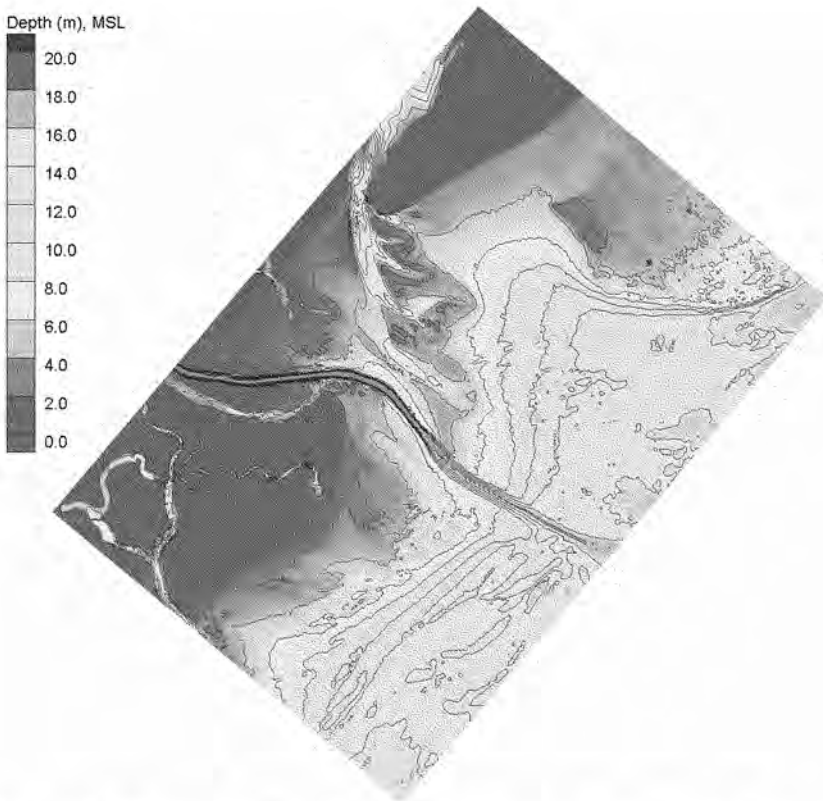
Figure 4-2. With-project grid (depths in meters, MSL). Land is shown in brown.
