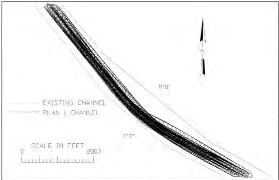
Figure 16. Composite S-class runs on turn between Tybee Range and Bloody Point Range
