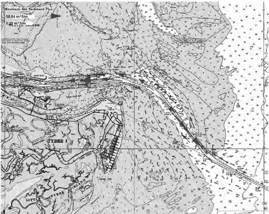
Figure 5D-1. Change in cumulative sediment transport vectors for November 1979 GTRAN simulation.
