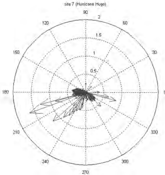
Figure 32. Current vectors at site 7 (current speed in m/s)
