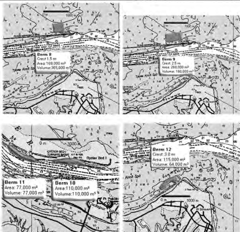
Figure 4-16. Berm location area, crest, and maximum volume
