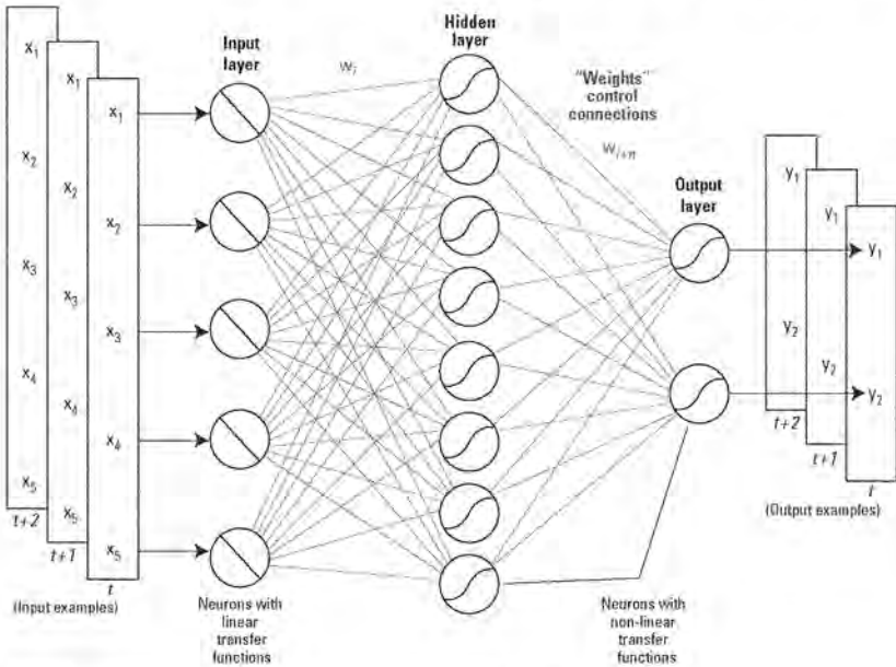
Figure 21. Multilayer perceptron artificial neural network architecture.
