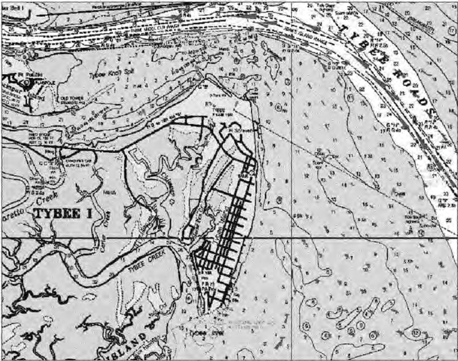
Sep 1989 Net Sediment Transport Under Existing Conditions
