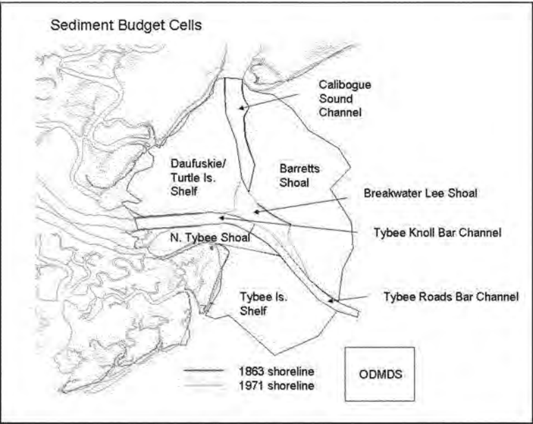
Figure 2-30. Volume Change Cells.
