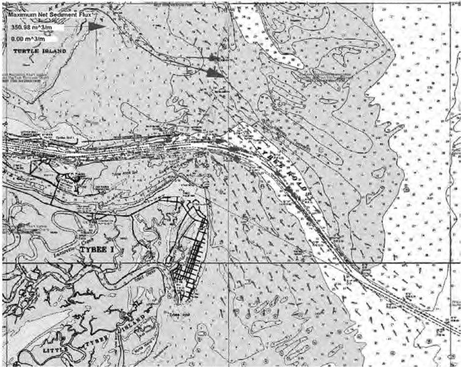
Figure 5B-8. Cumulative sediment transport vectors for July 1999 deepened conditions GTRAN simulation.
