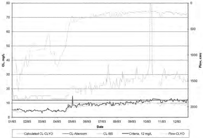
Figure 5-5 Calculated Chloride Time Series at Clio - 1993
