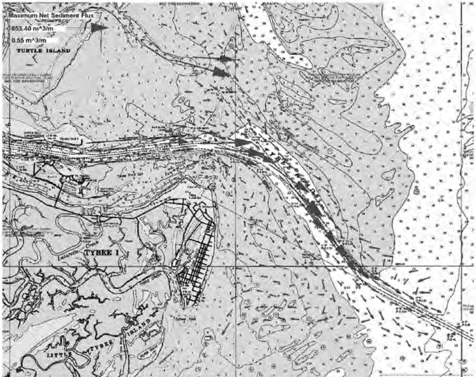
Figure 5B-4. Cumulative sediment transport vectors for September 1989 (Hugo) deepened conditions GTRAN simulation.
