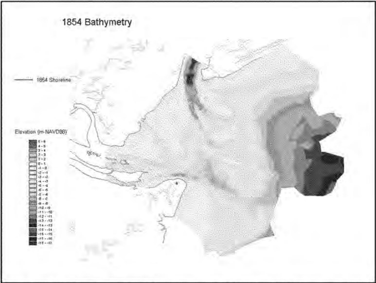
Figure 2-9. 1854 Bathymetry representing the pre 1871 project conditions.
