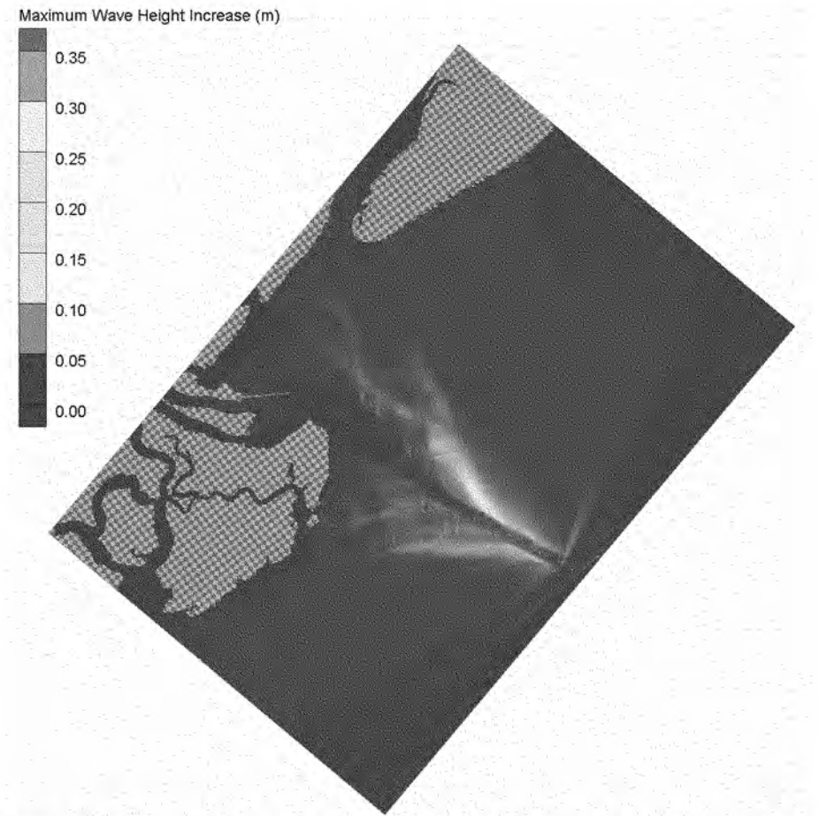
Figure 4-12. Maximum Wave Height Increases for Each Grid Cell for 1-30 November 1979. Maximum Increase of 0.12 m.
