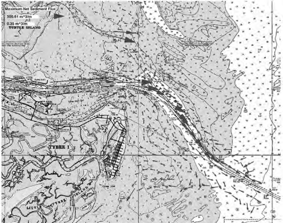
Figure 5B-3. Cumulative sediment transport vectors for September 1989 (Hugo) existing conditions GTRAN simulation.
