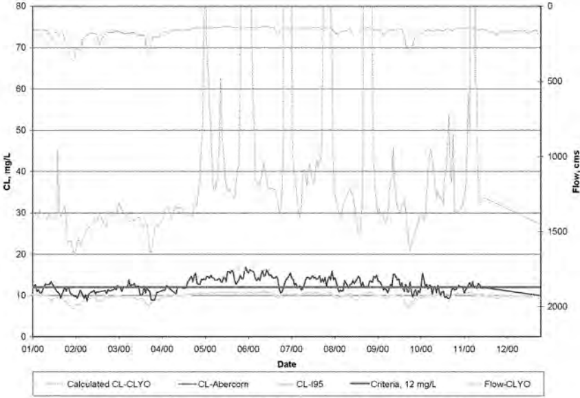
Figure 5-7 Calculated Chloride Time Series at Clio - 2000
