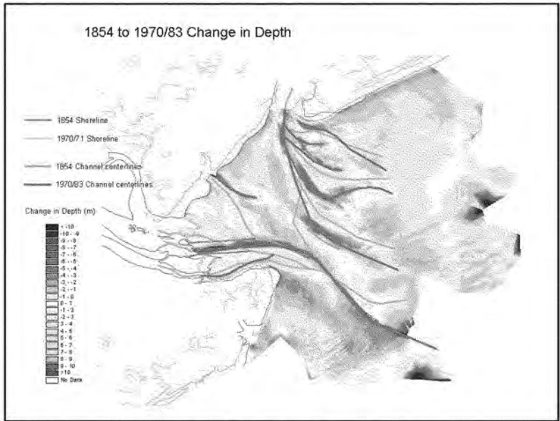
Figure 2-21. 1854 to 1970/83 change in bathymetry.
