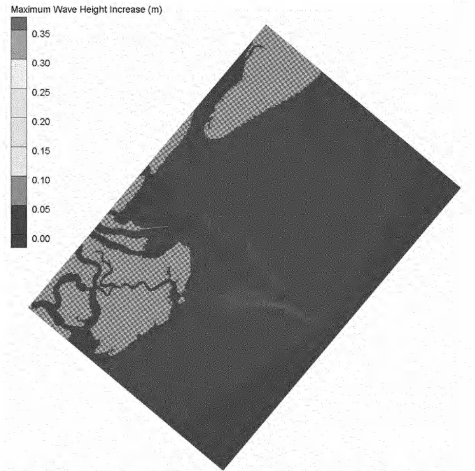
Figure 4-18. Maximum Wave Height Increases for Each Grid Cell for 1-31 July 1999. Maximum Increase of 0.05 m.
