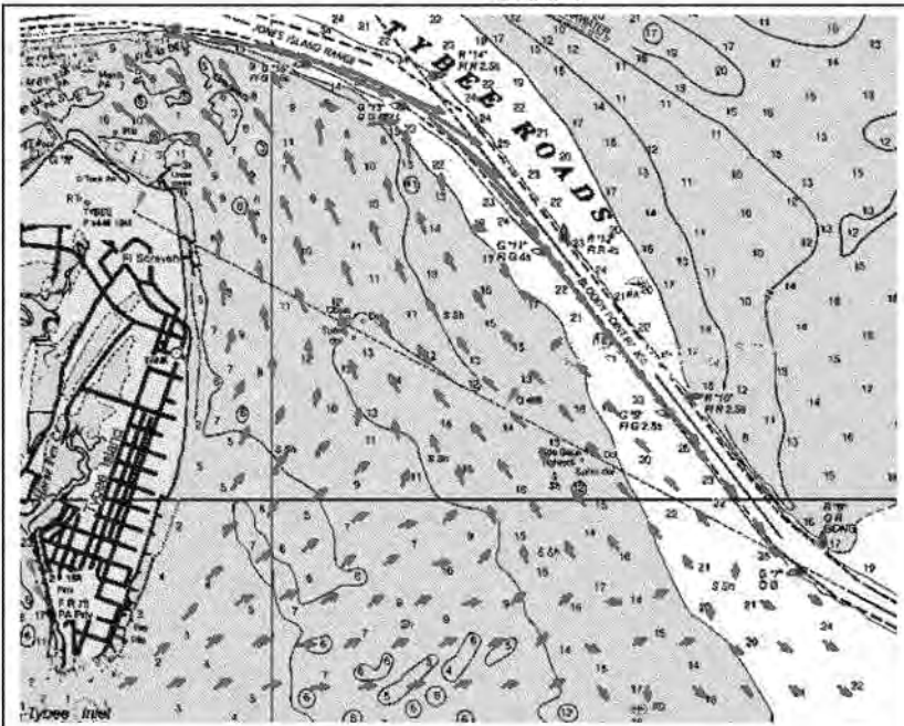
Figure 4-26. Net transport vectors for 24-year simulation (1976-1999). Note: not to same scale as presented in Figures 21 and 22.
