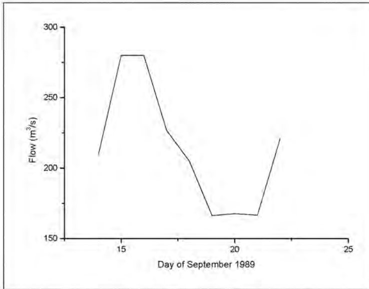
Figure 23. Daily discharge river flow for September 1989
