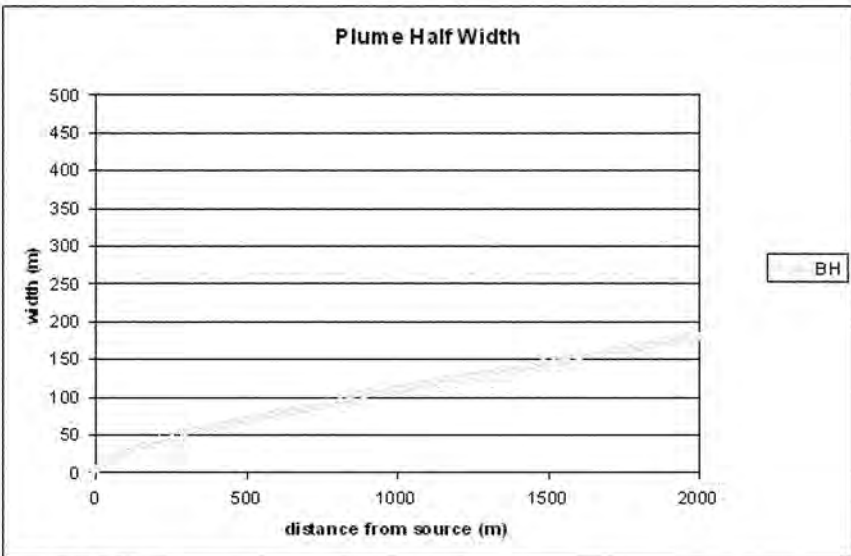
Figure 5-12c: Plume gaussian half-width, simulation tyb45cms
