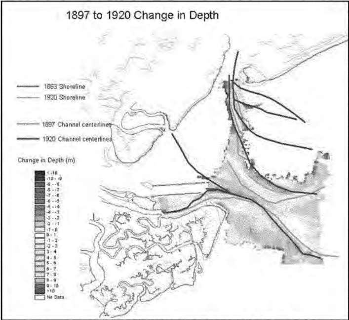
Figure 2-19. 1897 to 1920 change in bathymetry.
