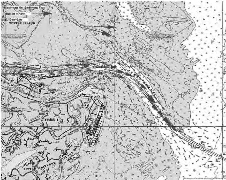
Figure 5D-2. Change in cumulative sediment transport vectors for September 1989 GTRAN simulation.
