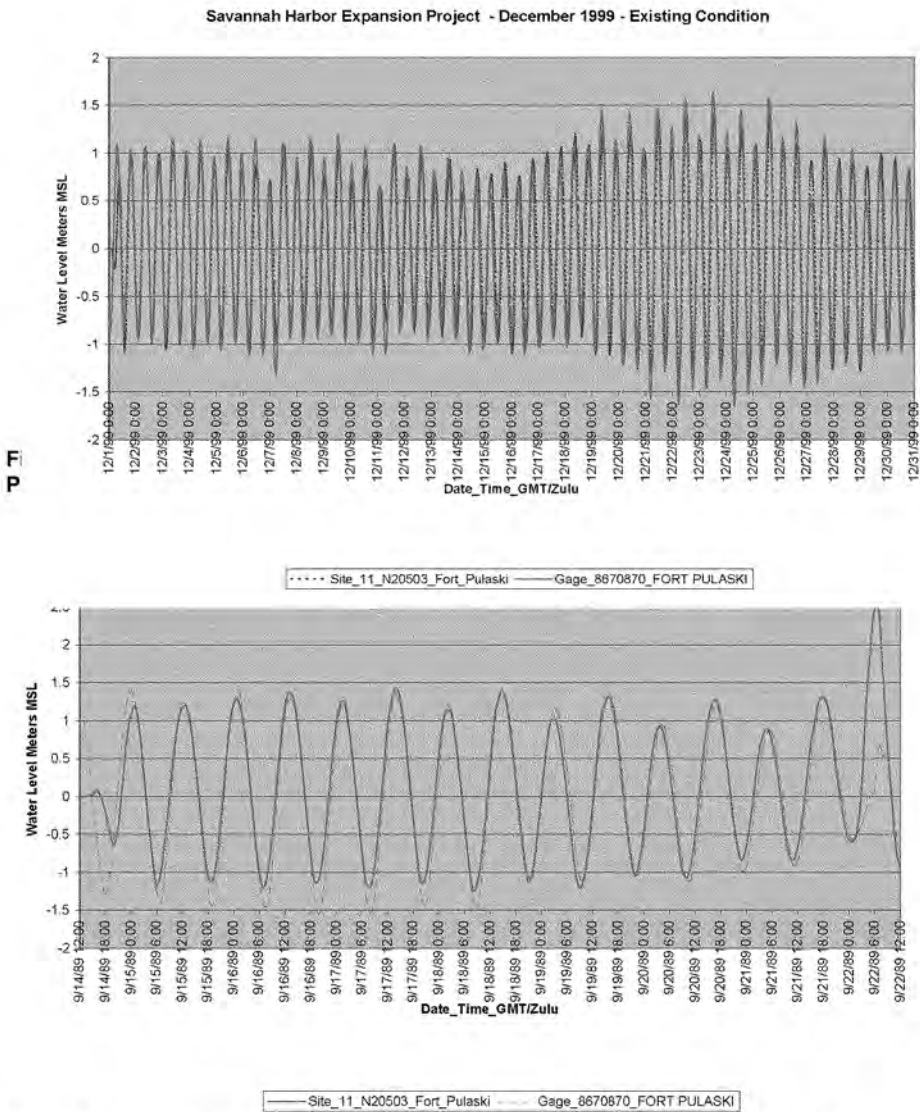
Figure 3-2. Comparison of measured and predicted water surface elevations for the retracted Hurricane Hugo. Note the divergence from measurements on 22 September when the storm track was altered to strike Savannah.
