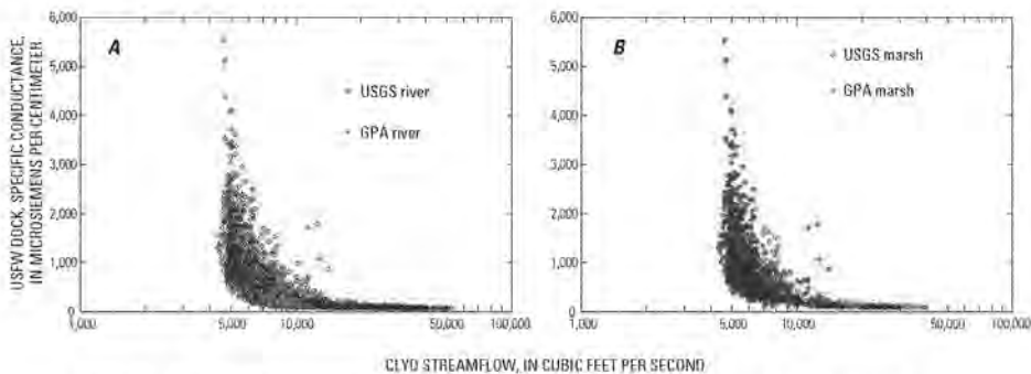
Figure 18. The daily mean streamflow at Savannah River at Clio, Ga., and daily mean specific conductance at U.S. Fish and Wildlife Service Dock, Little Back River, for the conditions during which the gaging network was active. The two river networks are shown in the plot on the left (A), and two marsh networks are shown on the plot on the right (B).
