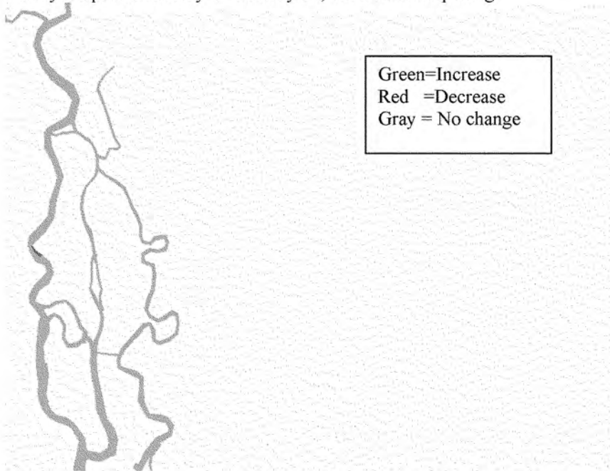
23. Figure A3.4 Change in a suitable for Sturgeon juveniles Habitat area within the analyzed period January 1 - January 31, 1999 : 4 ft deepening
