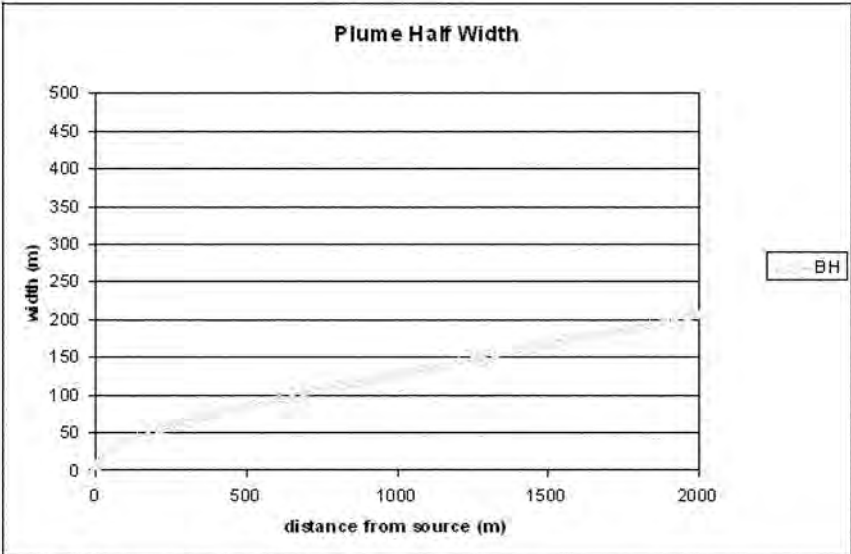
Figure 5-12b: Plume gaussian half-width, simulation tyb35cms
