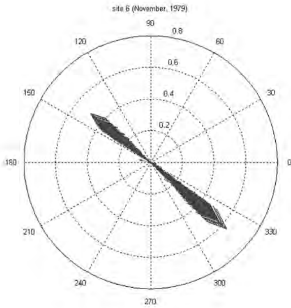
Figure 43. Current vectors at site 6 (current speed in m/s)
