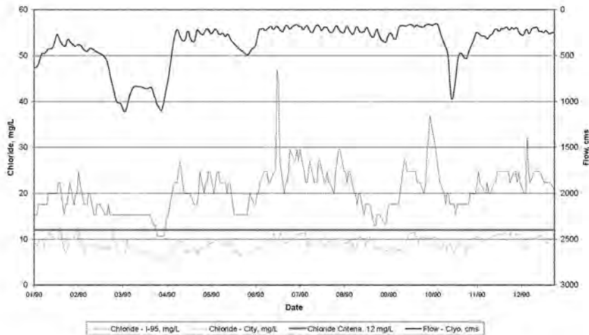
Figure 4-2 Chloride Values and Corresponding Flow Measurements for 1990
