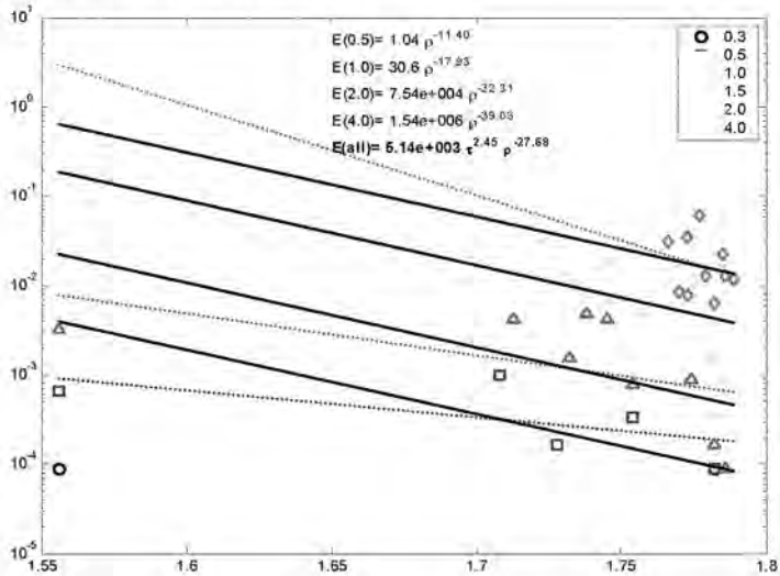
Figure A-5a: Erosion data for Site 38N
