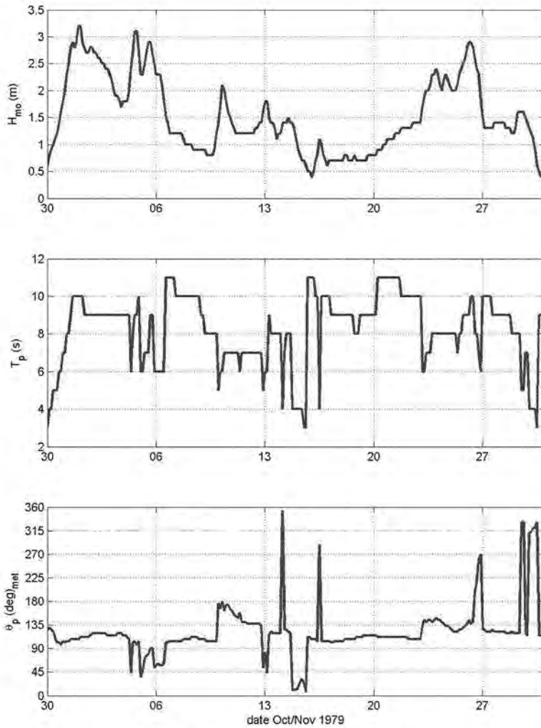
Figure 2-4. Offshore wave conditions for month of November 1979 at WIS sta 33. H_{m0} is energy-based wave height, T_p is the spectral peak period, \theta_p is the meteorological-convention wave direction (direction from which waves are approaching).
