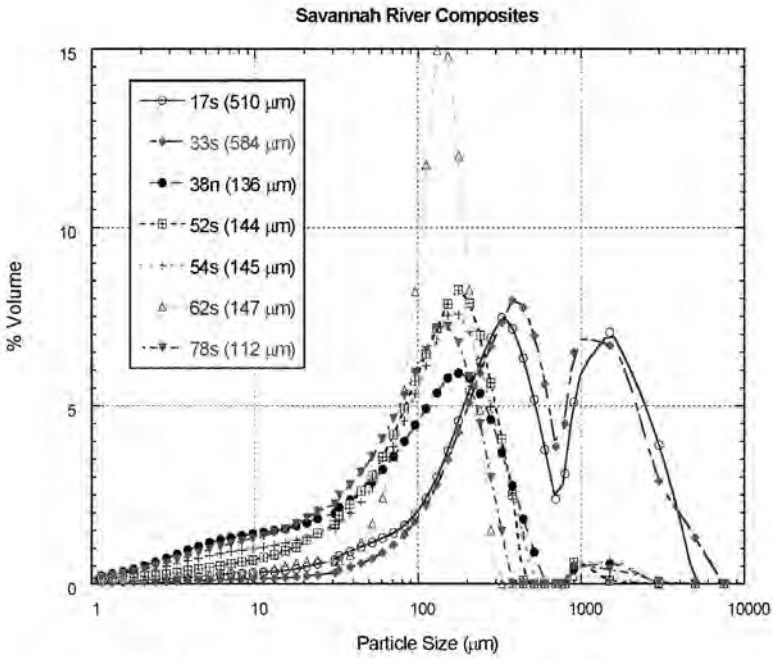
Figure A-4: Grain size distribution at six Sedlume analysis sites
