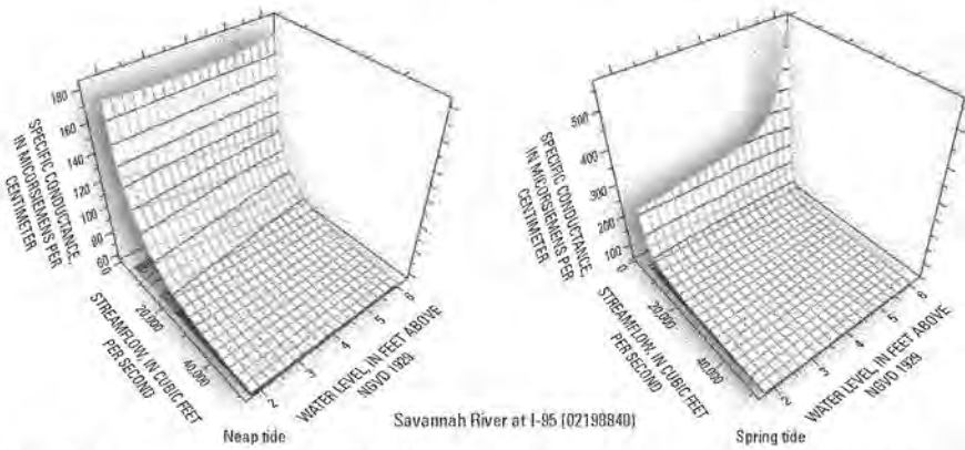
Figure 35. The interaction of water level (FWL8980A) and streamflow (Q8500A) on specific conductance at Savannah River at I-95 (station 02198840) for neap and spring tide conditions. The response surface on the left shows specific conductance response at the gage under neap tide conditions (all other input values set to the mean historical condition for both response surfaces). The response surface on the right shows the specific conductance response under spring tide conditions. Note differences in the z-axis (vertical) scale. During neap tides, salinity intrusion at I-95 is greatest during low-flow conditions through the full range of water-level conditions. During spring tides, salinity intrusion can be over twice as high as neap tide during low-flow and high water-level conditions.
