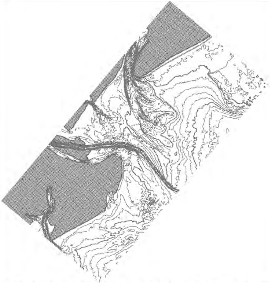
Figure 2-2. STWAVE nested grid bathymetry. Depths relative to Mean Sea Level (MSL). Contour interval 1 m and bold contours at 5 and 10-m depth.
