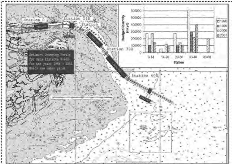
Figure 6-2. Recent pattern of channel maintenance dredging (length of the dark bars in the various channel sections indicate the magnitude of volume dredged)
