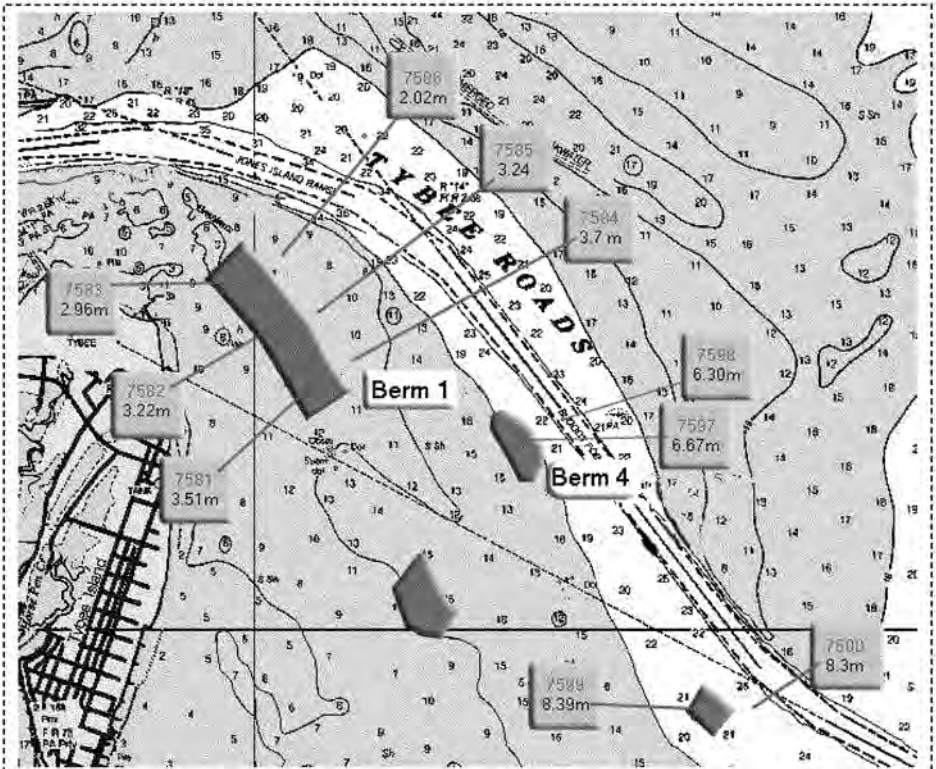
Figure 4-18. Locations for GTRAN erosion calculation: mounds 1,4,5.
