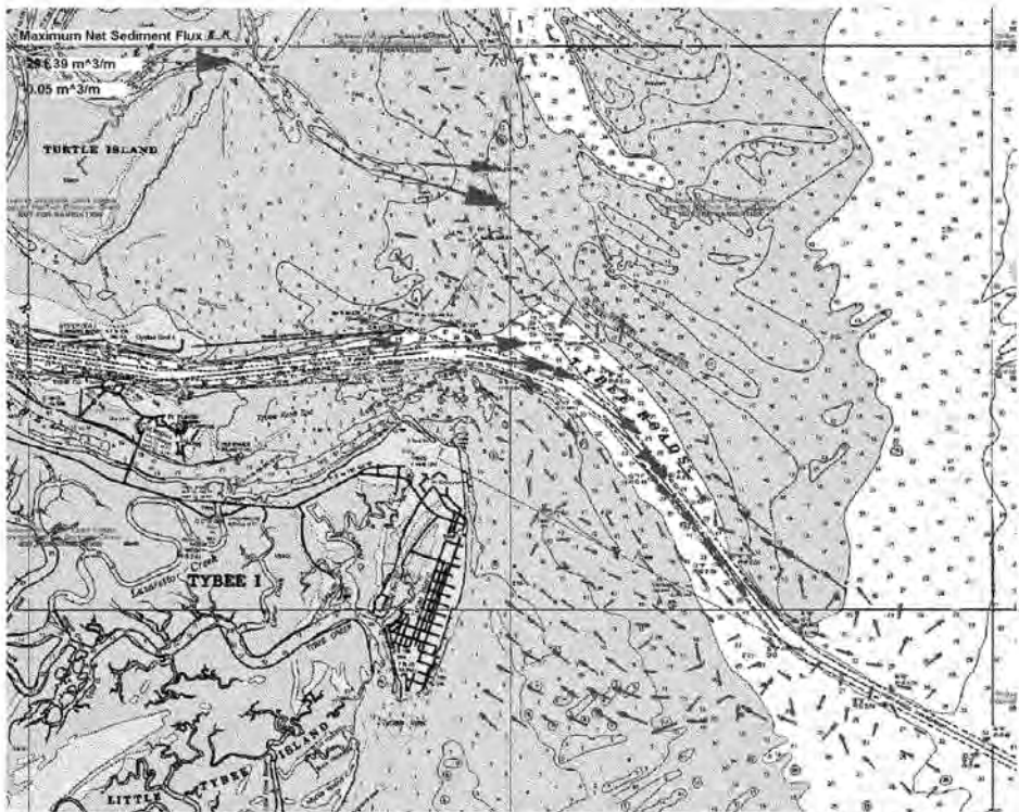
Figure 5B-5. Cumulative sediment transport vectors for January 1992 existing conditions GTRAN simulation.
