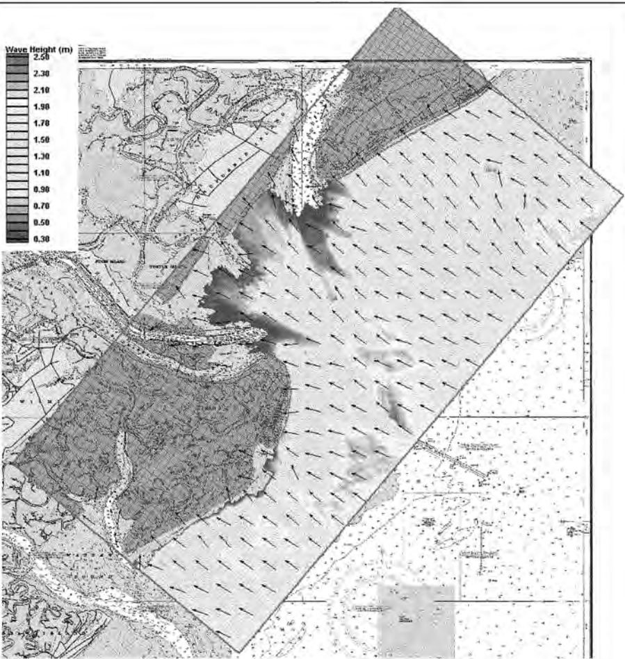
Figure 2-5. Wave transformation at mean low water over the nested grid for a frequently occurring energetic wave condition (Offshore wave conditions: H_{m0} = 1.75 , T_p = 9 sec, \theta_p = 118 deg true)
