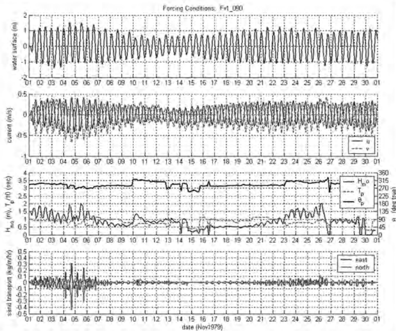
Figure 4-21f Time-series of water level, current, waves, and transport for November 1979 at Point 90 (Figure 4-20)
