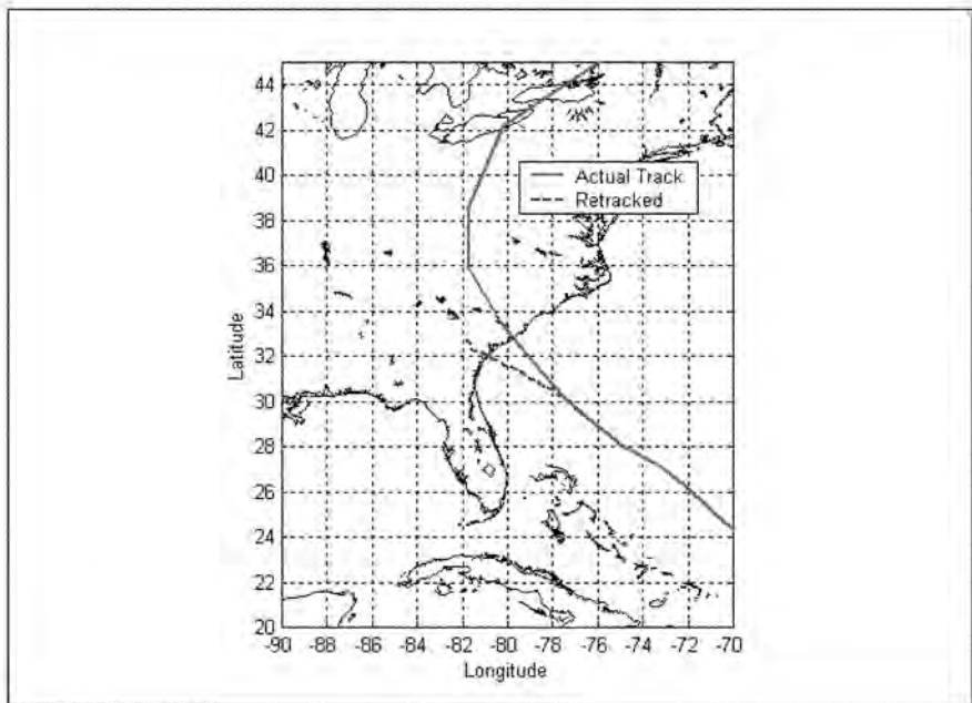
Figure 19. Actual and retracked Hurricane Hugo track
