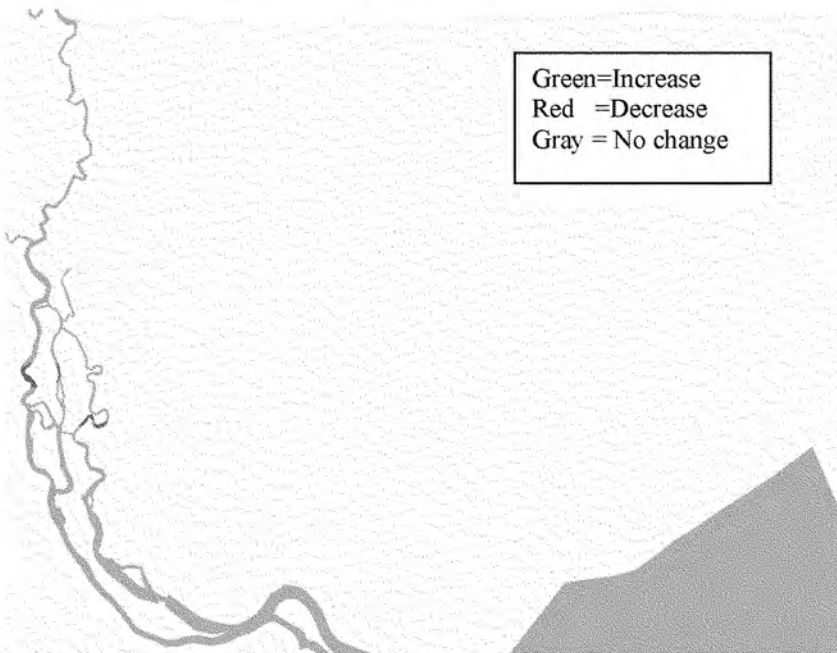
15. Figure C.1.2. Change in a suitable for Bass Spawning Habitat area within the analyzed period April 1 - April 30, 1999 : 6 ft deepening
