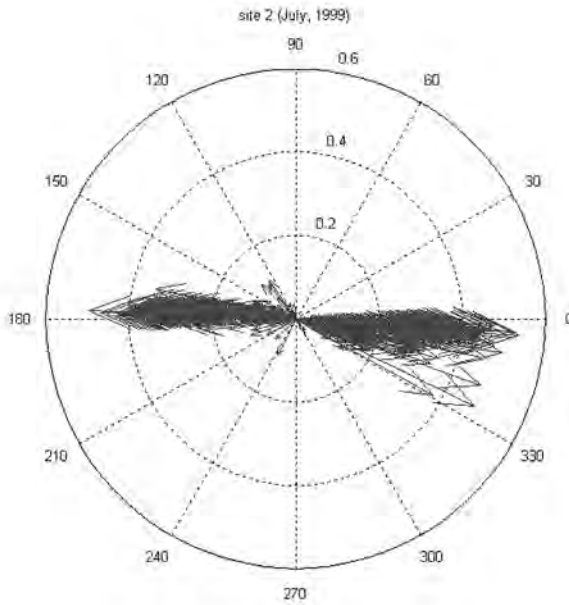
Figure 62. Current vectors at site 2 (current speed in m/s)
