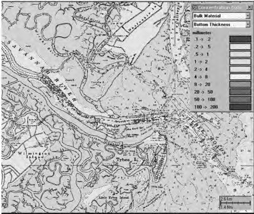
Figure 5-6: Bottom deposition after 4 days of dredging, simulation PBCCAA
