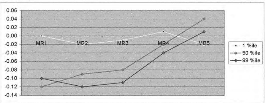
31. Figure A3.1. Changes in longitudinal profile of Dissolved Oxygen (mg/l) distribution along Critical cells of Savannah Estuary: 3 ft deepening
