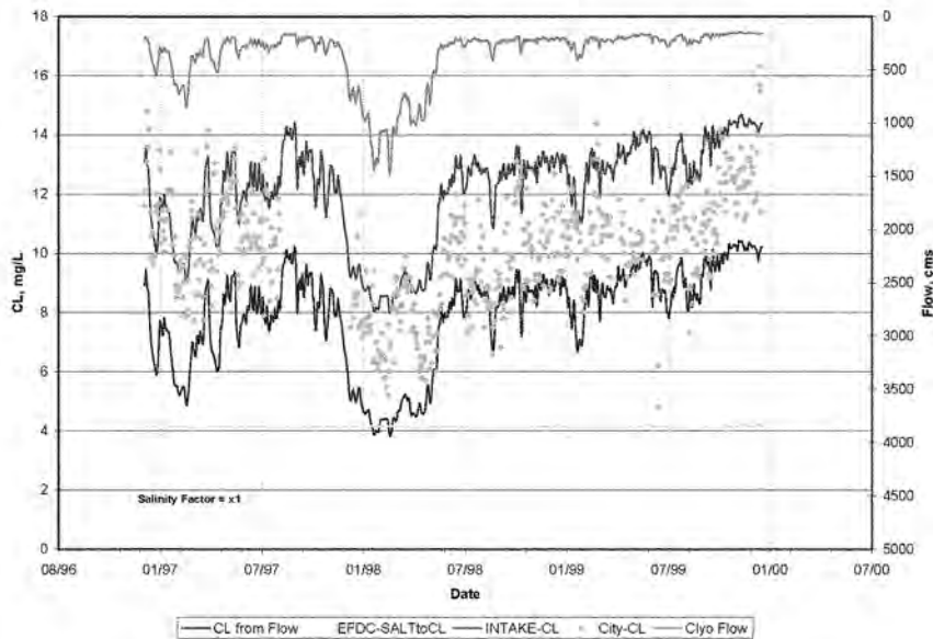
Figure 7-1 Predicted Chlorides at the Intake (1997 through 1999)
