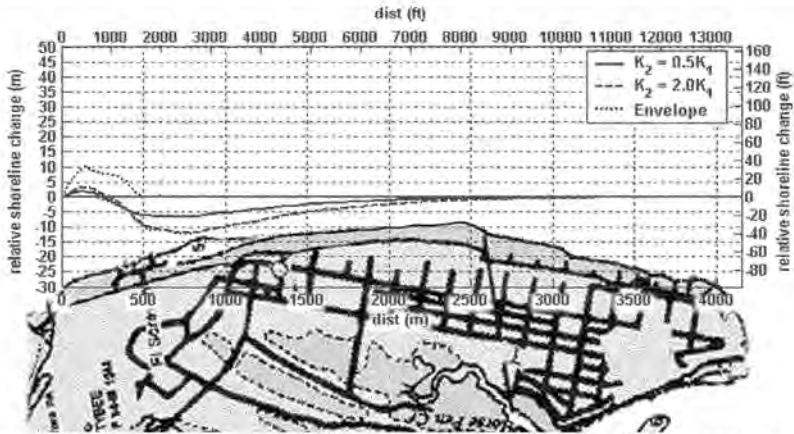
Figure 4-13. Relative change in shoreline between the Berm02 and base case. Solid line represents range in solutions within the uncertainty in the value of K_2 . Dotted line indicates range of relative shoreline change over the 20-year simulation.
