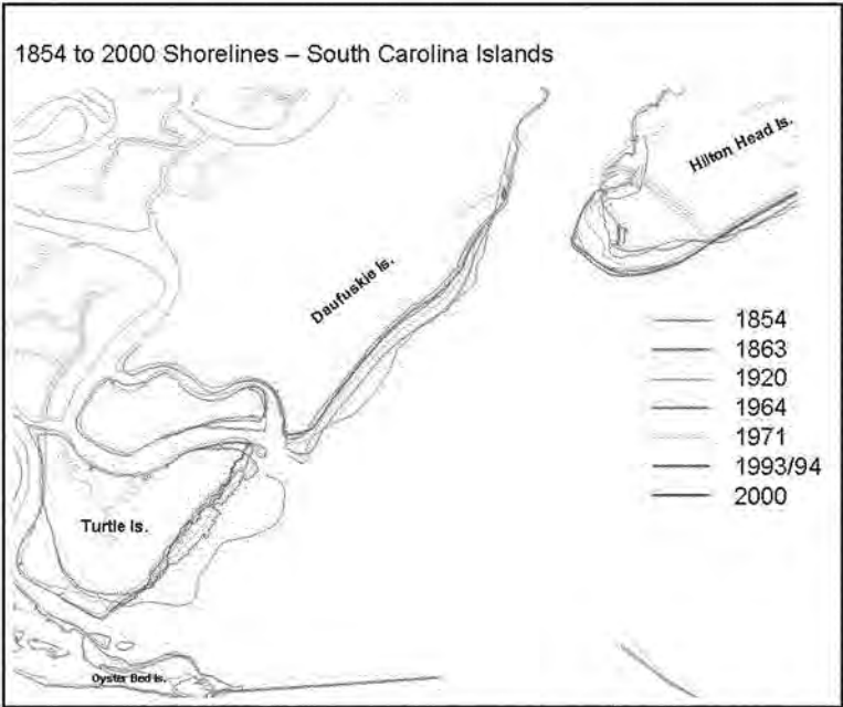
Figure 2-8. Historical shoreline positions of Turtle, Daufuskie and Hilton Head Islands, SC from digital shoreline used in study.
