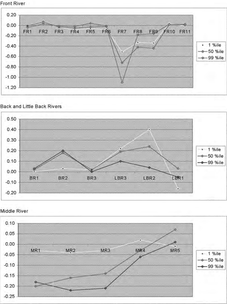
31. Figure A1.1. Changes in longitudinal profile of Dissolved Oxygen (mg/l) distribution along Critical cells of Savannah Estuary: 6 ft deepening
