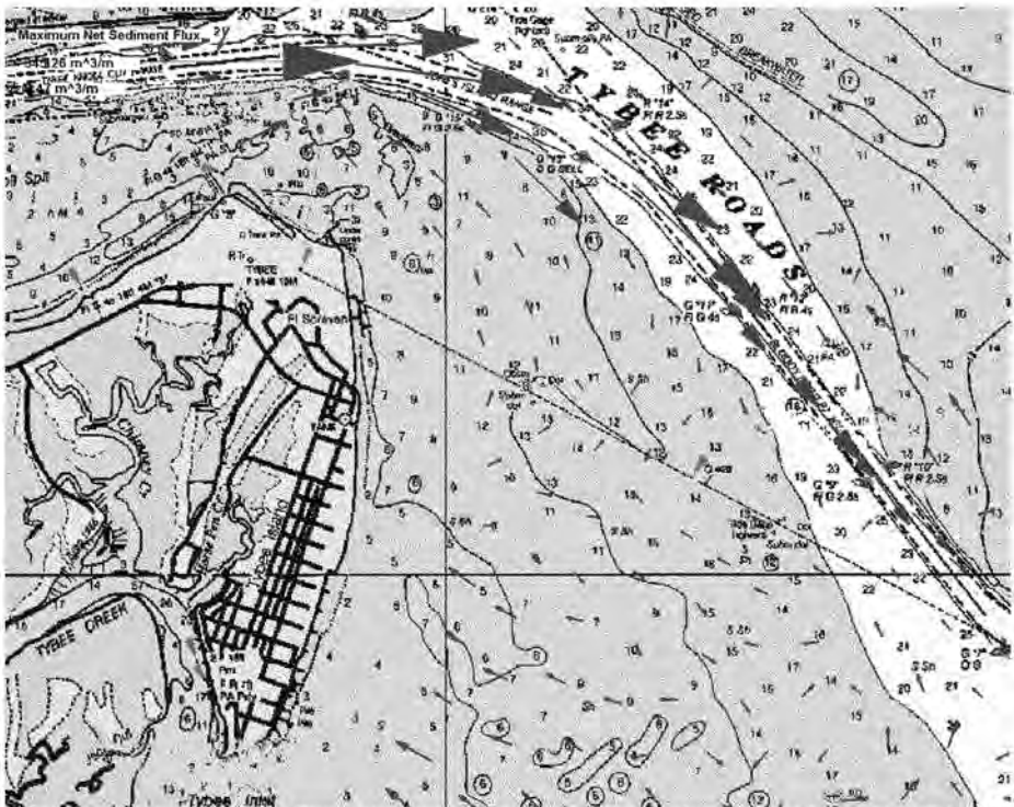
Figure 5-5. Cumulative sediment transport vectors for December 1999 existing conditions GTRAN simulation (Tybee Shelf).
