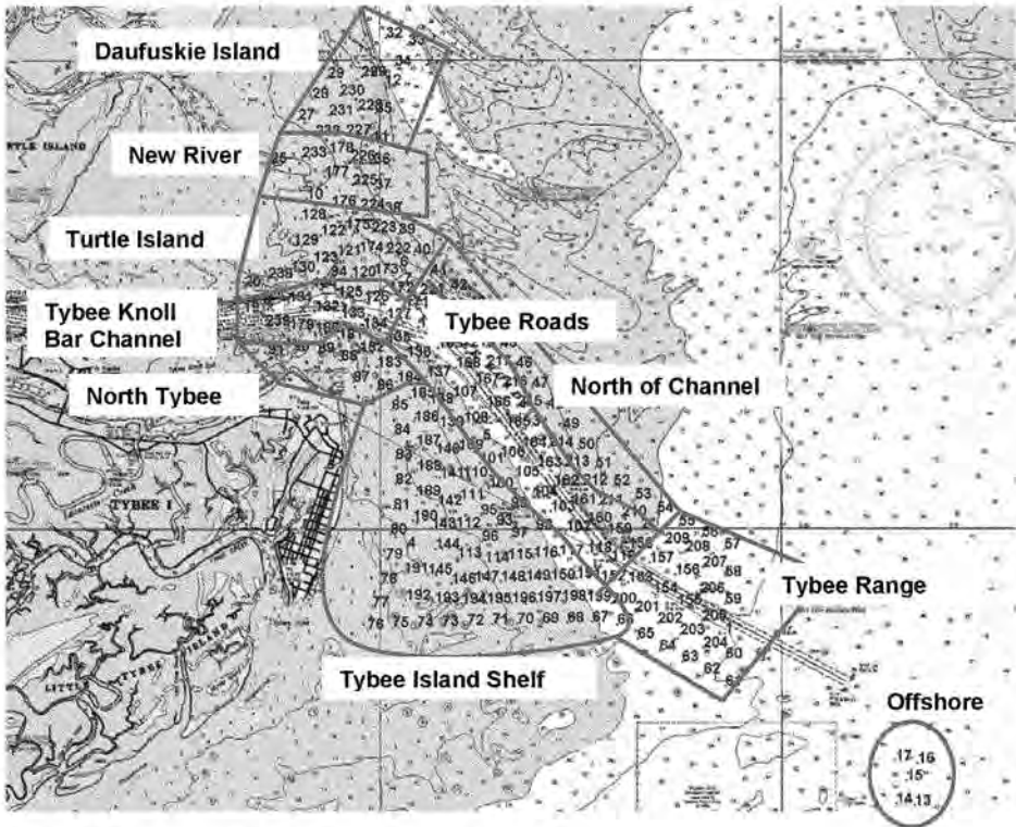
Figure 5-4. Summary of Regions Used in Table 5-1.
