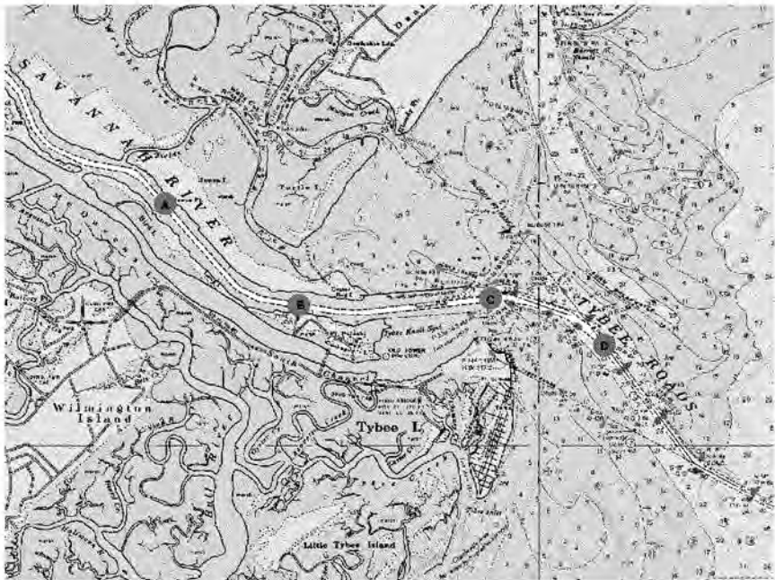
Figure 5-1: Locations of SSFATE simulations
