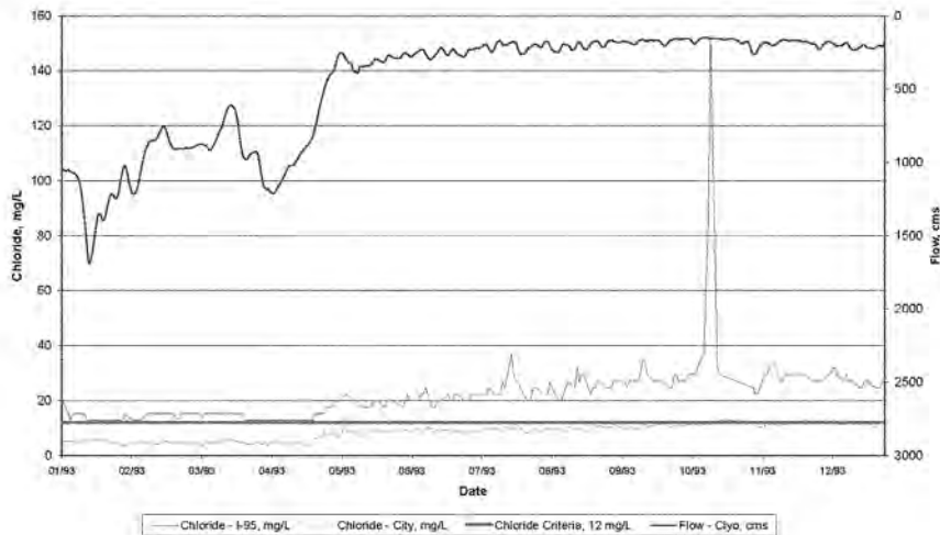
Figure 4-3 Chloride Values and Corresponding Flow Measurements for 1993
