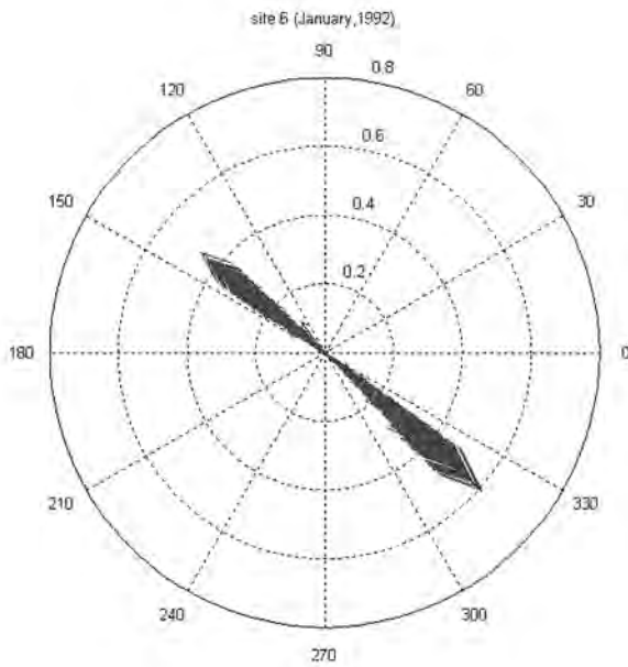
Figure 56. Current vectors at site 6 (current speed in m/s)
