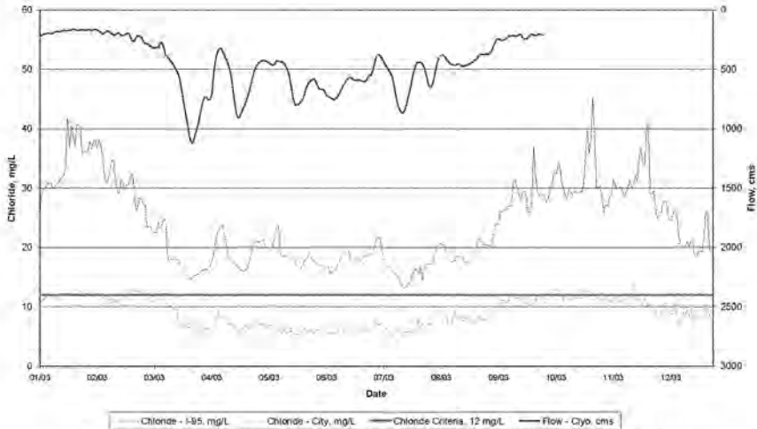
Figure 4-6 Chloride Values and Corresponding Flow Measurements for 2003
