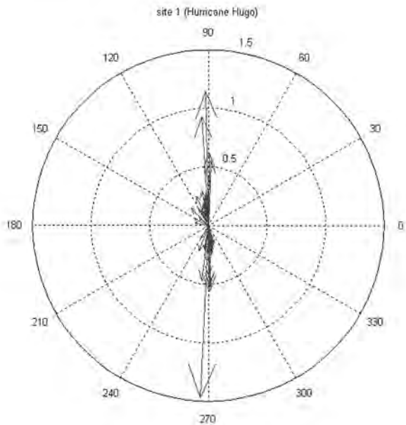
Figure 26. Current vectors at site 1 (current speed in m/s)
