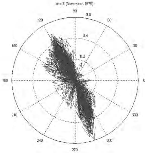
Figure 40. Current vectors at site 3 (current speed in m/s)
