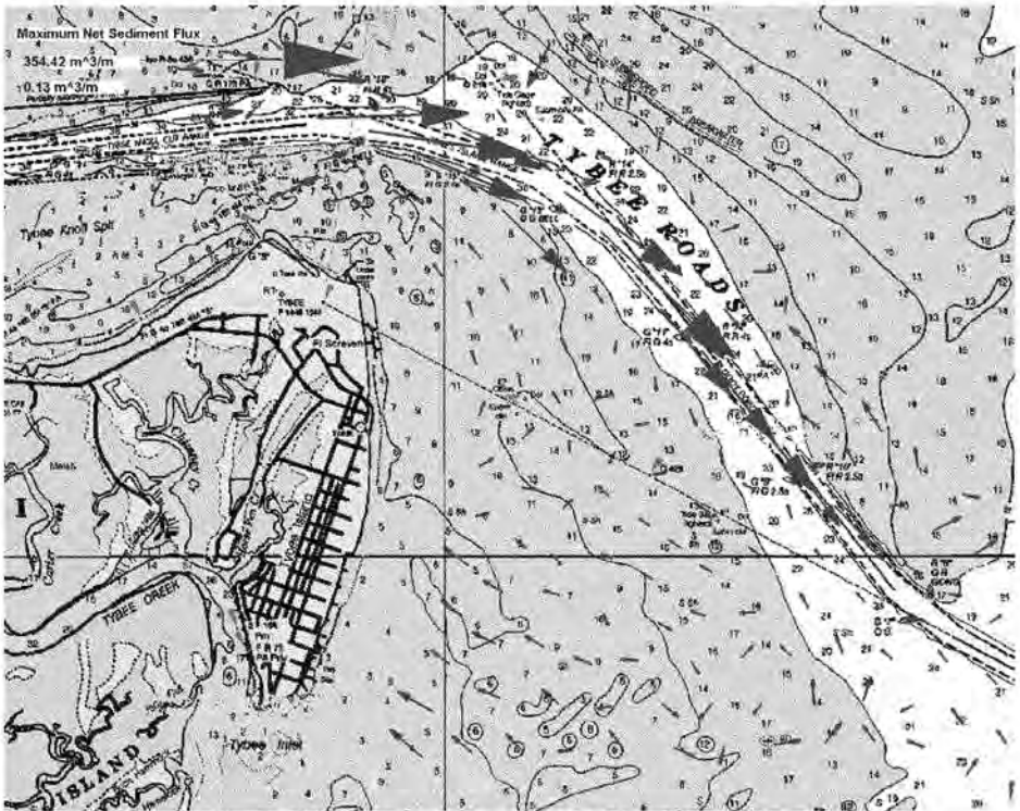
Figure 5-6. Cumulative sediment transport vectors for December 1999 deepened conditions GTRAN simulation (Tybee Shelf).
