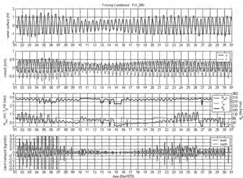
Figure 4-21d Time-series of water level, current, waves, and transport for November 1979 at Point 80 (Figure 4-20)
