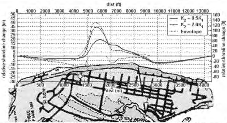
Figure 4-14. Relative change in shoreline between the Berm13 and base case. Solid line represents range in solutions within the uncertainty in the value of K_2 . Dotted line indicates range of relative shoreline change over the 20-year simulation.
