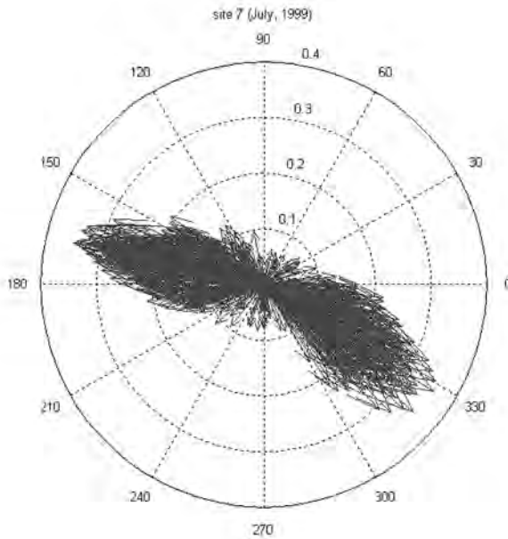
Figure 67. Current vectors at site 7 (current speed in m/s)
