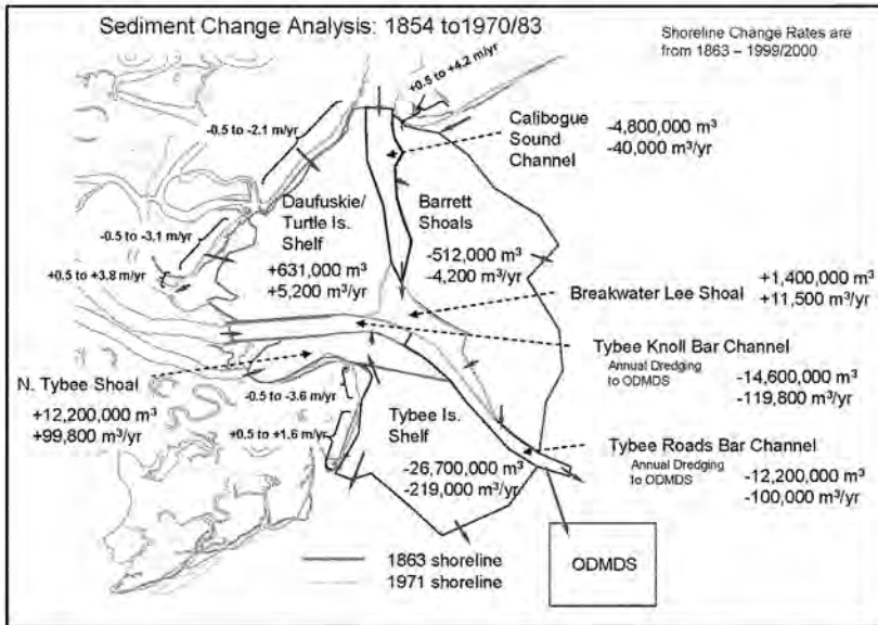
Figure 2-31. 1854 to 1970/83 Volume Change.
