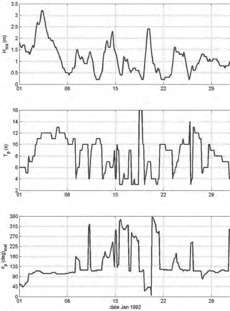
Figure 2-3. Offshore wave conditions for month of January 1992 at WIS sta 33. H_{m0} is energy-based wave height, T_p is the spectral peak period, \theta_p is the meteorological-convention wave direction (direction from which waves are approaching).
