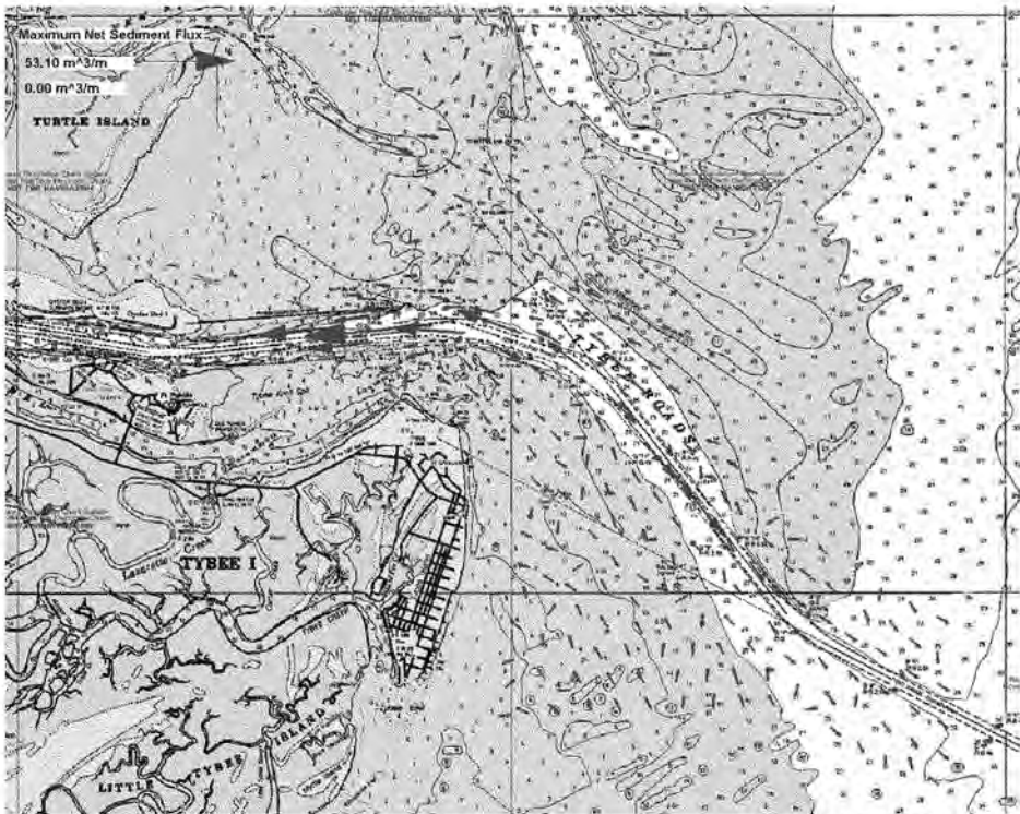
Figure 5D-4. Change in cumulative sediment transport vectors for July 1999 GTRAN simulation.
