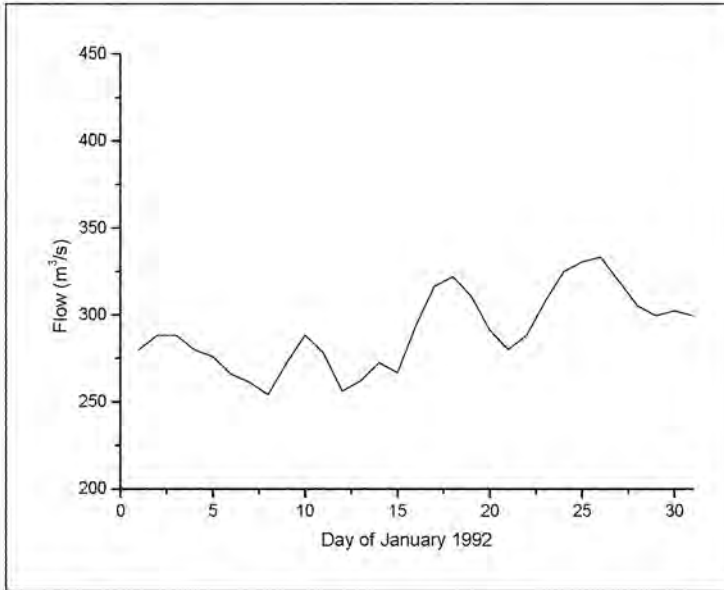
Figure 46. Daily discharge river flow for January 1992
