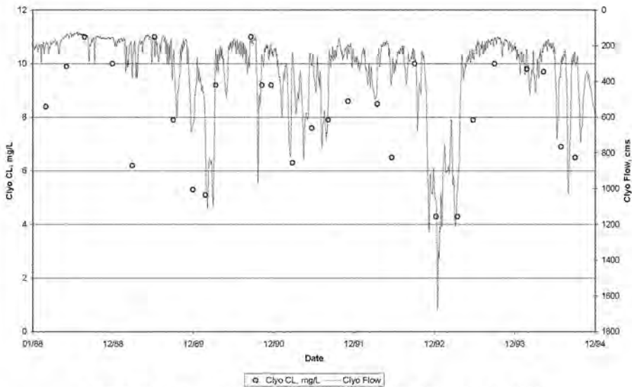
Figure 5-2 Flow and Chloride Observations at Clyo, GA (USGS 02198500)
