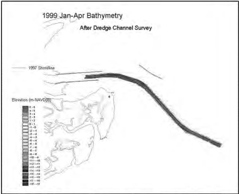
Figure 2-15. January/April 1999 Channel after dredge survey.
