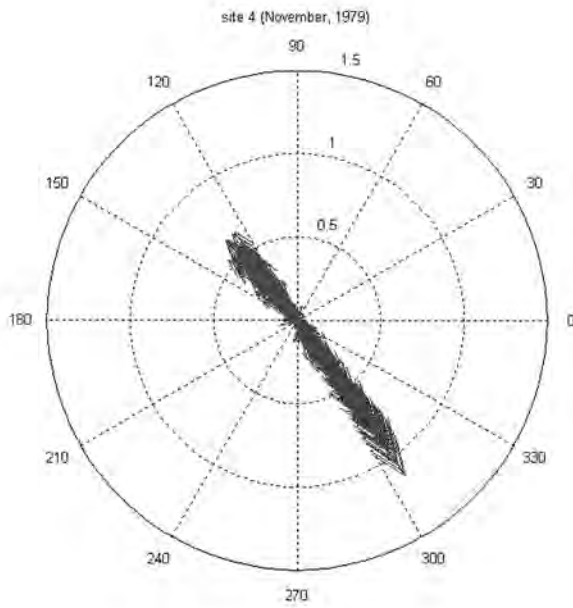
Figure 41. Current vectors at site 4 (current speed in m/s)
