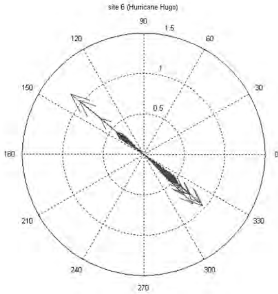
Figure 31. Current vectors at site 6 (current speed in m/s)
