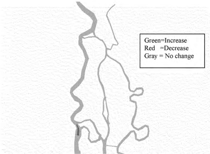
21. Figure A.1.2 Change in a suitable for Flounder Habitat area within the analyzed period August 1 - August 31, 1999 : 2 ft deepening
