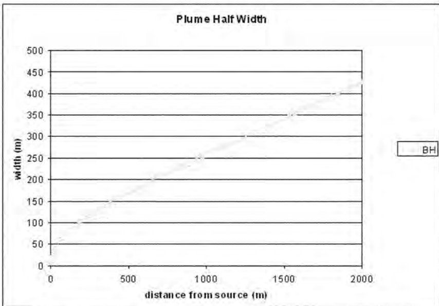
Figure 5-10a: Plume gaussian half width, simulation riv10d
