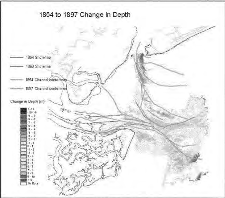
Figure 2-18. 1854 to 1897 change in bathymetry.
