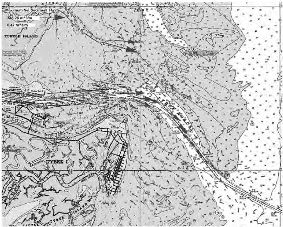
Figure 5B-9. Cumulative sediment transport vectors for December 1999 existing conditions GTRAN simulation.
