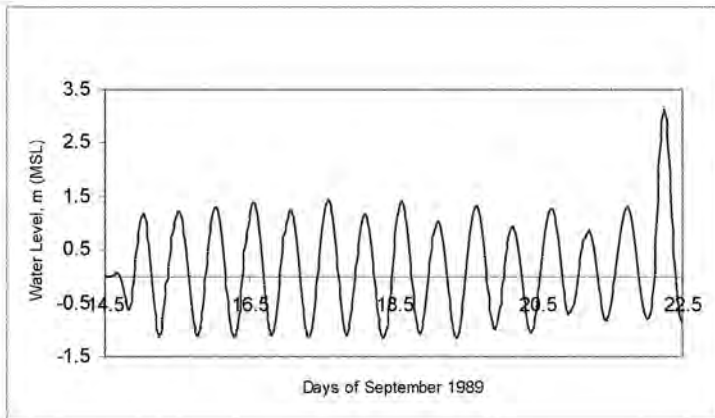
Figure 24. Calculated water level at Ft Pulaski
