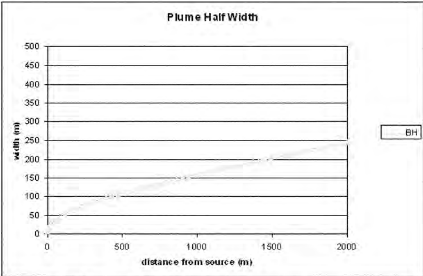
Figure 5-12a: Plume gaussian half-width, simulation tyb25cms
