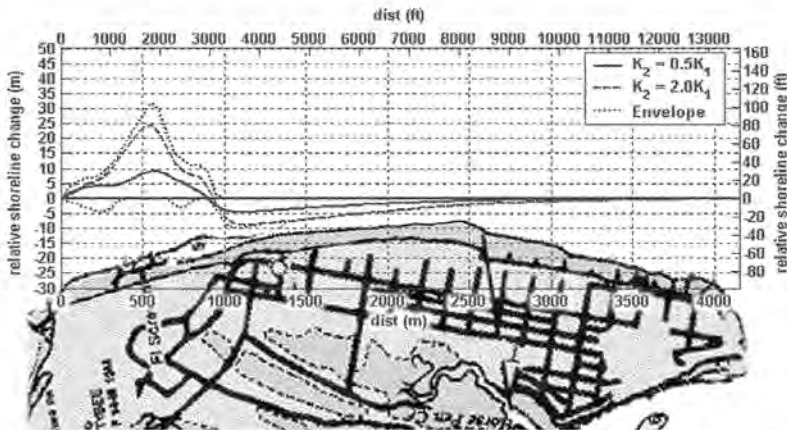
Figure 4-12. Relative change in shoreline between the Berm01 and base case. Solid line represents range in solutions within the uncertainty in the value of K_2 . Dotted line indicates range of relative shoreline change over the 20-year simulation.
