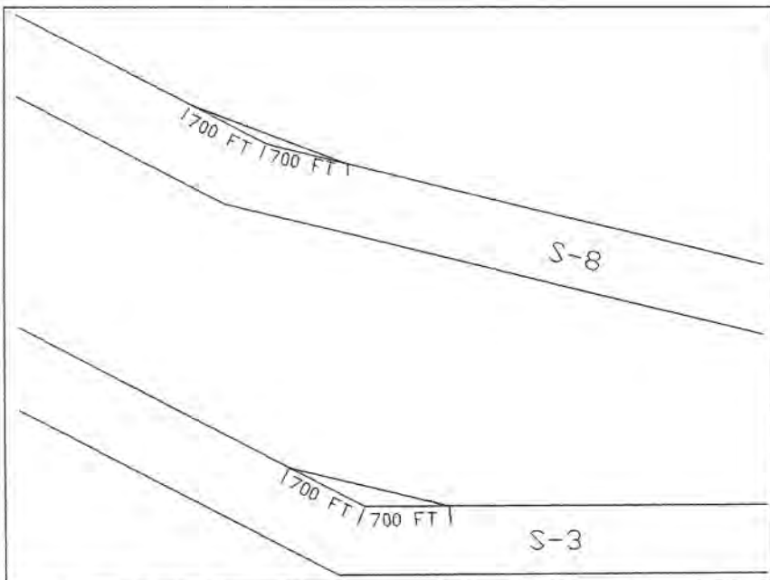
Figure 2. Bend Wideners
