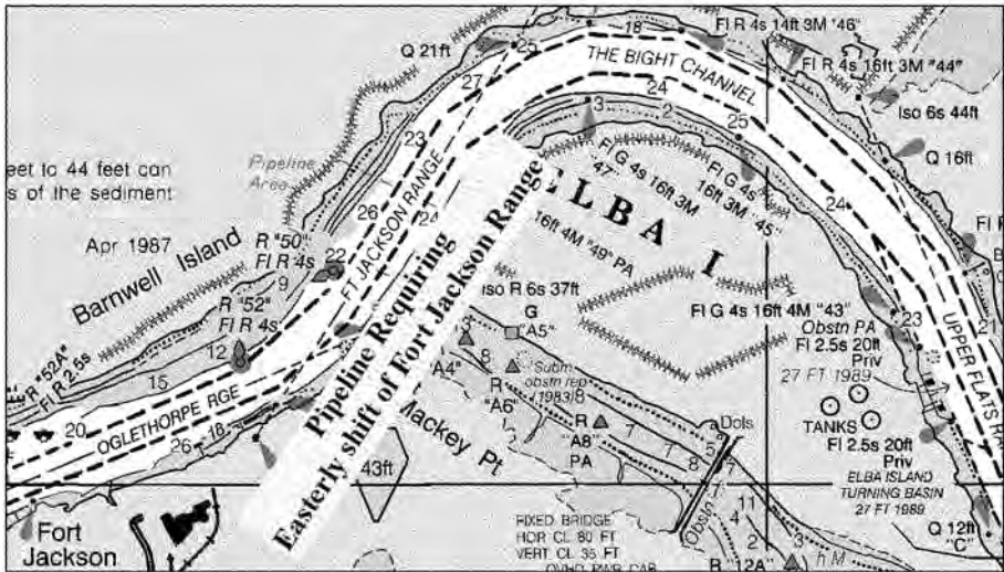
Figure 6. Pipeline requires shifting channel to east
