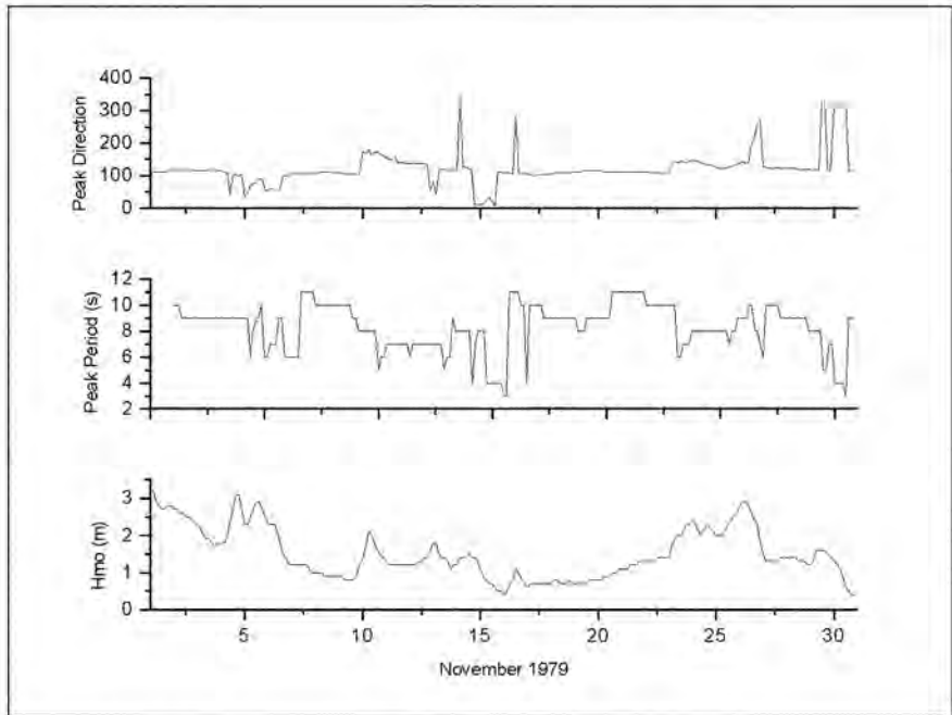
Figure 33. Wave height, period and direction during November 1979
