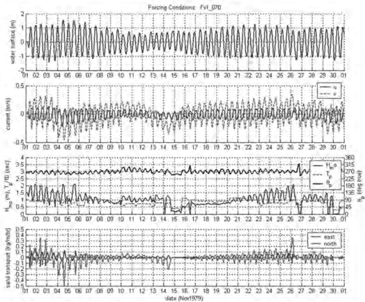
Figure 4-21b Time-series of water level, current, waves, and transport for November 1979 at Point 70 (Figure 4-20)
