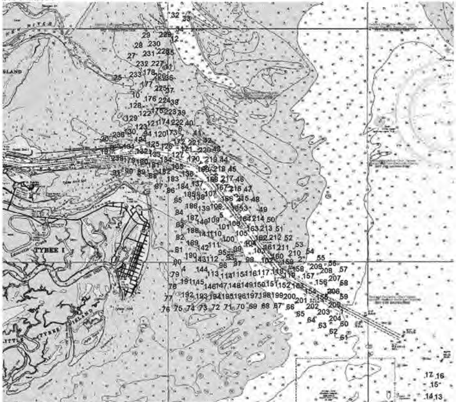
Figure 5-3. GTRAN calculation locations.
