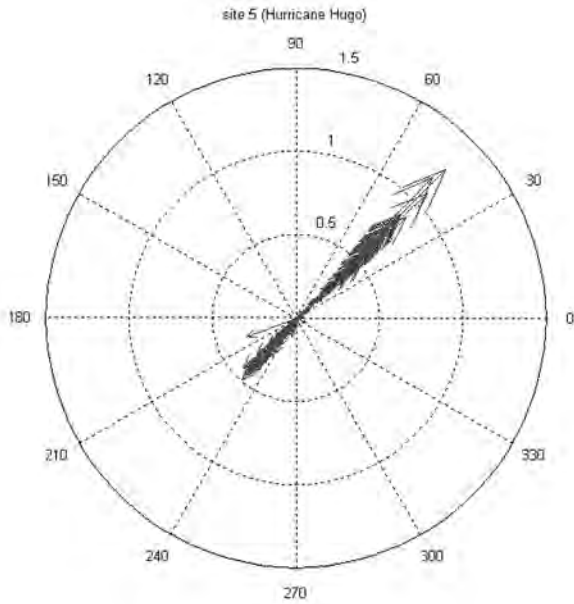
Figure 30. Current vectors at site 5 (current speed in m/s)
