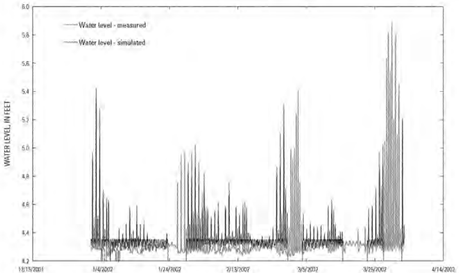
Figure 28. Measured and simulated hourly water levels at Site B2 on the Little Back River for the period January 1 to March 31, 2002. Breaks in the prediction time series are caused by incomplete time series for one or more of the model inputs.
