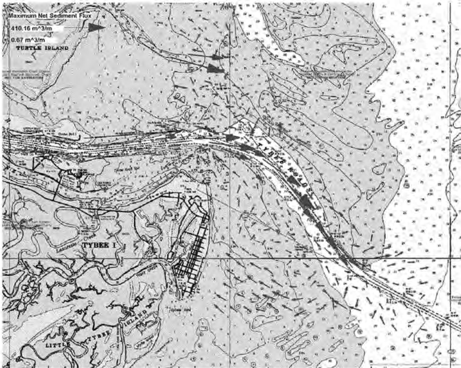
Figure 5B-2. Cumulative sediment transport vectors for November 1979 deepened conditions GTRAN simulation.
