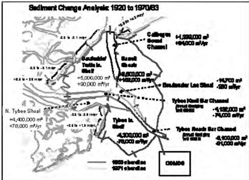
Figure 2-32. 1920 to 1970/83 Volume Changes
