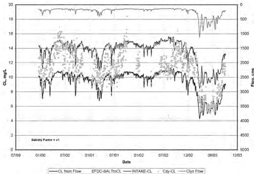
Figure 7-2 Predicted Chlorides at the Intake (2000 through 2003)
