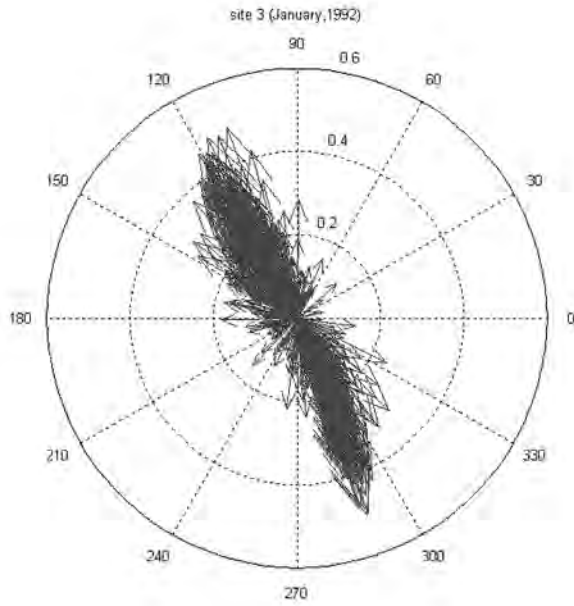
Figure 53. Current vectors at site 3 (current speed in m/s)
