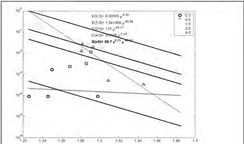
Figure A-5c: Erosion data for Site 52S
