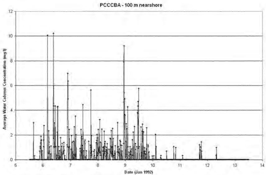
Figure 5-5c: SSFATE simulation PCCCAA, depth-averaged time-series concentration 100m toward shore from the source
