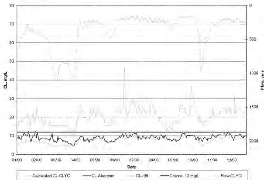
Figure 5-4 Calculated Chloride Time Series at Clio - 1990
