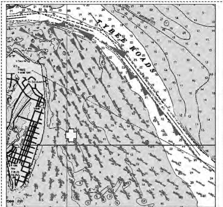
Figure 6-1. Sediment transport pattern at the Savannah River Entrance
