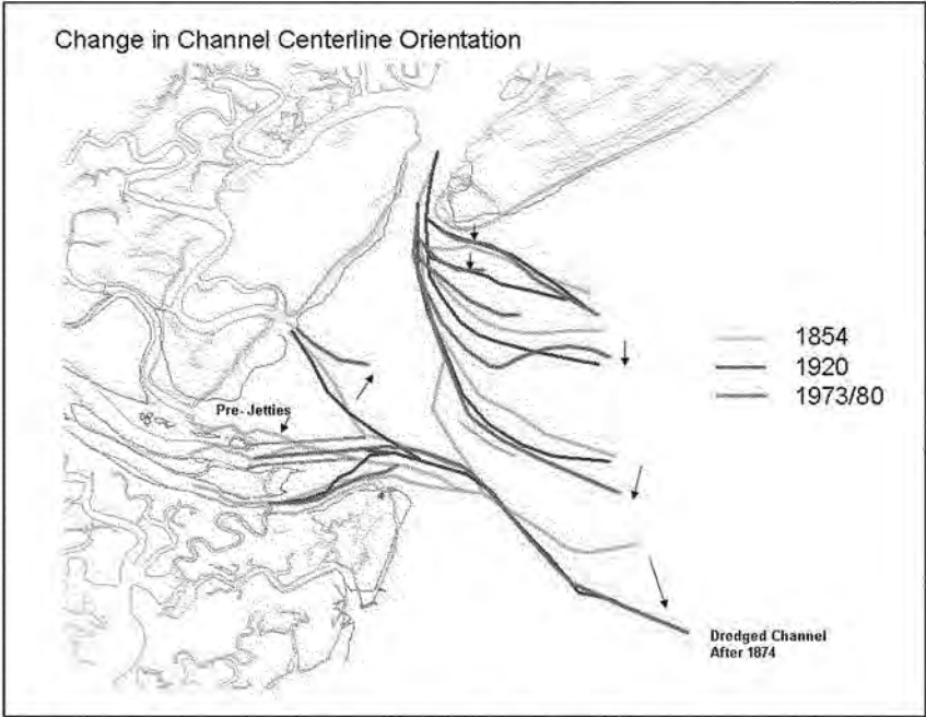
Figure 2-28. Change in channel centerline orientation.
