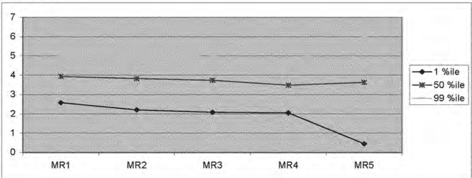
8. Figure A.1. Longitudinal profile of Dissolved Oxygen (mg/l) distribution along Critical cells of Savannah Estuary: Existing bathymetry
