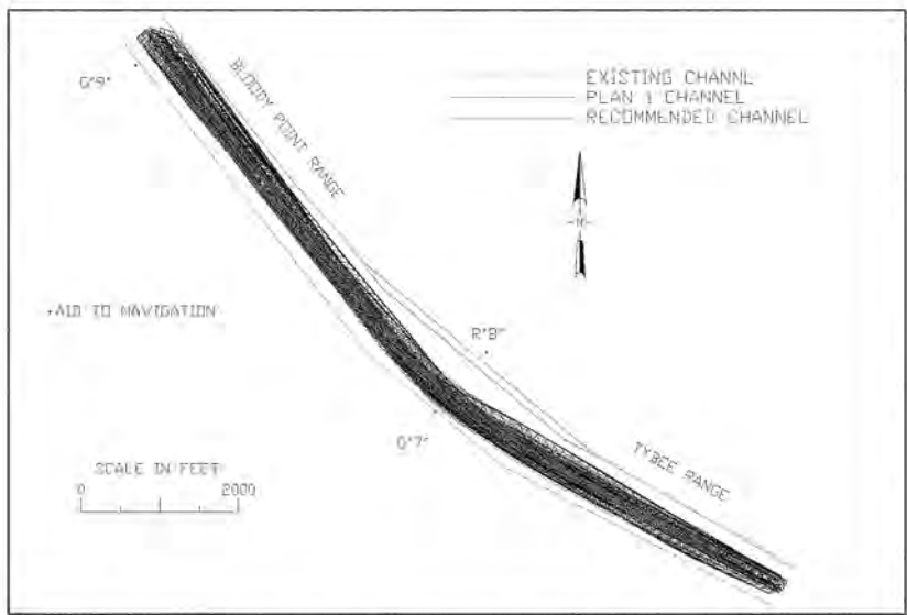
Figure 21. 43-ft draft Susan Maersk at turn between Tybee and Bloody Point Ranges
