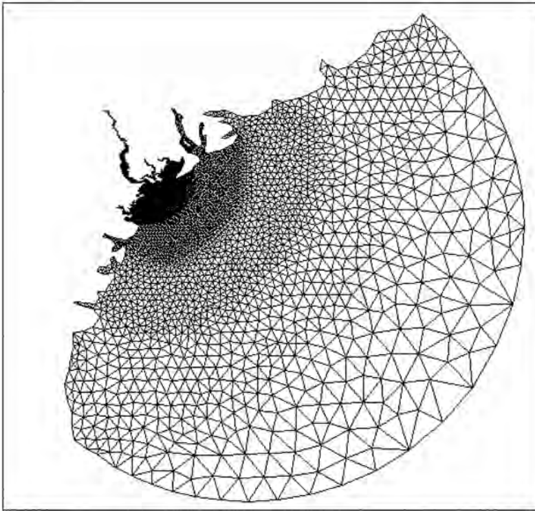
Figure 3. Regional ADCIRC grid
