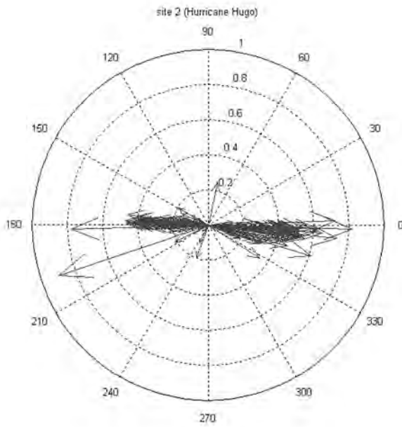
Figure 27. Current vectors at site 2 (current speed in m/s)
