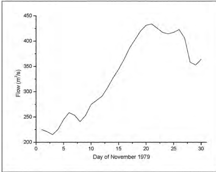
Figure 33. Daily discharge river flow for November 1979
