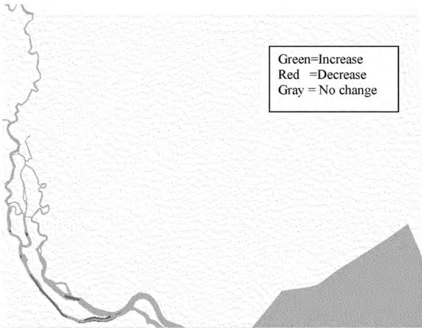
19. Figure D.1.2. Change in a suitable for Bass Eggs Habitat area within the analyzed period April 1 - April 30, 1999 : 6 ft deepening
