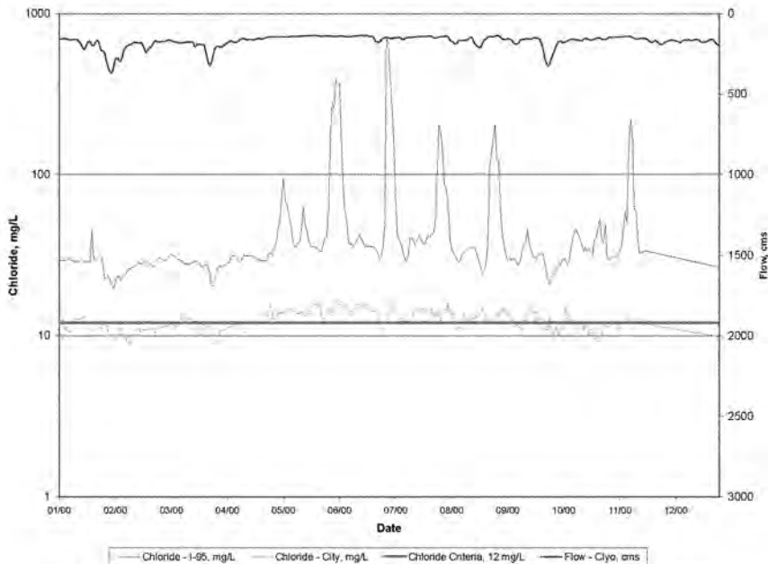
Figure 4-5 Chloride Values and Corresponding Flow Measurements for 2000
