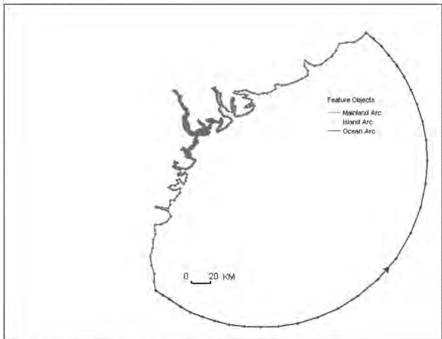
Figure 2. ADCIRC domain and its boundaries
