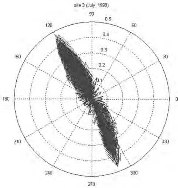
Figure 63. Current vectors at site 3 (current speed in m/s)
