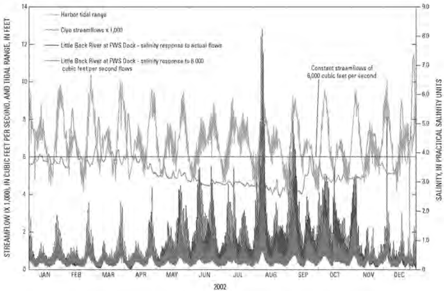
Figure 45. Salinity response at Little Back River at U.S. Fish and Wildlife Service Dock (station 021989791) for calendar year 2002 streamflows and constant 6,000 ft 3 /s streamflows. Tidal range for Savannah River at Fort Pulaski (station 02198980) also are shown.
