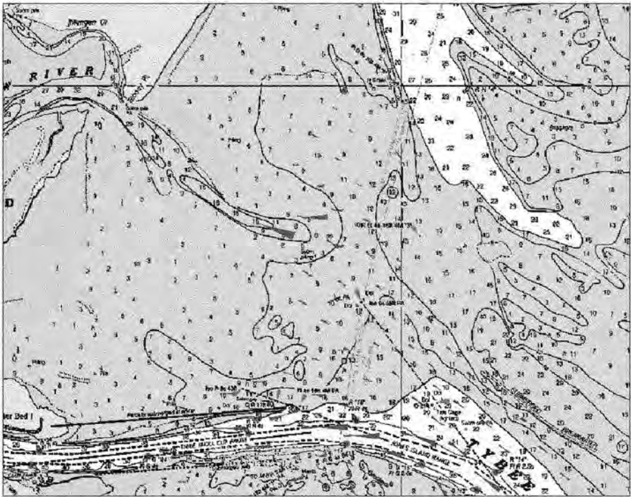
Jul 1999 Net Sediment Transport After Deepening
