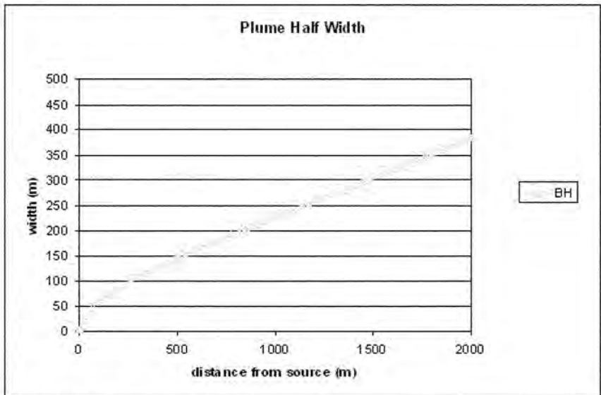
Figure 5-10c: Plume gaussian half width, simulation riv10j
