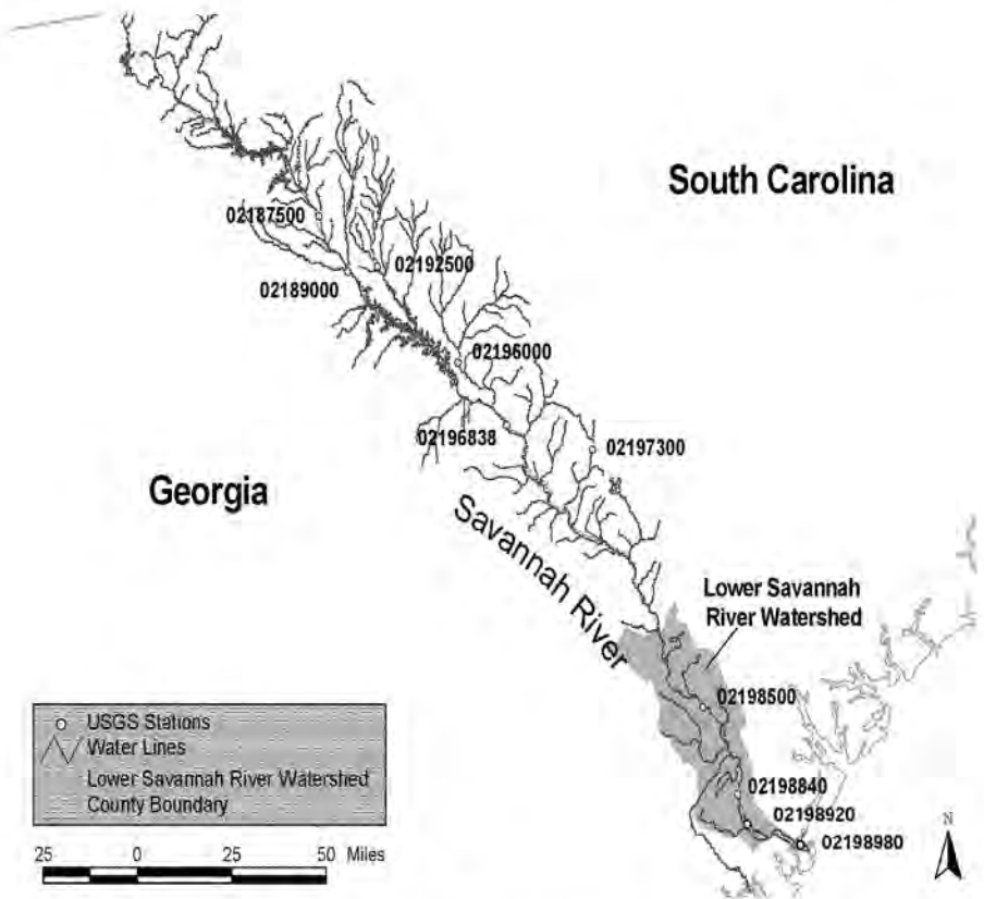
Figure 6-1 USGS Station Locations Within and Upstream of the Lower Savannah River Watershed
