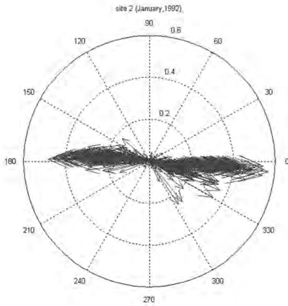
Figure 52. Current vectors at site 2 (current speed in m/s)
