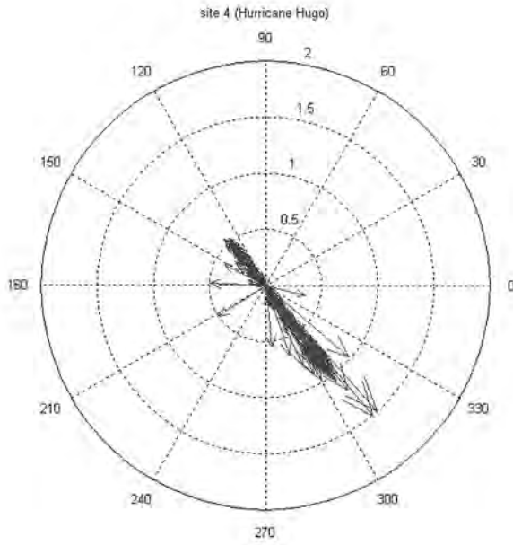
Figure 29. Current vectors at site 4 (current speed in m/s).
