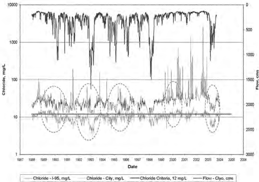
Figure 4-1 Chloride Values and Corresponding Flow Measurements
