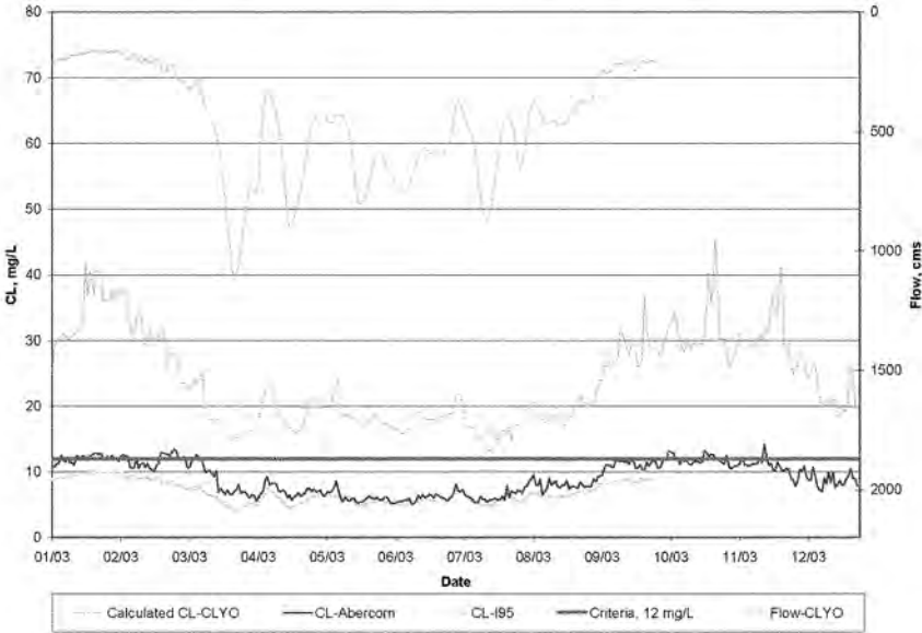
Figure 5-8 Calculated Chloride Time Series at Clio - 2003
