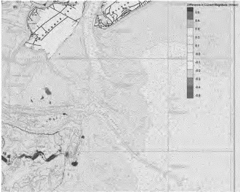
Figure 3-17. Difference in maximum current magnitudes for January 1992 (deepened channel minus existing bathymetry).
