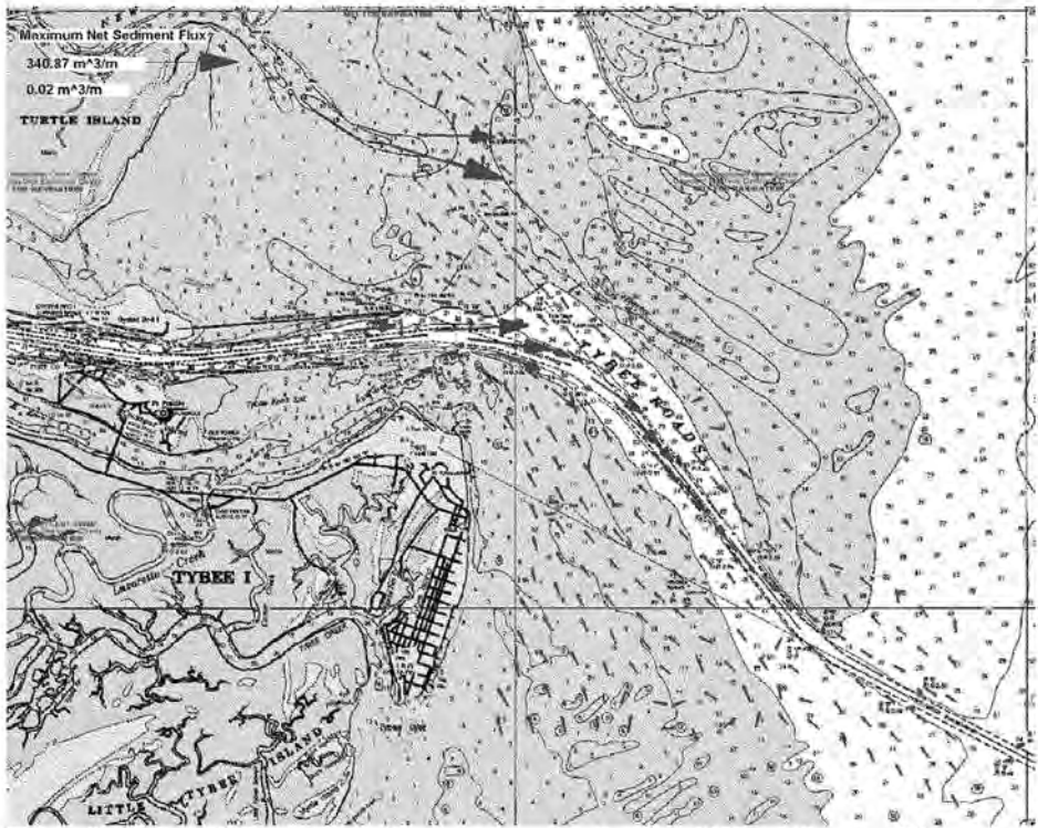
Figure 5B-7. Cumulative sediment transport vectors for July 1999 existing conditions GTRAN simulation.
