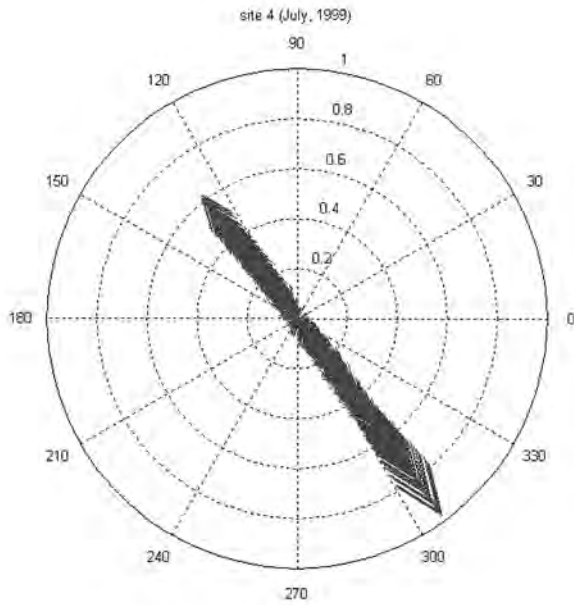
Figure 64. Current vectors at site 4 (current speed in m/s)
