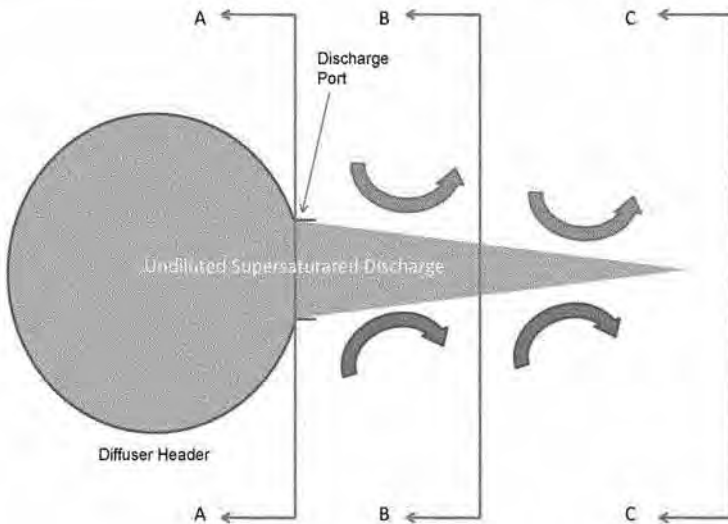
Fig. 4 Schematic of Mixing in Diffuser Jet
