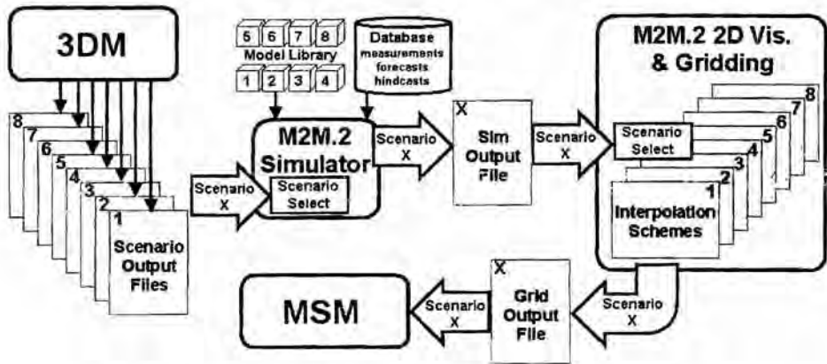
Figure 3. Schematic of data and workflow through the M2M.2.
