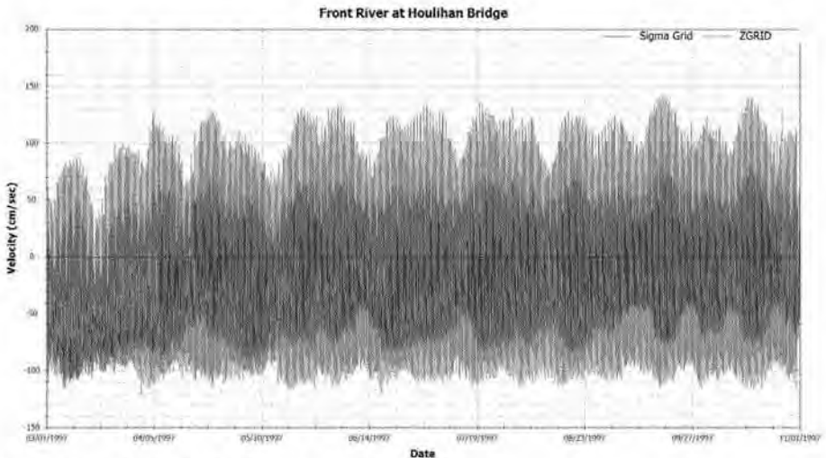
Figure 4-4 Front River Velocity Comparison
