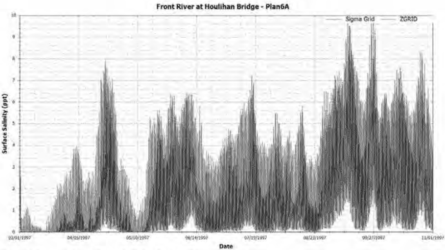
Figure 4-7 Front River Salinity Comparisons – Plan6A
