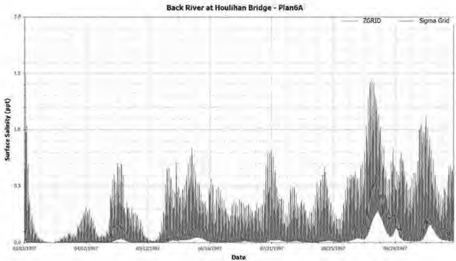
Figure 4-9 Back River Salinity Comparisons – Plan6A
