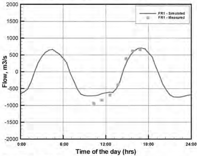
Figure 18 – Front River (FR1) Transect on October 6, 1999
