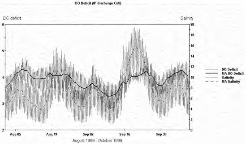
Figure 9 – DO deficit versus salinity at IP discharge (MA = Moving Average)
