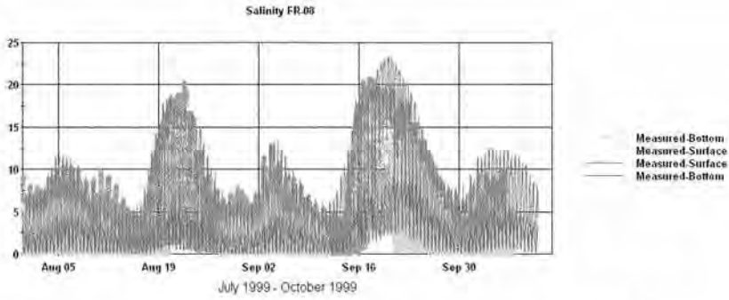
Figure 11 – 1999 Salinity on the Front River near Middle River Confluence (FR-08)
