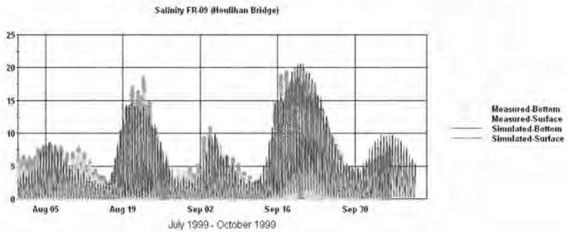
Figure 12 – 1999 Salinity on the Front River at Houlihan Bridge (FR-09)
