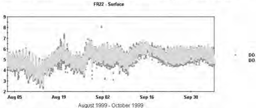
Figure 22 – 1999 Dissolved Oxygen on Front River in Kings Island TB (FR-22) Surface
