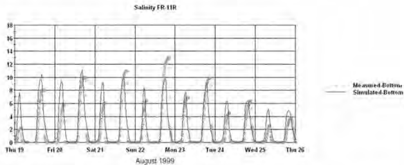
Figure 14 – August 1999 Salinity on the Front River Upstream of Houlihan Bridge (FR-11R)
