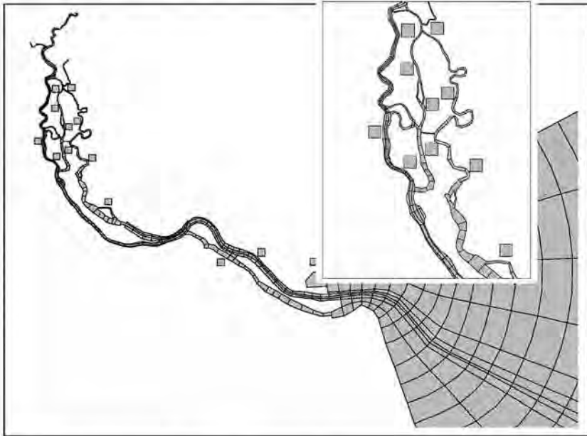
Figure 2-2 Savannah Harbor Z-Grid Model (marsh cells shown for representation)
