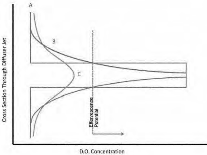
Fig 5. D.O. Profile in Diffuser Jet
