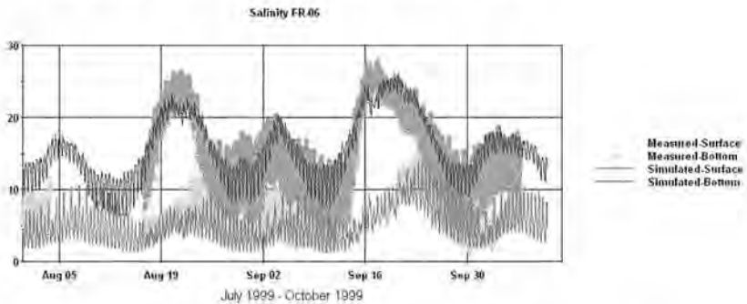
Figure 10 – 1999 Salinity on the Front River Upstream of Talmadge Bridge (FR-06)
