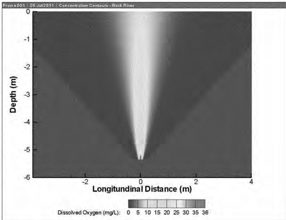
Figure 18 Mixing Zone results from Visual Plumes
