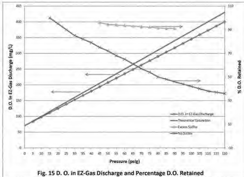
Fig. 15 D.O. in EZ-Gas Discharge and Percentage D.O. Retained
