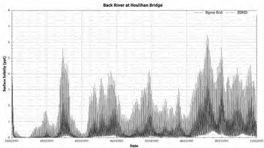
Figure 4-3 Back River Salinity Comparisons
