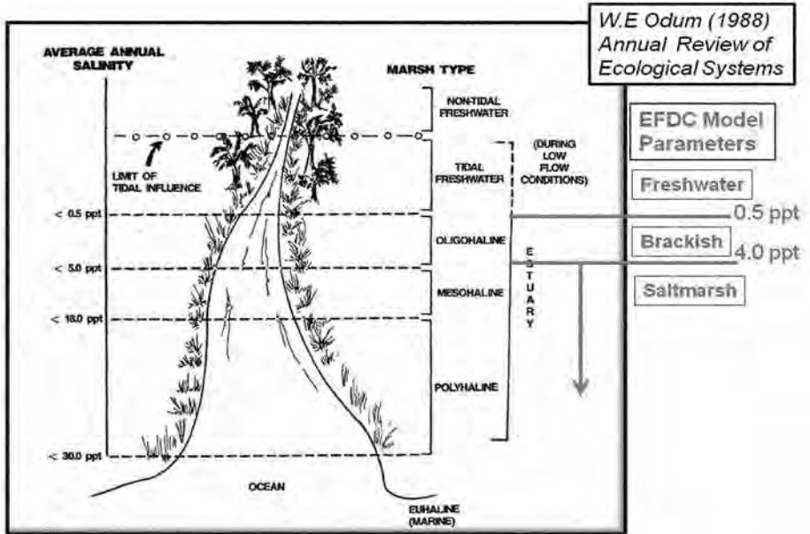
Figure 51. Tidal Estuarine System with EFDC Model Parameters
