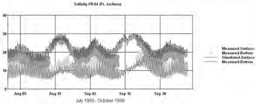
Figure 9 – 1999 Salinity on the Front River at Fort Jackson (FR-04)
