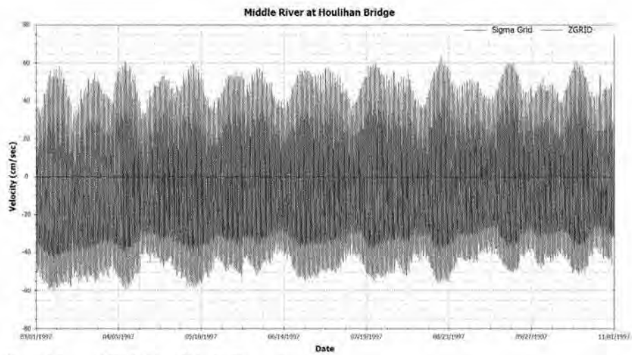
Figure 4-5 Middle River Velocity Comparison
