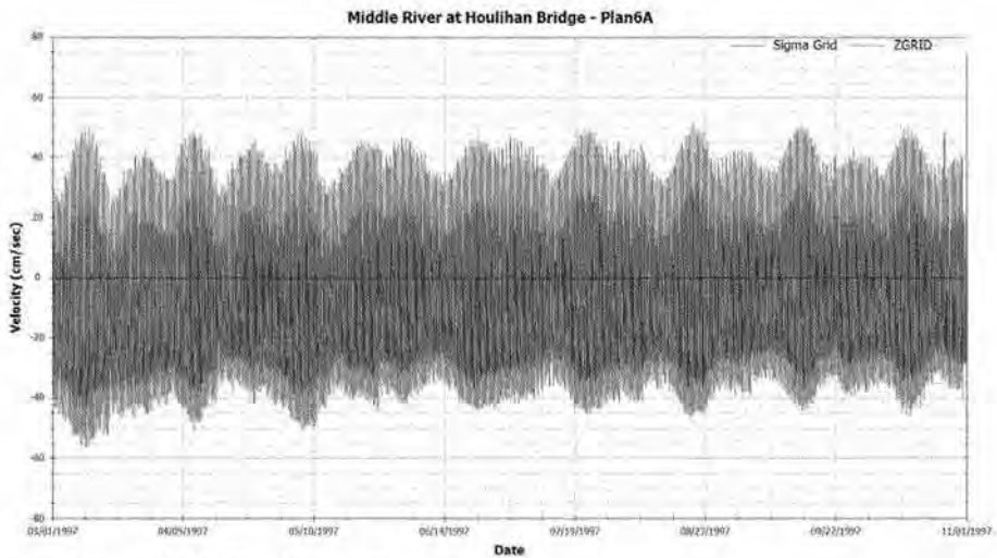
Figure 4-11 Middle River Velocity Comparison
