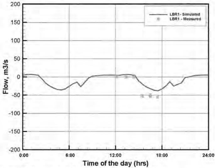
Figure 20 – Little Back River (LBR1) Transect on October 6, 1999
