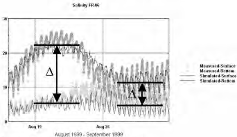
Figure 8 – Salinity Stratification at FR-06 on the Front River
