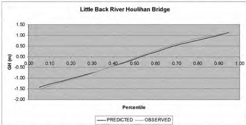
Figure 2-3 Percentile Comparison of Predicted and Measured Gage Heights
