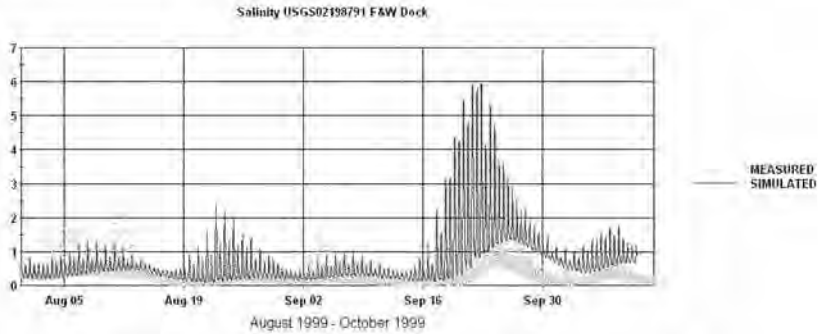
Figure 16 – 1999 Salinity on the Little Back River at F&W Dock (USGS 02198791)
