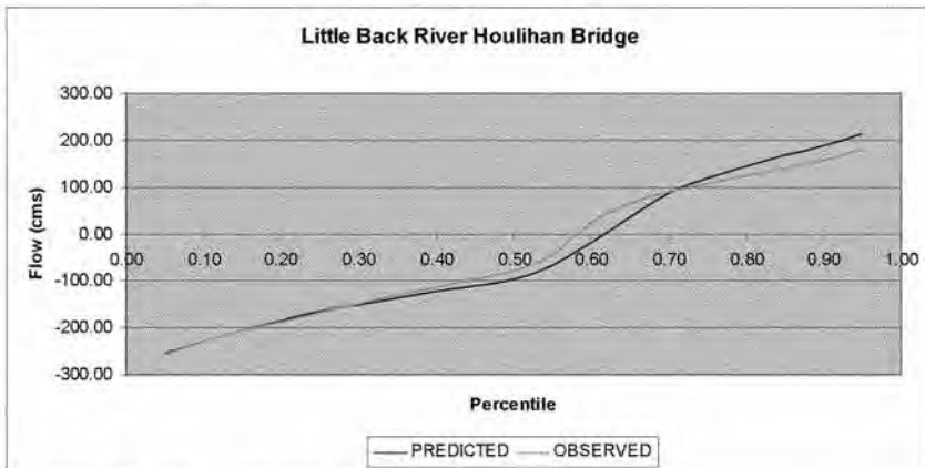
Figure 2-4 Percentile Comparison of Predicted and Measured Flows
