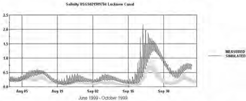
Figure 17 – 1999 Salinity on the Little Back River at Lucknow Canal (USGS 021989784)
