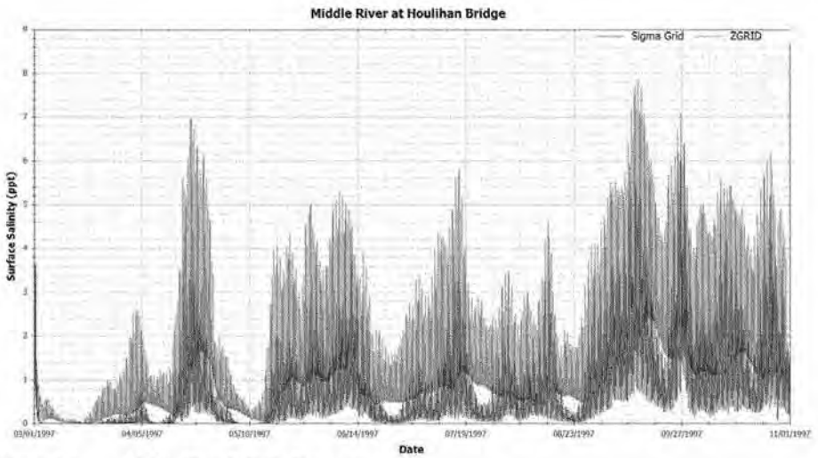
Figure 4-2 Middle River Salinity Comparisons
