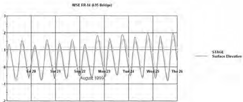
Figure 5 - August 1999 Water Surface Elevation at I-95 Bridge (FR-14)
