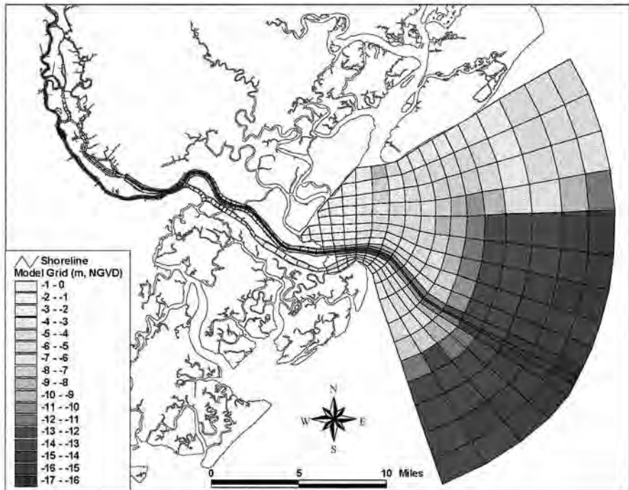
Figure 2-1 EFDC Sigma Grid
