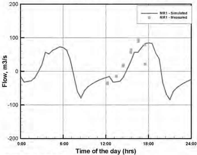
Figure 19 – Middle River (MR1) Transect on October 6, 1999
