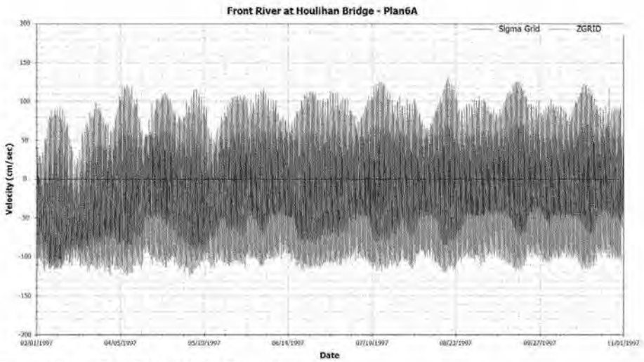
Figure 4-10 Front River Velocity Comparison
