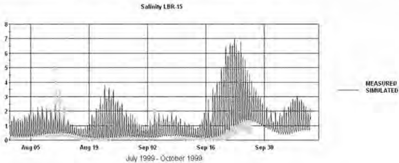
Figure 15 – 1999 Salinity on the Little Back River at Houlihan Bridge (LBR-15)
