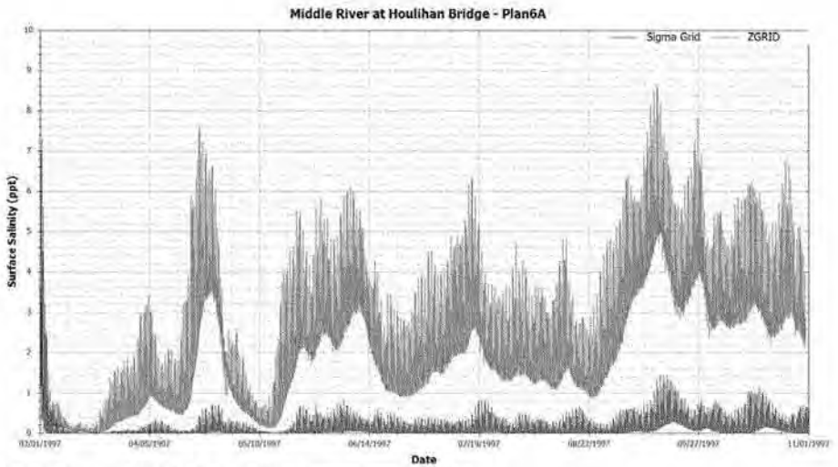
Figure 4-8 Middle River Salinity Comparisons – Plan6A
