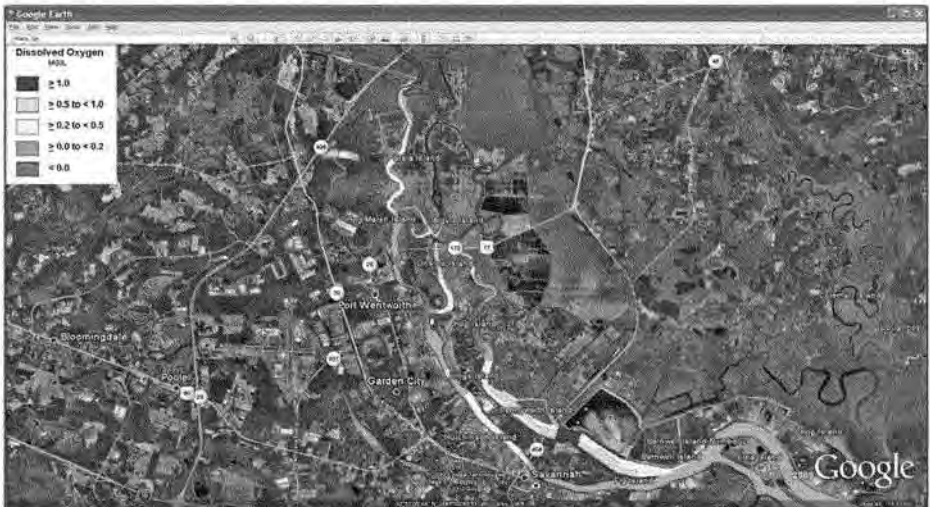
Figure B-4 Delta D.O. (50 th percentile): Mitigation plan 6a-3ft and D.O. discharge
