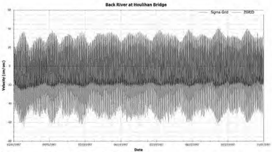
Figure 4-6 Back River Velocity Comparison
