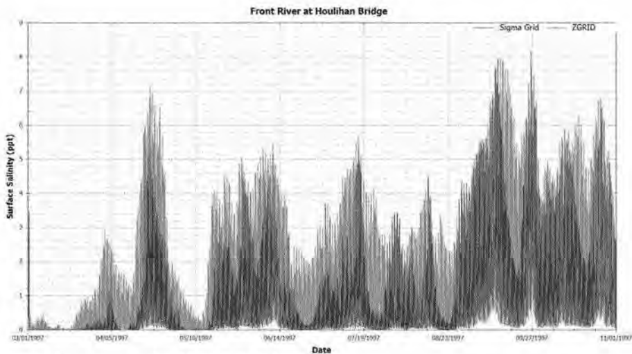
Figure 4-1 Front River Salinity Comparisons
