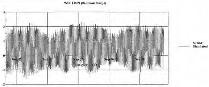
Figure 2 – 1999 Water Surface Elevation at Houlihan Bridge (FR-09)
