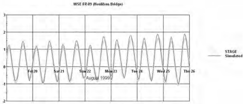
Figure 3 – August 1999 Water Surface Elevation at Houlihan Bridge (FR-09)
