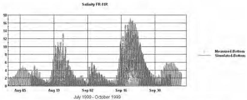
Figure 13 – 1999 Salinity on the Front River Upstream of Houlihan Bridge (FR-11R)
