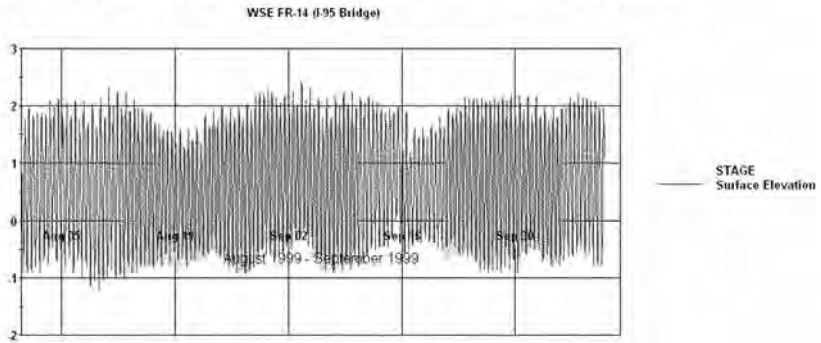
Figure 4 – 1999 Water Surface Elevation at I-95 Bridge (FR-14)
