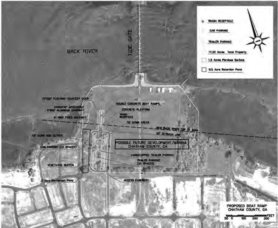
Figure 4.2.1-2 Proposed Hutchinson Island Boat Ramp
