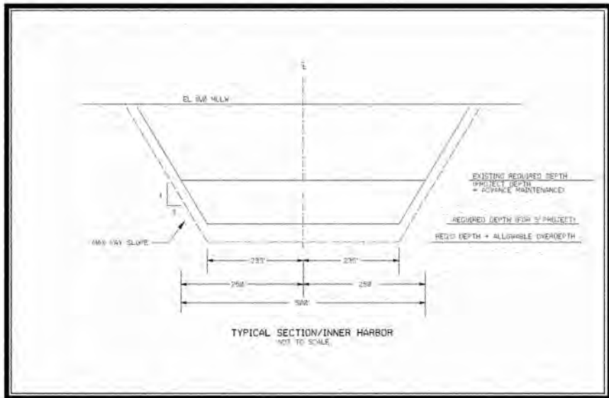
Figure 8-1: Typical Channel Cross Section
