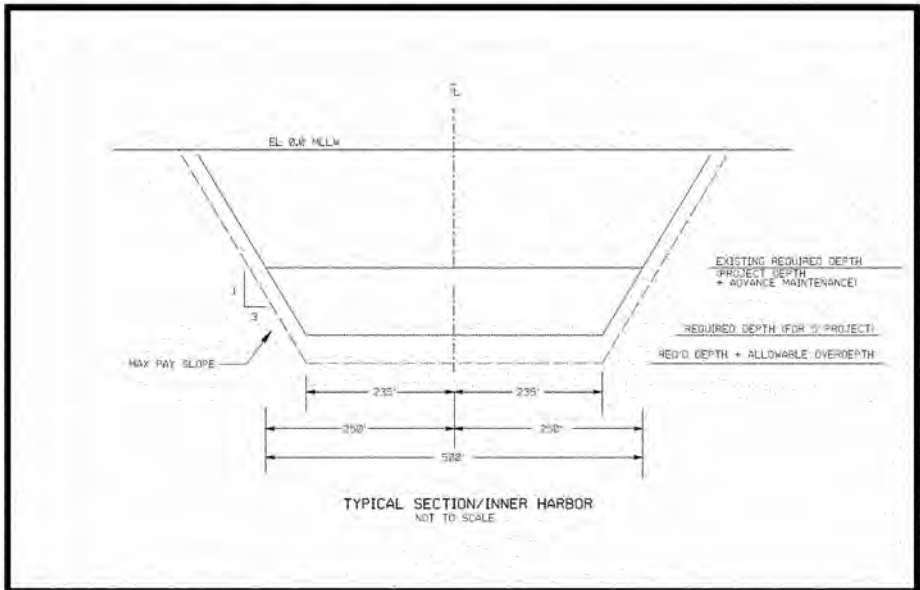
Figure 1-3: Typical Dredging Section – Inner Harbor
