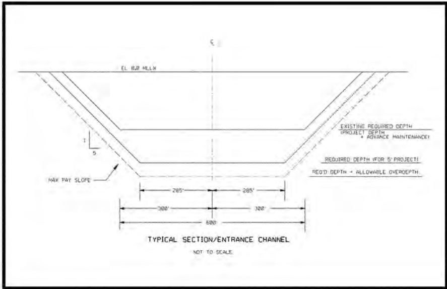
Figure 1-4: Typical Dredging Section – Entrance Channel
