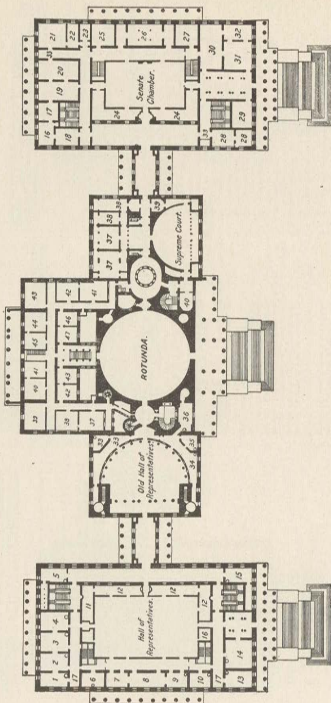
PRINCIPAL FLOOR.
