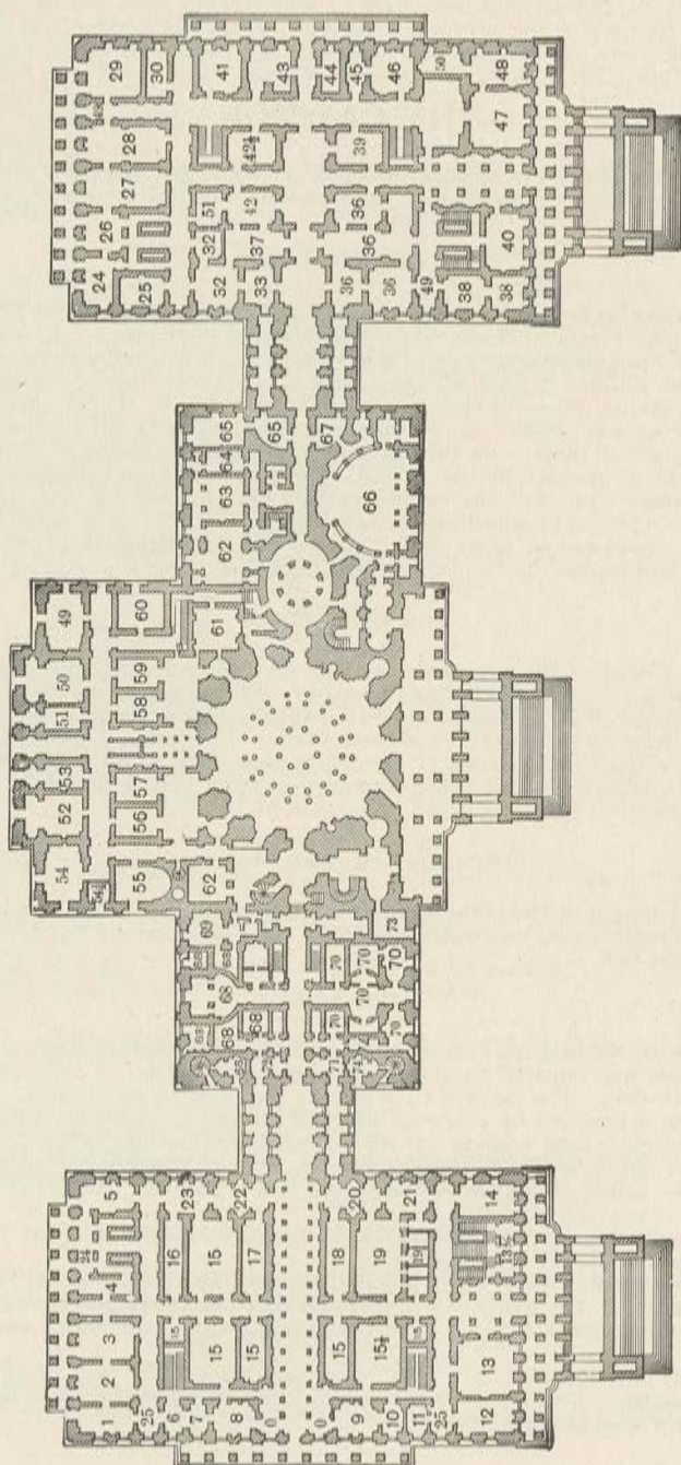
BASEMENT FLOOR.
